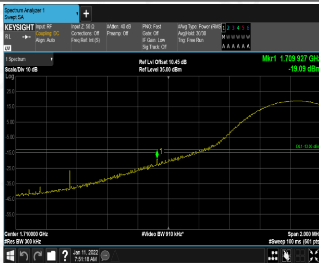
Band4-15MHz-QPSK-20025-1RB#74
