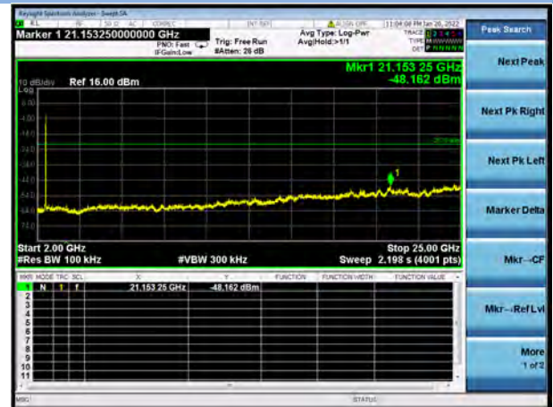
802.11b CHANNEL 13, SPURIOUS 2 GHz ~ 25 GHz
