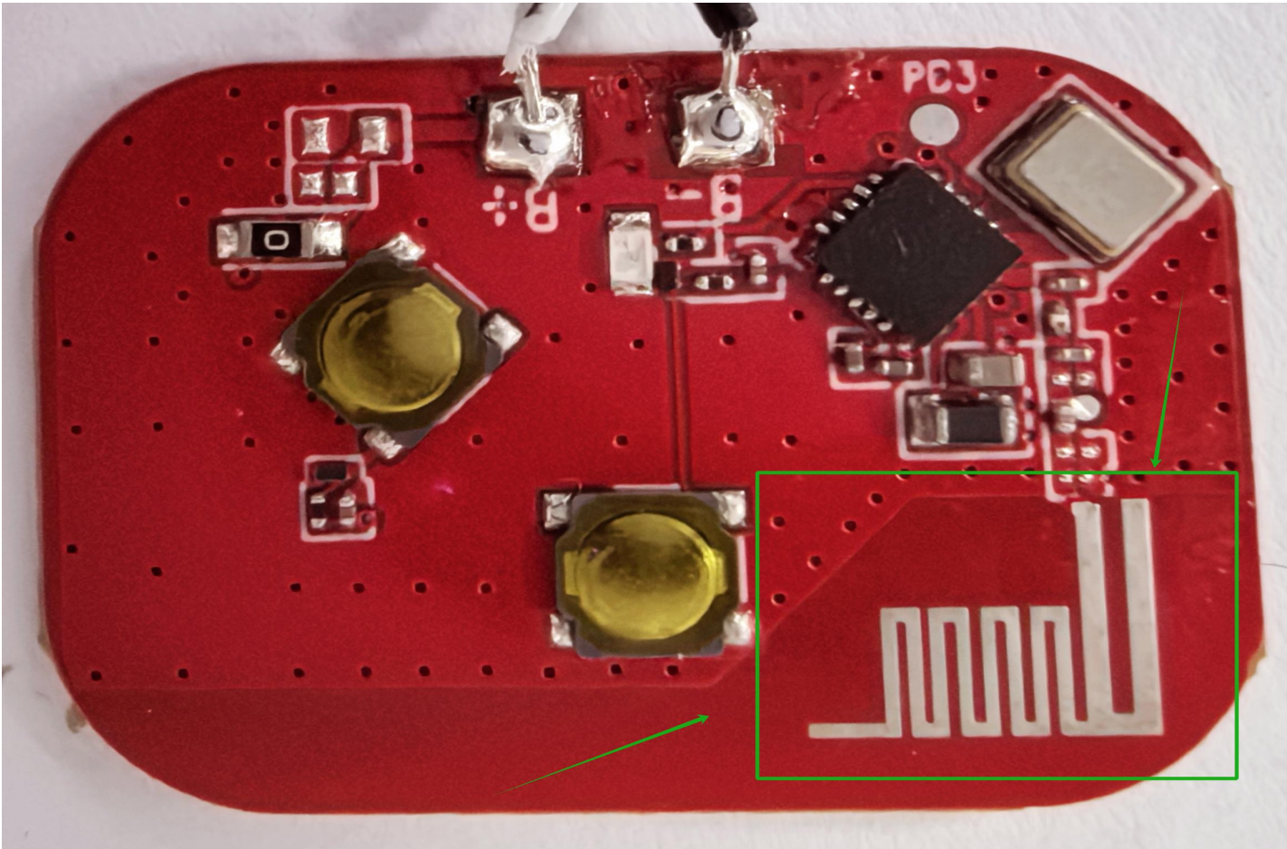
Antenna Photo & Length (mm)
