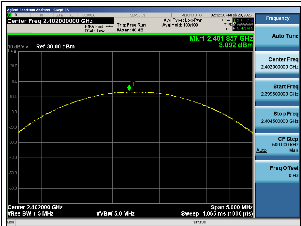
Test_Graph_EDR_ANT1_2402_2Mbps_Peak Power
