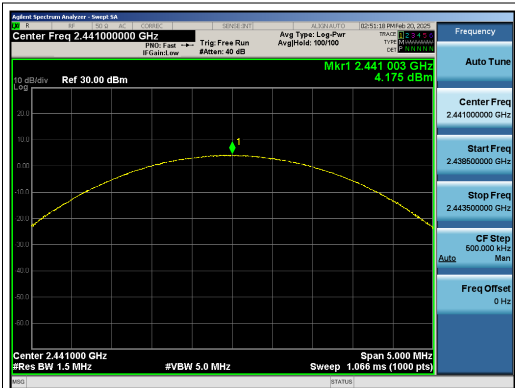
Test_Graph_EDR_ANT1_2441_3Mbps_Peak Power
