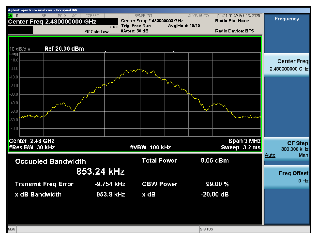
Test_Graph_BR_ANT1_2480_1Mbps_OBW
