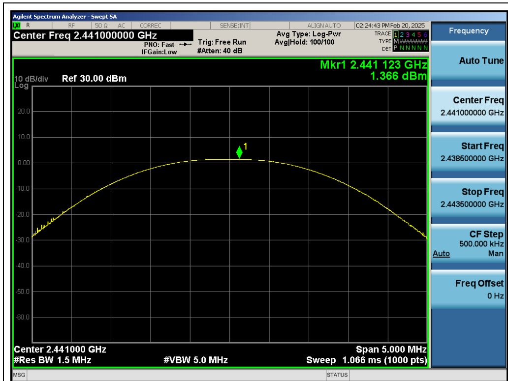
Test_Graph_BR_ANT1_2441_1Mbps_Peak Power
