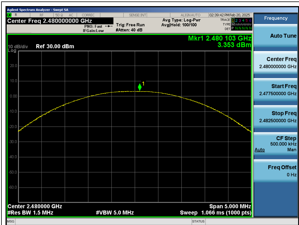
Test_Graph_EDR_ANT1_2480_2Mbps_Peak Power
