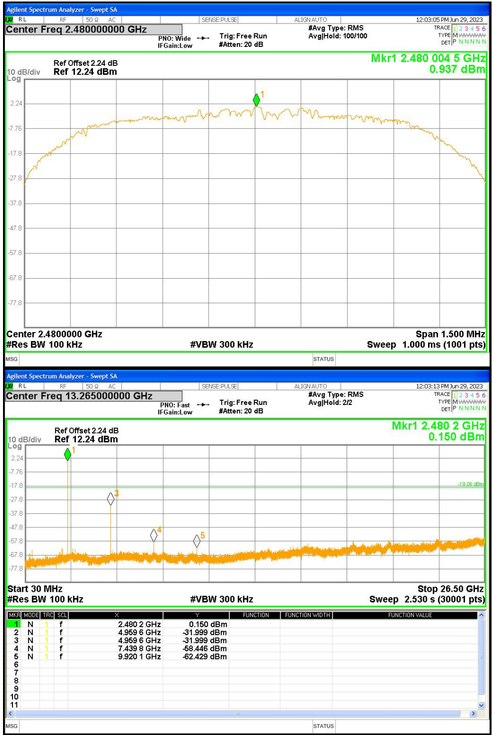
30MHz~26.5GHz
