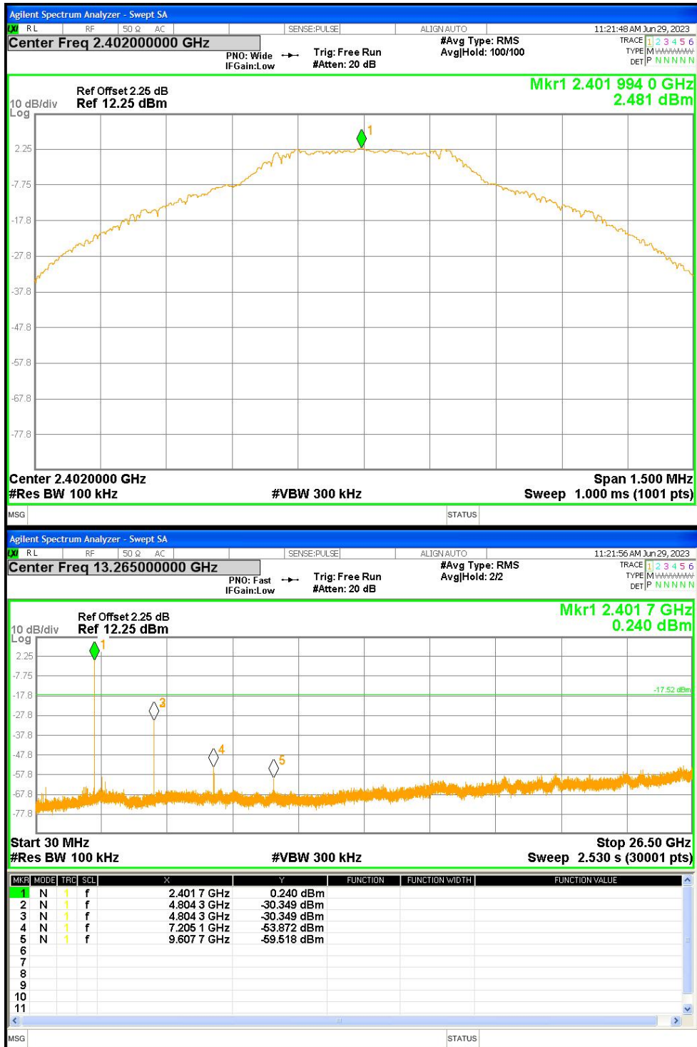
30MHz~26.5GHz
