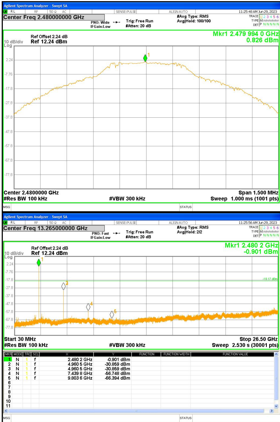
30MHz~26.5GHz
