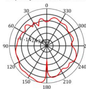
frequency=2500MHz, X-Z Plane
