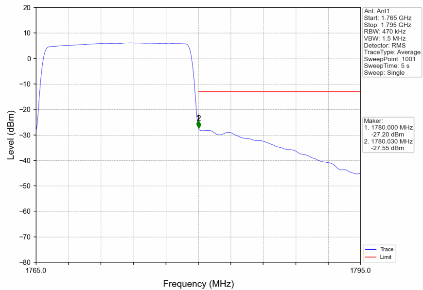
Band66_15MHz_16QAM_HCH_1772.5MHz_RB_75_0_NTNV
