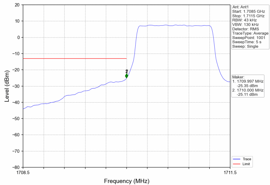
Band66_1.4MHz_16QAM_LCH_1710.7MHz_RB_6_0_NTNV
