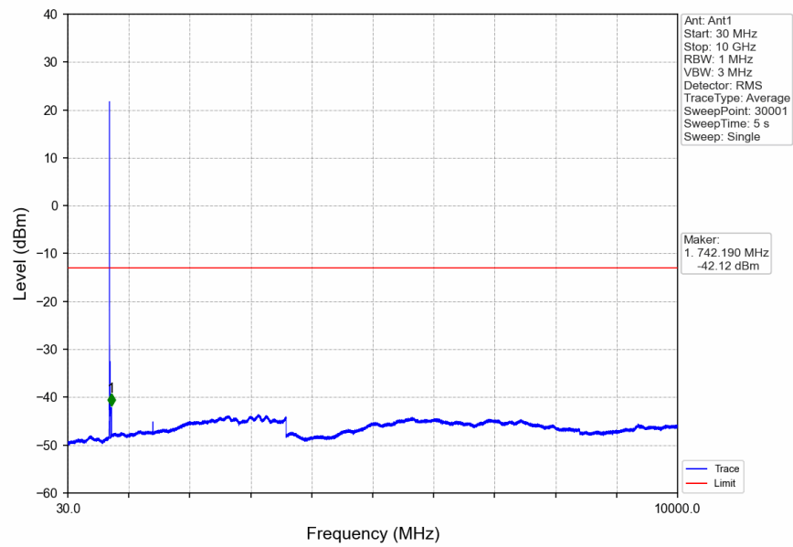
Band12_5MHz_16QAM_HCH_713.5MHz_RB_1_0_NTNV
