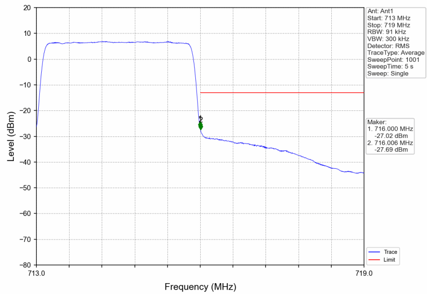
Band12_3MHz_16QAM_HCH_714.5MHz_RB_15_0_NTNV
