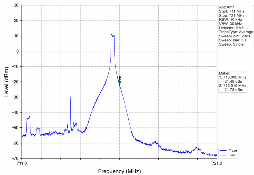
Band12_5MHz_QPSK_HCH_713.5MHz_RB_1_24_NTNV
