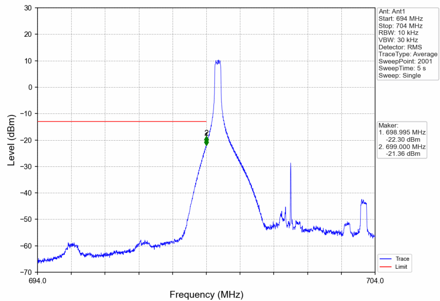
Band12_5MHz_16QAM_LCH_701.5MHz_RB_1_0_NTNV
