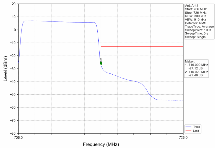
Band12_10MHz_16QAM_HCH_711MHz_RB_50_0_NTNV
