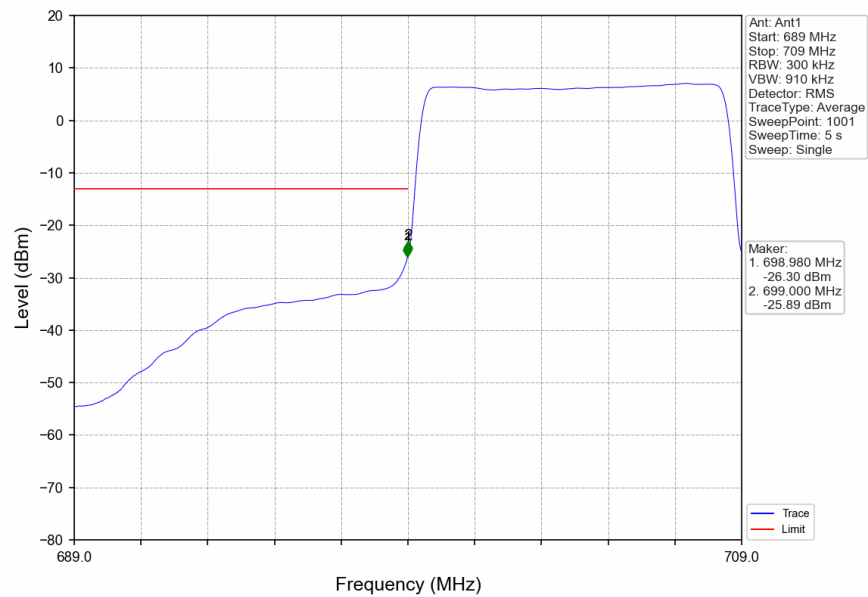
Band12_10MHz_16QAM_LCH_704MHz_RB_50_0_NTNV
