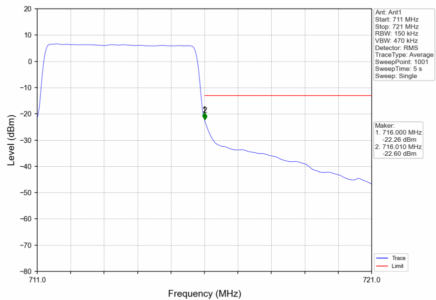
Band12_5MHz_16QAM_HCH_713.5MHz_RB_25_0_NTNV
