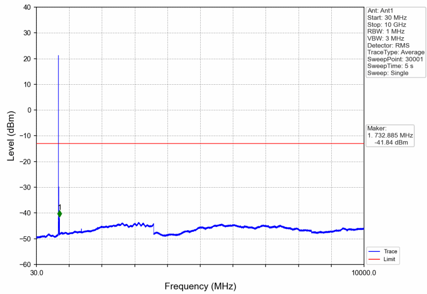
Band12_5MHz_16QAM_LCH_701.5MHz_RB_25_0_NTNV
