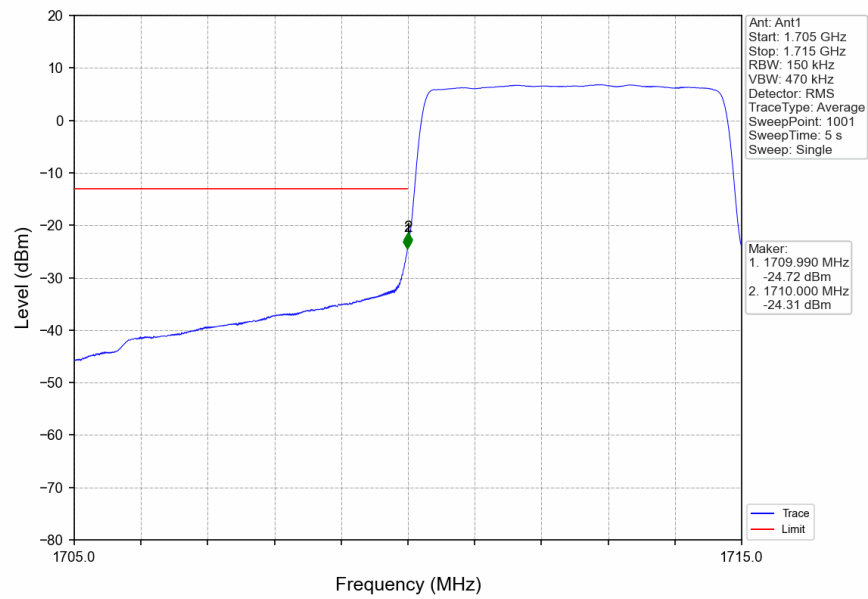
Band4_5MHz_16QAM_LCH_1712.5MHz_RB_25_0_NTNV
