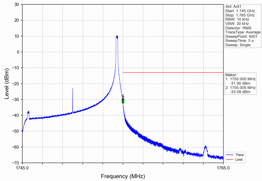
Band4_10MHz_16QAM_HCH_1750MHz_RB_50_0_NTNV
