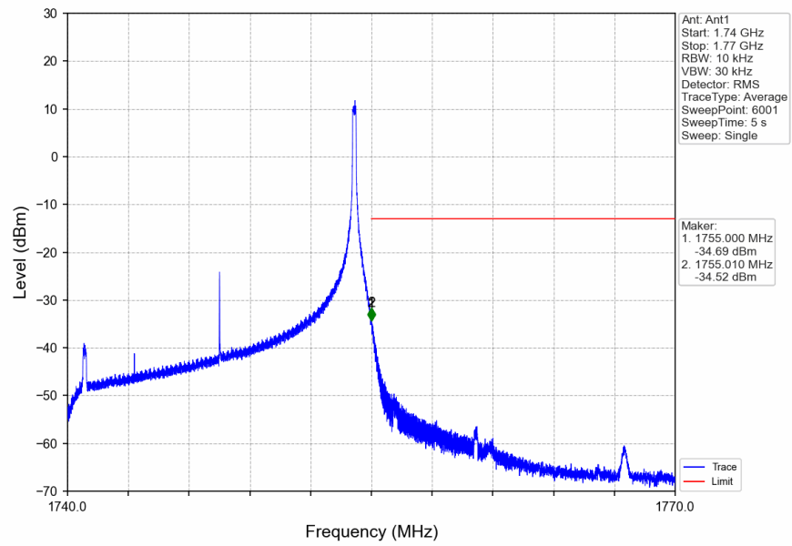
Band4_15MHz_16QAM_HCH_1747.5MHz_RB_75_0_NTNV
