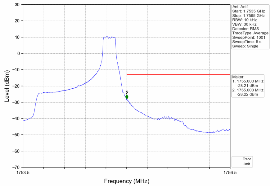
Band4_1.4MHz_16QAM_HCH_1754.3MHz_RB_6_0_NTNV
