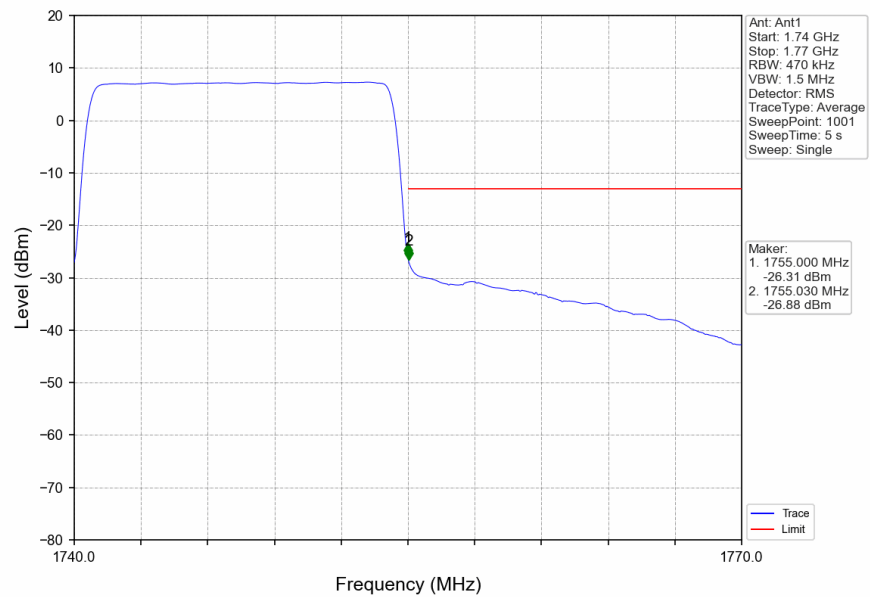
Band4_15MHz_16QAM_HCH_1747.5MHz_RB_75_0_NTNV
