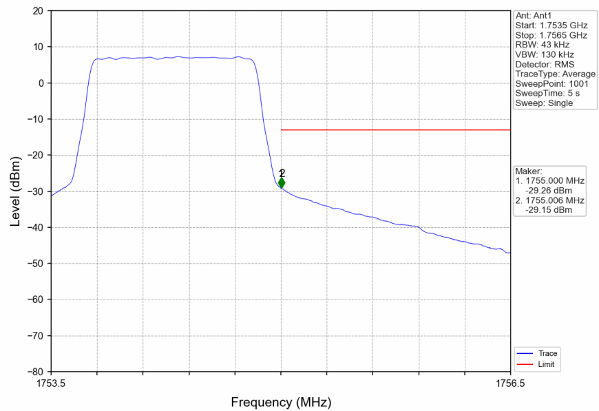
Band4_1.4MHz_16QAM_HCH_1754.3MHz_RB_6_0_NTNV
