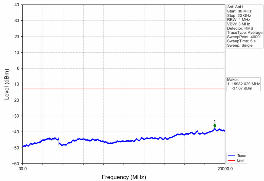
Band4_5MHz_16QAM_HCH_1752.5MHz_RB_1_0_NTNV
