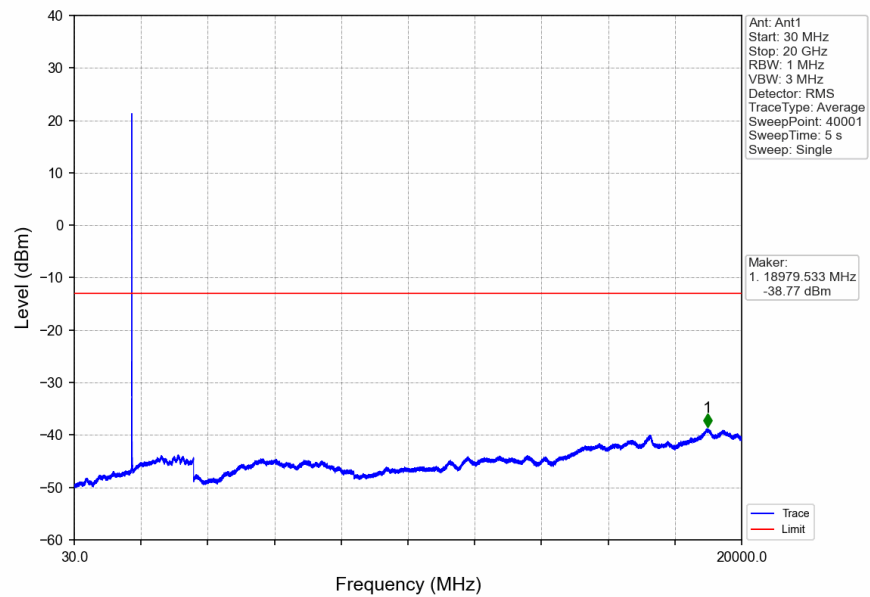
Band4_3MHz_16QAM_HCH_1753.5MHz_RB_1_0_NTNV
