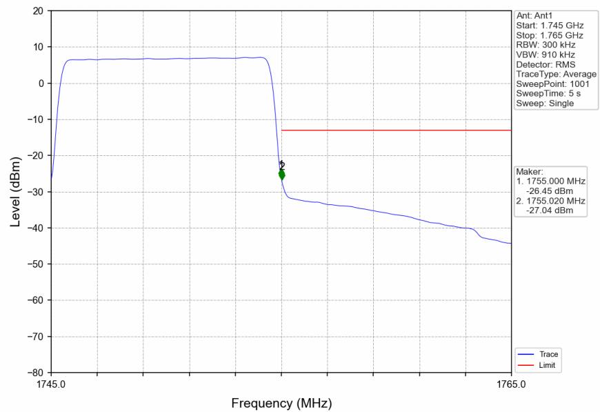
Band4_10MHz_16QAM_HCH_1750MHz_RB_50_0_NTNV
