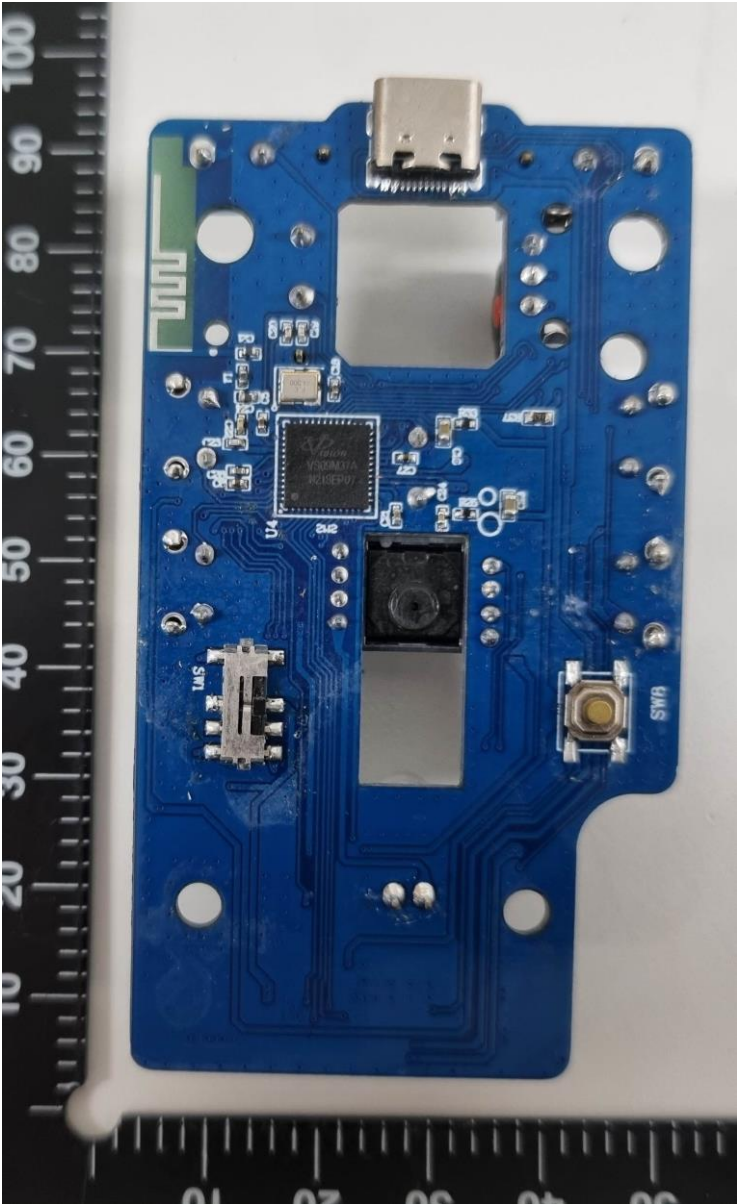
Main Board (mouse, rear)
