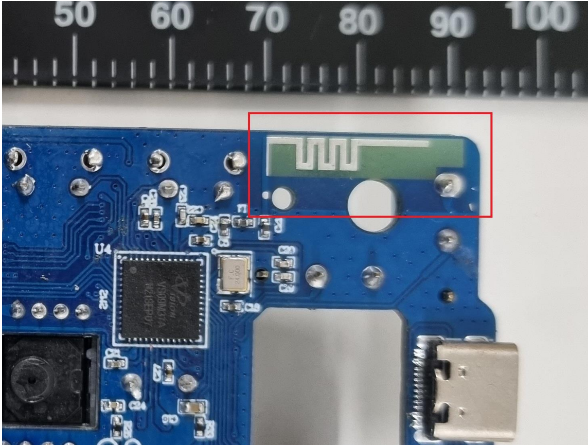
Antenna (Close-up and Location)
