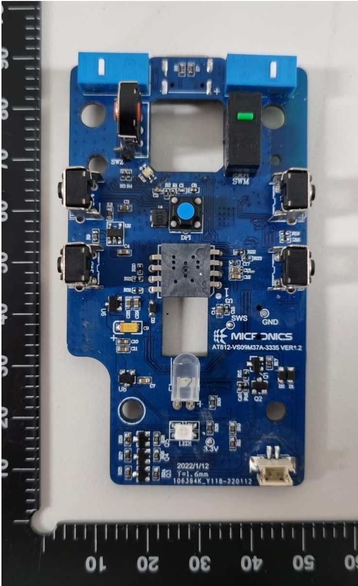
Main Board(mouse, front)
