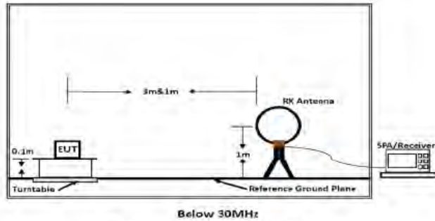
Figure 1. Below 30MHz
