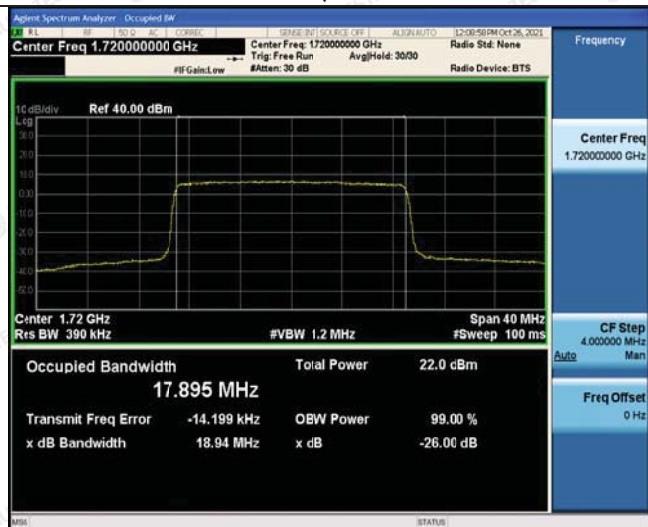
16QAM
