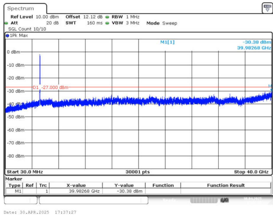
Tx. Spurious NVNT ac80 5775MHz Ant1 Emission
