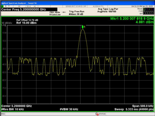
NT/NV_Antenna 0 IEEE 802.11n_Channel 40_20MHz
