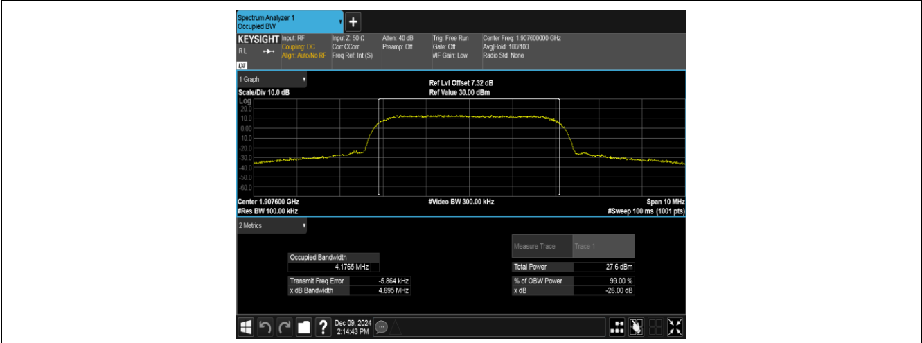
Band2-9538-2-PASS
