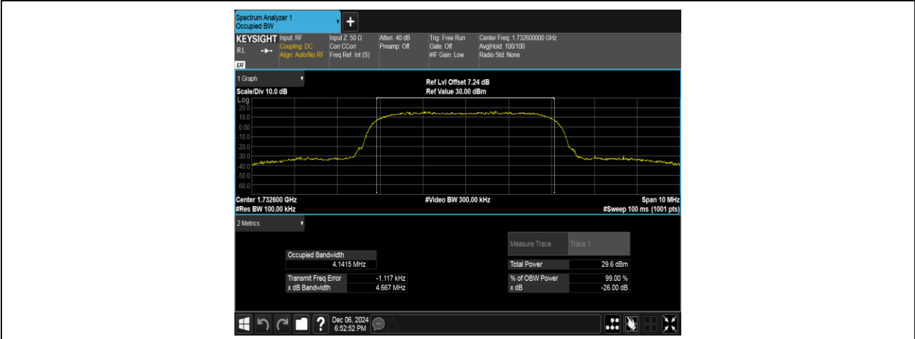
Band4-1413-1-PASS
