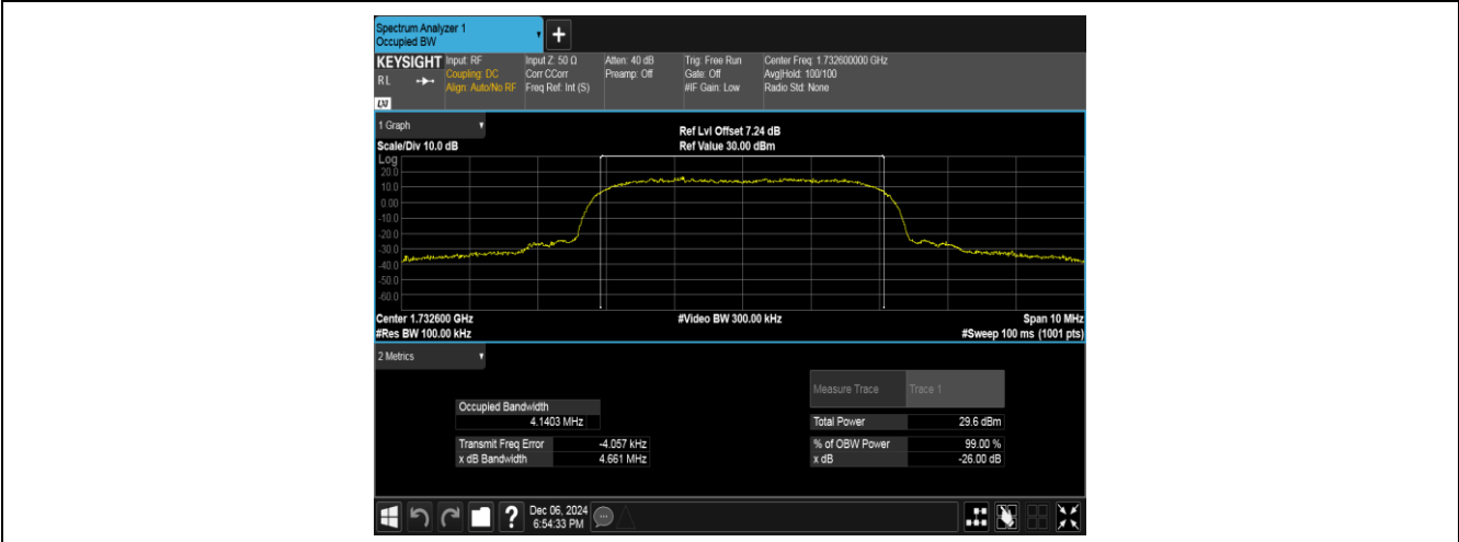
Band4-1413-2-PASS
