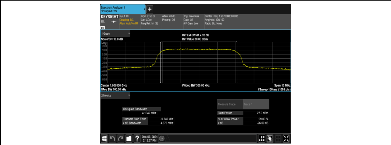
Band2-9538-1-PASS
