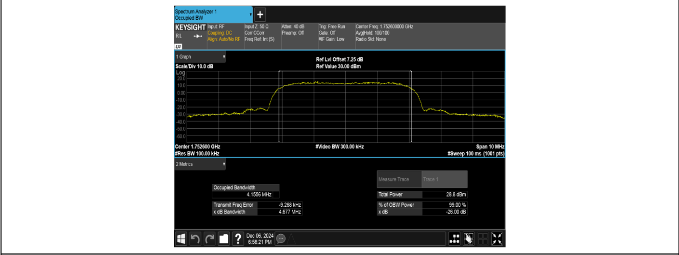
Band4-1513-4-PASS
