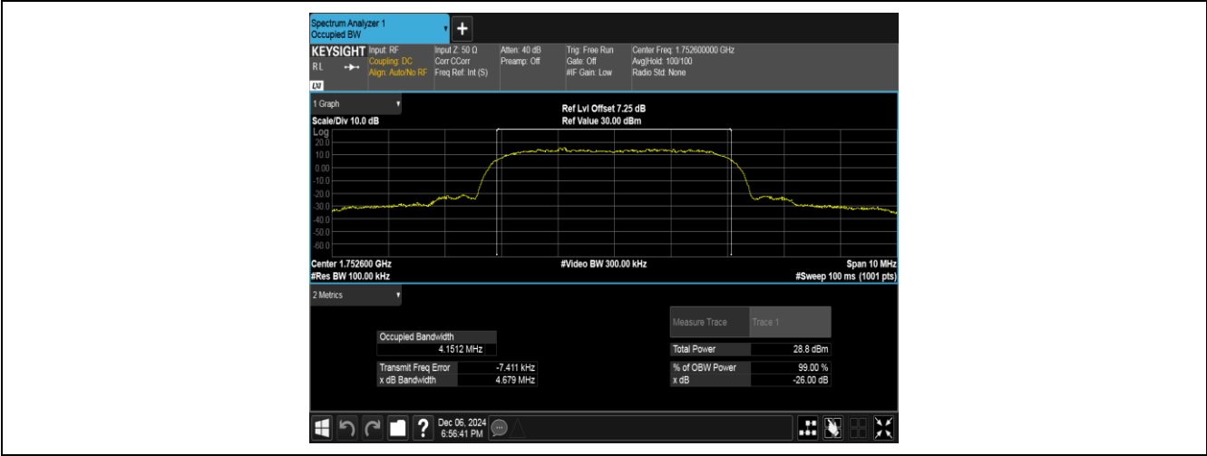
Band4-1513-3-PASS
