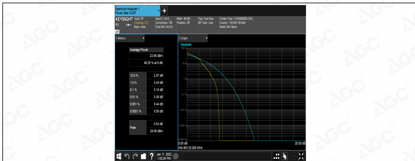
Band25-10MHz-16QAM-26090-50RB#0
