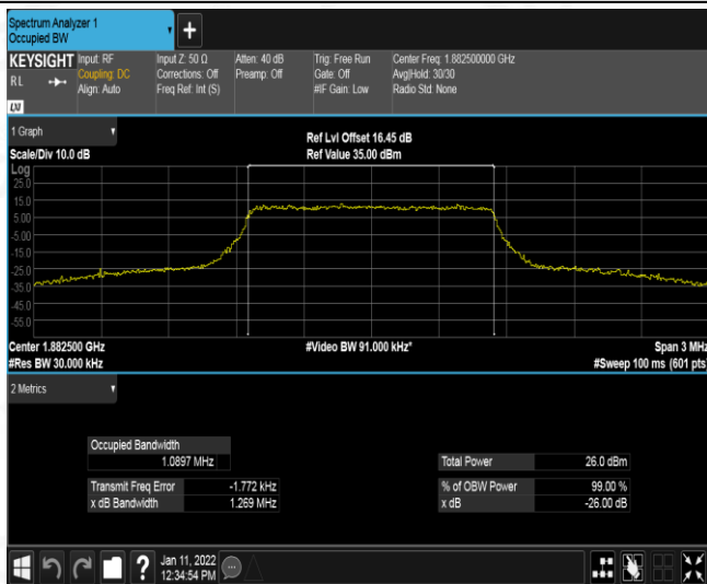
Band25-1.4MHz-16QAM-26365-6RB#0
