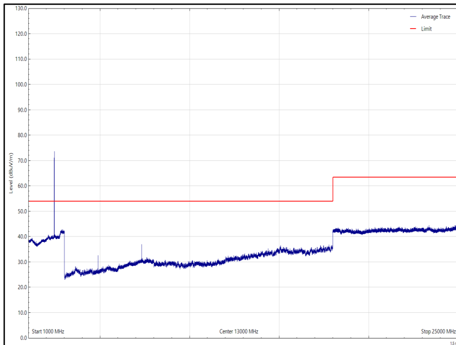
Figure 17 - Proprietary - X, 2440 MHz, 1 GHz to 25 GHz, Horizontal (Average)
