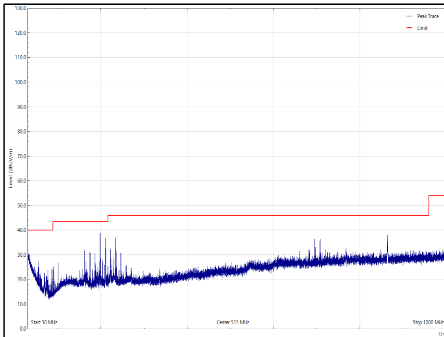
Figure 10 - Proprietary - X, 2402 MHz, 30 MHz to 1 GHz, Horizontal (Peak)
