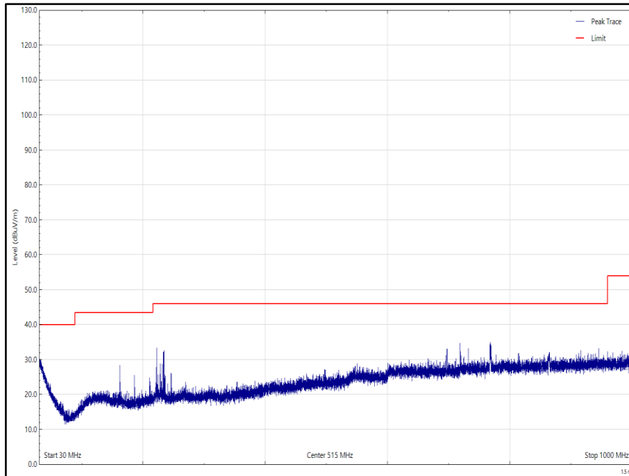
Figure 28 - Proprietary - Y, 2402 MHz, 30 MHz to 1 GHz, Horizontal (Peak)
