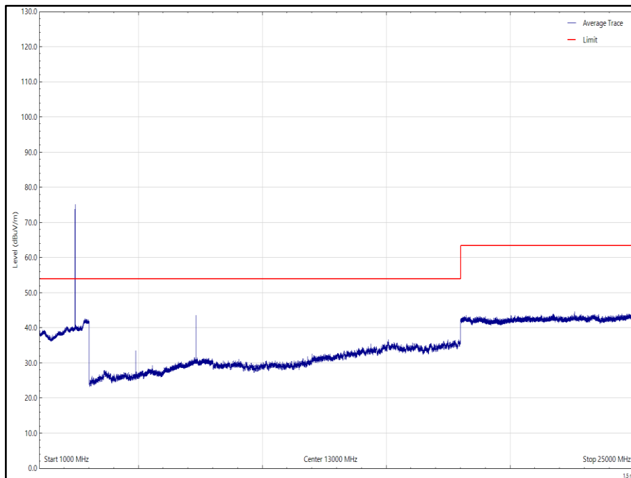
Figure 35 - Proprietary - Y, 2440 MHz, 1 GHz to 25 GHz, Horizontal (Average)
