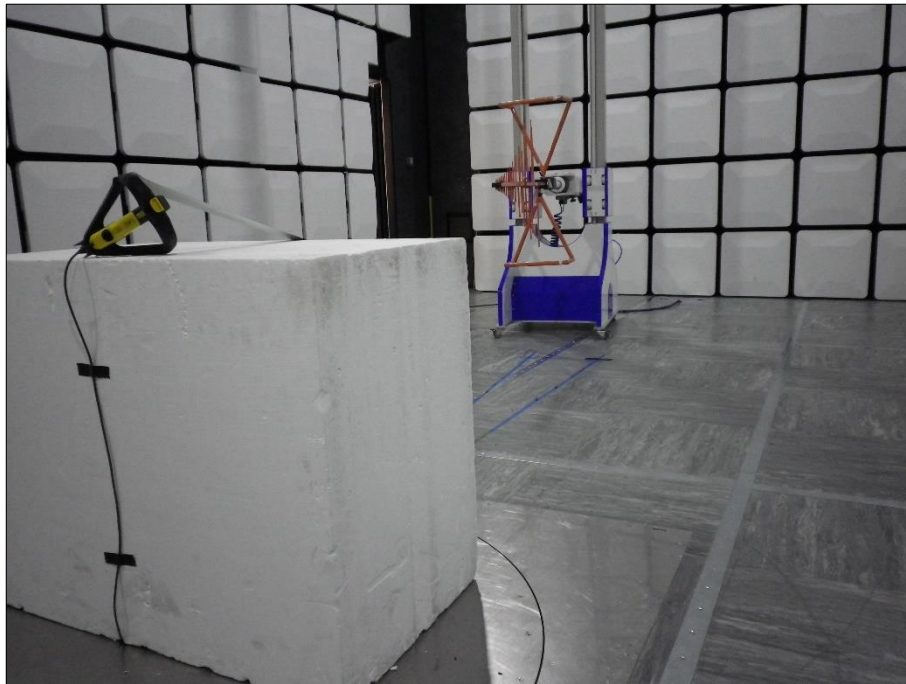
Figure 68 - Test Setup - 30 MHz to 1 GHz - Z Orientation
