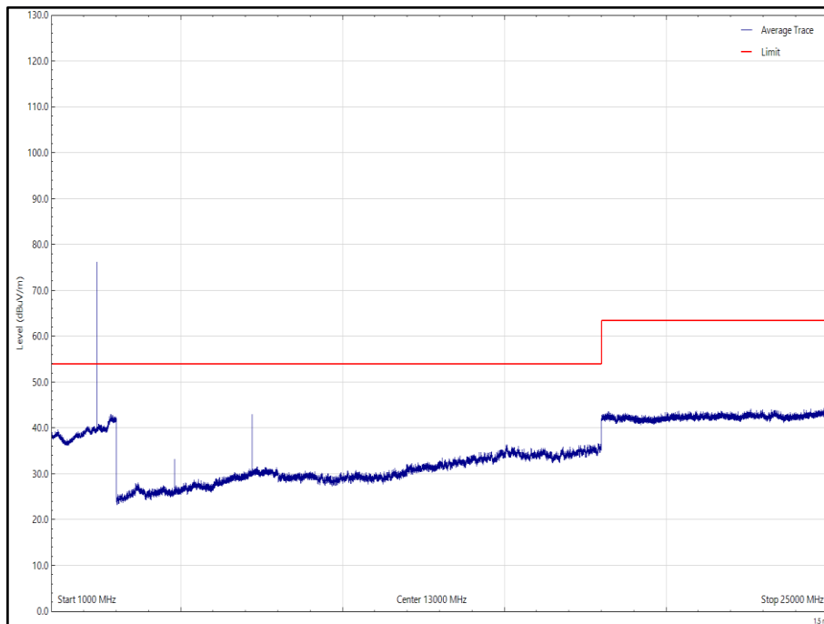
Figure 29 - Proprietary - Y, 2402 MHz, 1 GHz to 25 GHz, Horizontal (Average)
