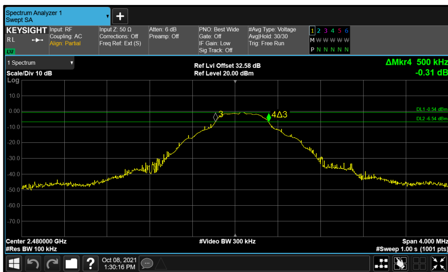
Figure 8 - A (A) 2480 MHz 6 dB Bandwidth
