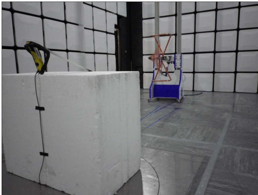
Figure 67 - Test Setup - 30 MHz to 1 GHz - Y Orientation
