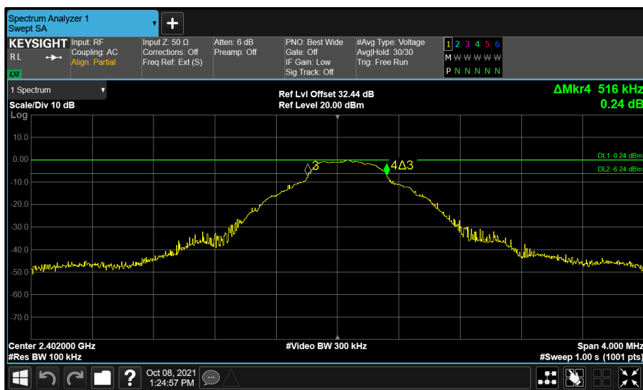
Figure 4 - A (A) 2402 MHz 6 dB Bandwidth
