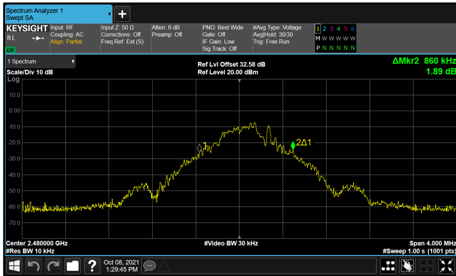
Figure 7 - A (A) 2480 MHz 99% Bandwidth
