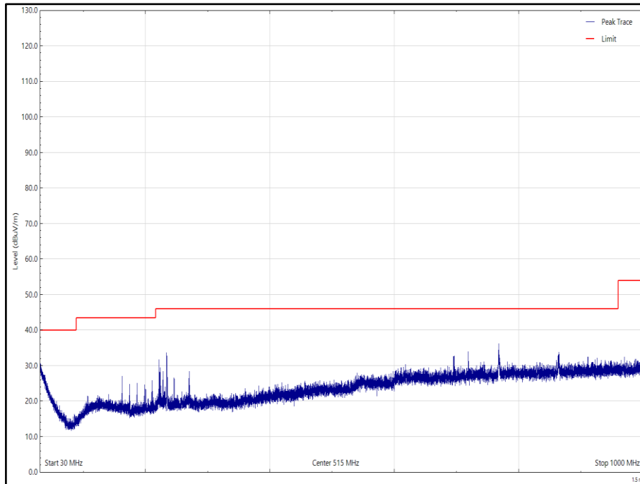
Figure 34 - Proprietary - Y, 2440 MHz, 30 MHz to 1 GHz, Horizontal (Peak)
