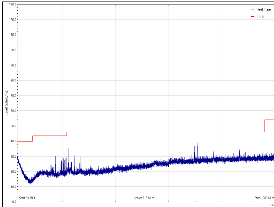
Figure 16 - Proprietary - X, 2440 MHz, 30 MHz to 1 GHz, Horizontal (Peak)
