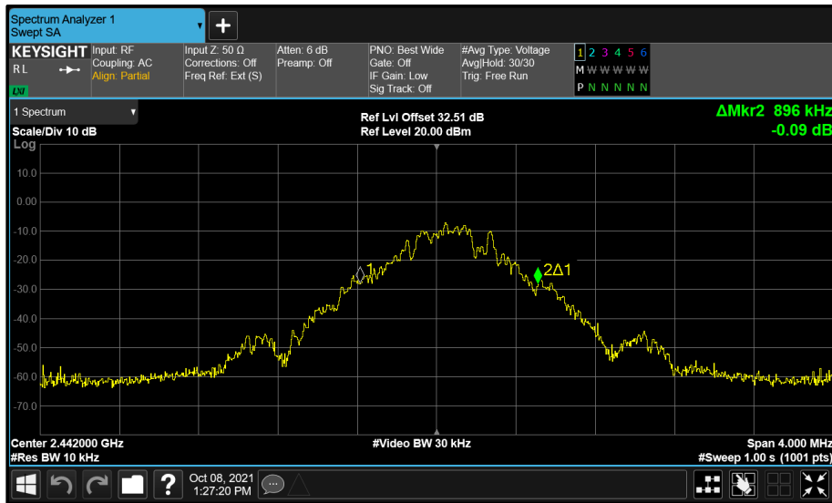
Figure 5 - A (A) 2442 MHz 99% Bandwidth
