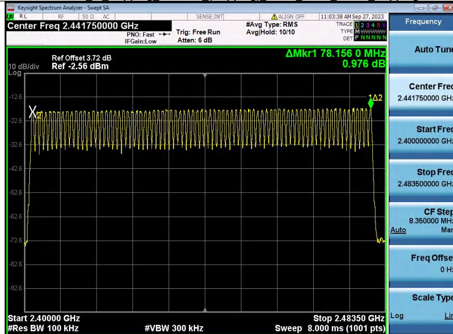
Number of Hopping Channel (Hopping) NVNT ANT1 1-DH5 Hopping
