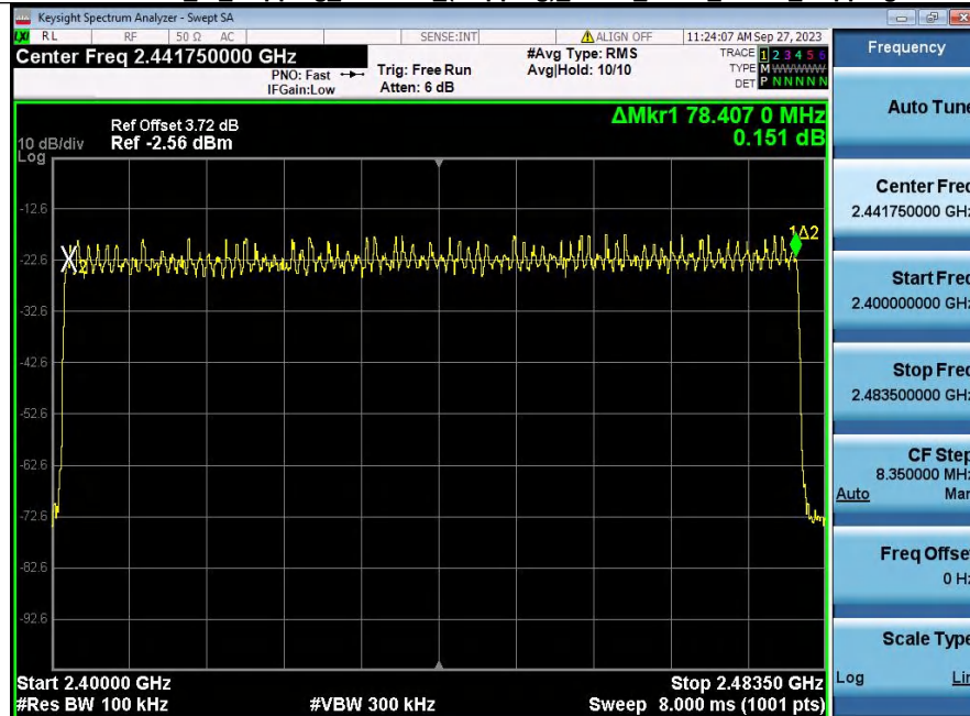
Number of Hopping Channel (Hopping) NVNT ANT1 2-DH5 Hopping
