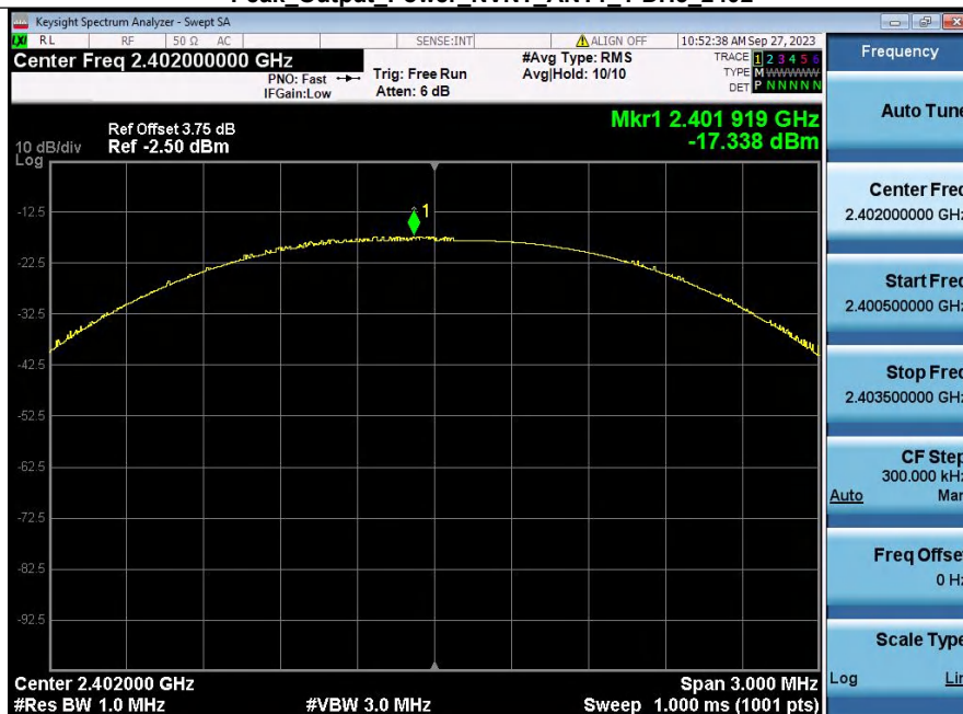
Peak Output Power NVNT_ANT1_1-DH5_2402
