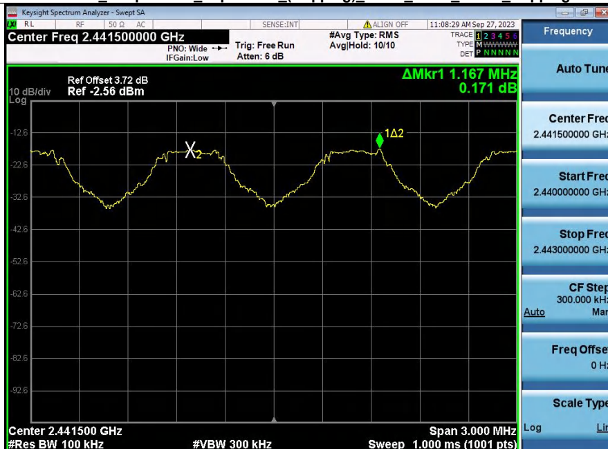
Carrier_Frequencies_Separation_(Hopping)_NVNT_ANT1_1-DH5_Hopping
