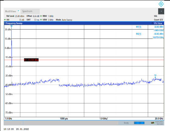
Band2-15MHz-16QAM-18900-1RB#0-Range2: 1000~20000MHz
