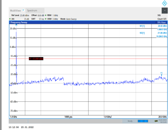
Band2-15MHz-16QAM-18675-1RB#0-Range2: 1000~20000MHz
