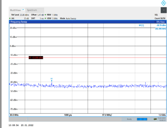
Band2-10MHz-QPSK-18900-1RB#0-Range1: 0~1000MHz
