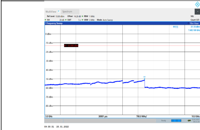
Band5-4132-3000~10000MHz
