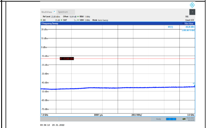
Band5-4182-1000~3000MHz
