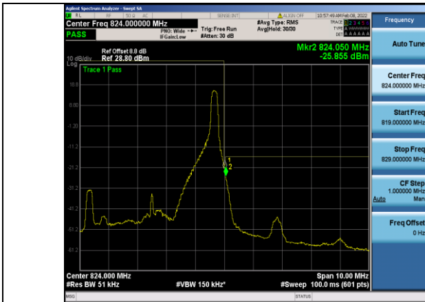
Band26-5MHz-QPSK-26765-1RB#24
