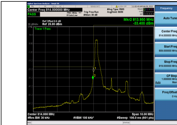
Band26-3MHz-16QAM-26705-1RB#0
