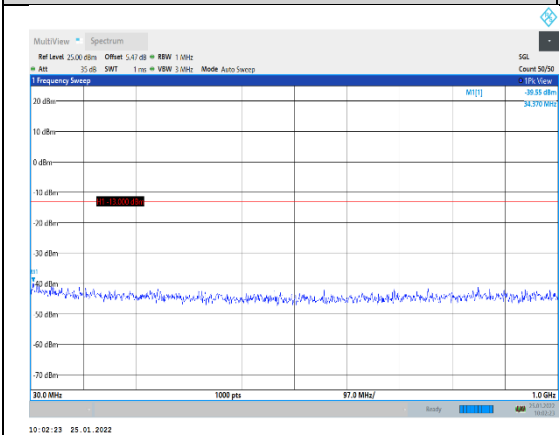
Band2-3MHz-16QAM-18900-1RB#0-Range1: 0~1000MHz
