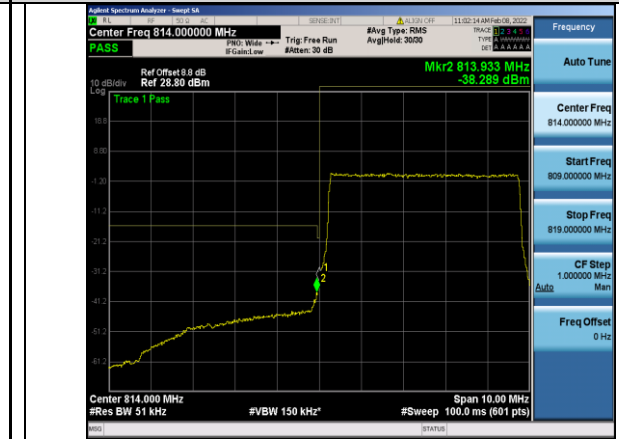
Band26-5MHz-QPSK-26715-25RB#0
