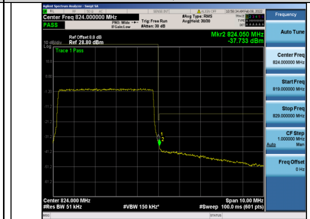
Band26-5MHz-16QAM-26765-25RB#0
