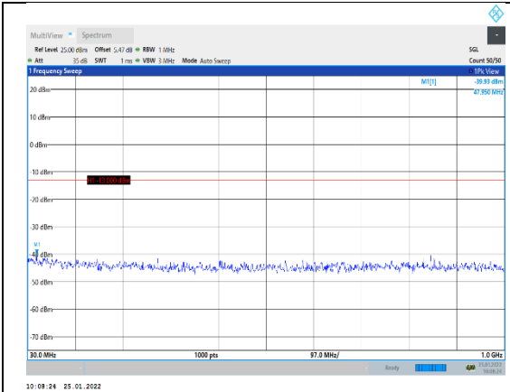
Band2-10MHz-16QAM-18650-1RB#0-Range 30~1000MHz
