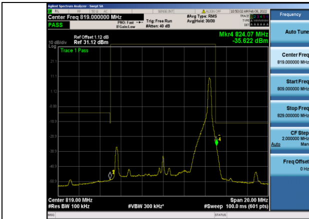
Band26-10MHz-16QAM-26740 Right-1RB#49
