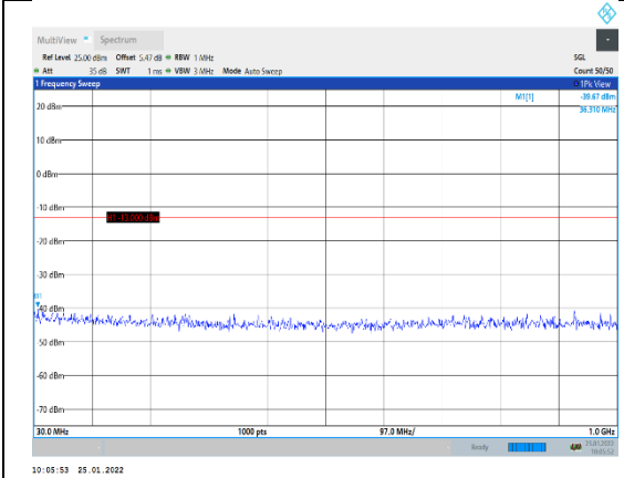
Band2-5MHz-16QAM-18900-1RB#0-Range1: 0~1000MHz
