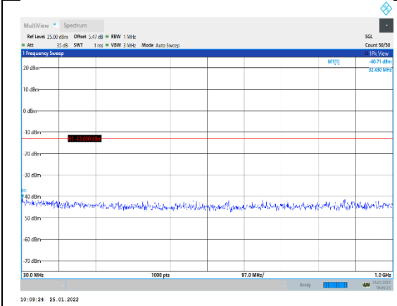
Band2-10MHz-16QAM-18900-1RB#0-Range 30~1000MHz
