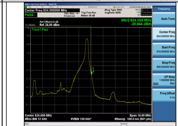
Band26-5MHz-16QAM-26765-1RB#24
