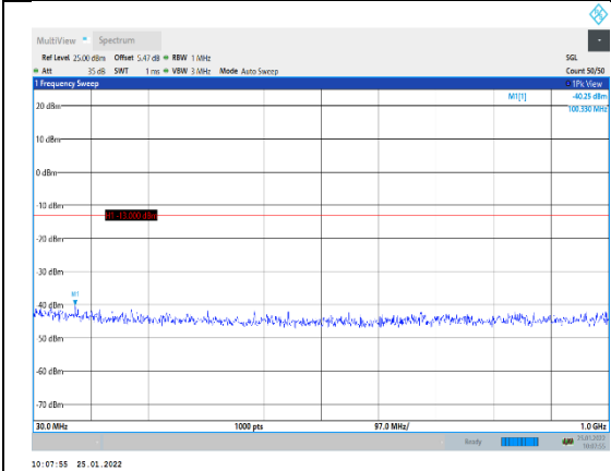
Band2-10MHz-QPSK-18650-1RB#0-Range1: 0~1000MHz
