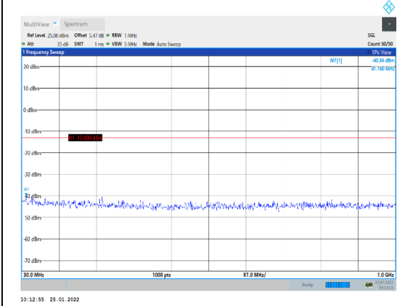
Band2-15MHz-16QAM-18900-1RB#0-Range 30~1000MHz
