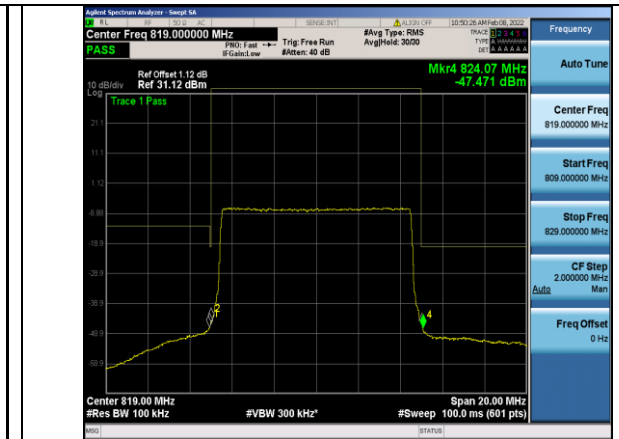
Band26-10MHz-16QAM-26740 Right-50RB#0
