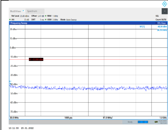
Band2-15MHz-16QAM-18675-1RB#0-Range 30~1000MHz
