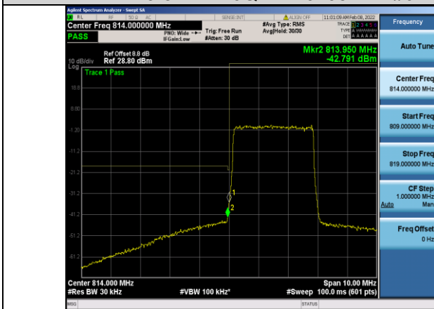
Band26-3MHz-16QAM-26705-15RB#0
