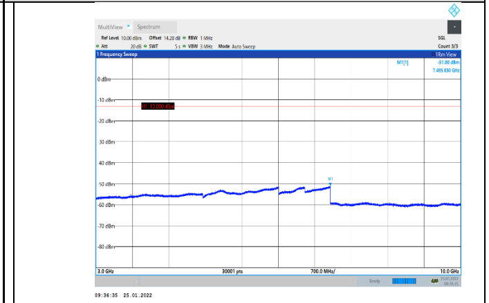
Band5-4182-3000~10000MHz
