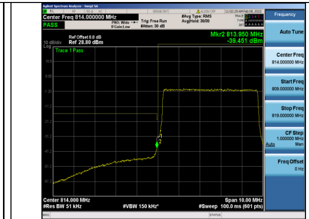
Band26-5MHz-16QAM-26715-25RB#0
