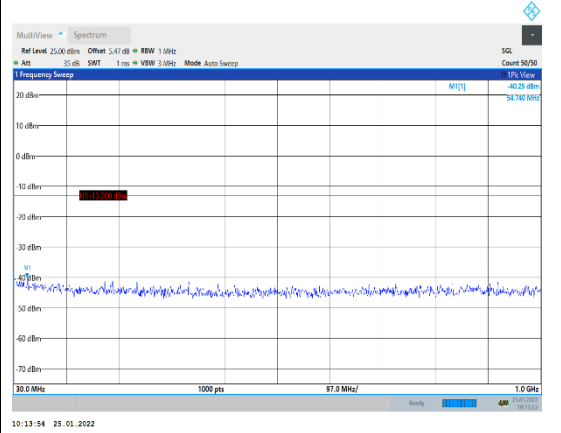
Band2-15MHz-16QAM-19125-1RB#0-Range1: 30~1000MHz
