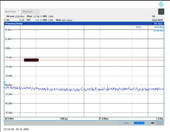
Band2-10MHz-16QAM-19150-1RB#0-Range1: 30~1000MHz
