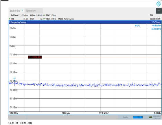
Band2-3MHz-16QAM-18615-1RB#0-Range1: 0~1000MHz
