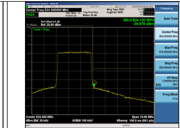
Band26-3MHz-16QAM-26775-15RB#0
