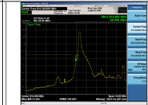
Band26-5MHz-QPSK-26715-1RB#0
