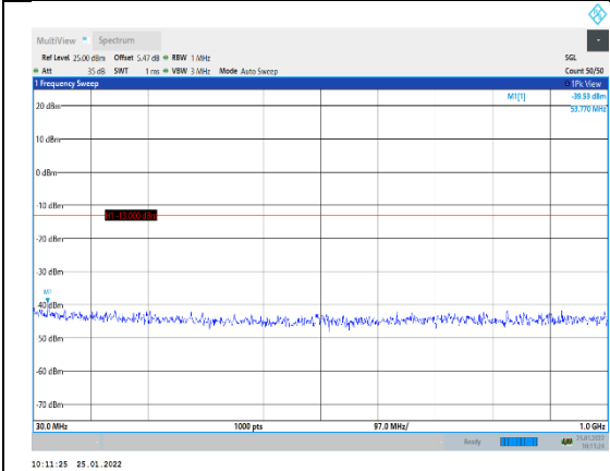
Band2-15MHz-QPSK-18675-1RB#0-Range1: 0~1000MHz
