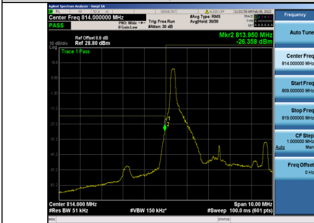
Band26-5MHz-16QAM-26715-1RB#0
