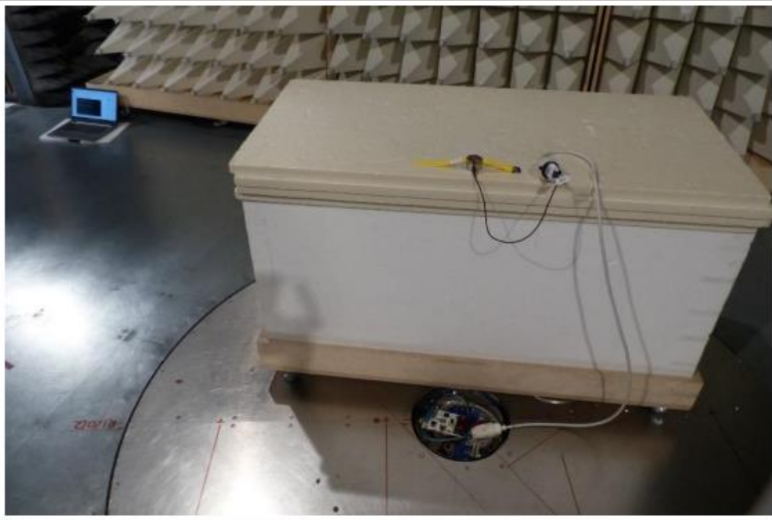
Test setup EUT Configuration 2
