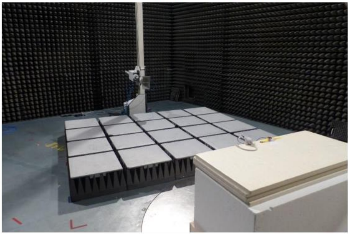
Test setup EUT Configuration 2 1000-13000MHz
