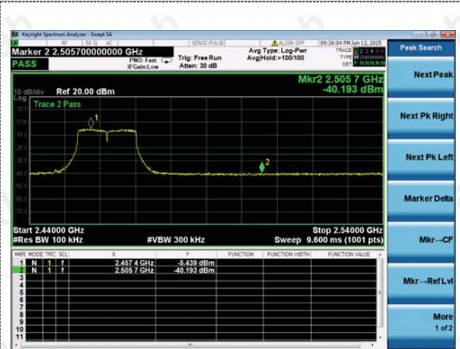
Right bandedge
