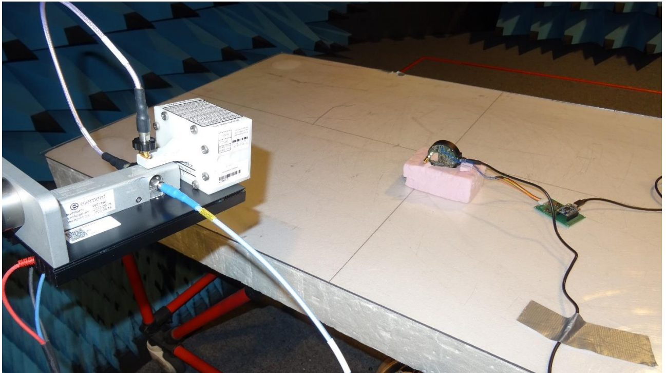
Picture 7: FS-SAC, exploratory radiated emission test 17 GHz – 25 GHz (front view)
