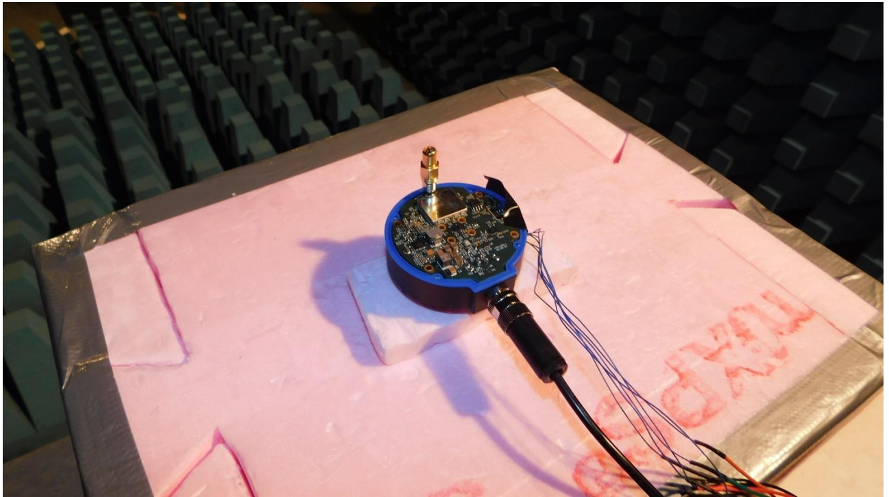
Picture 11: EUT position X
