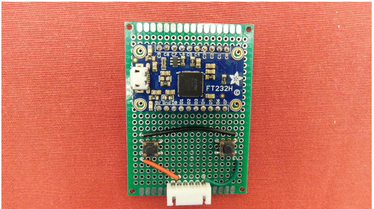
Picture 15: Adapter – top view
