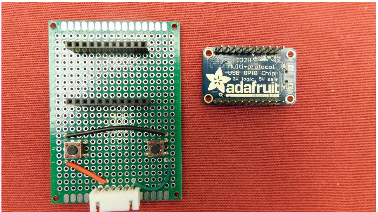
Picture 19: Adapter without module – rear view
