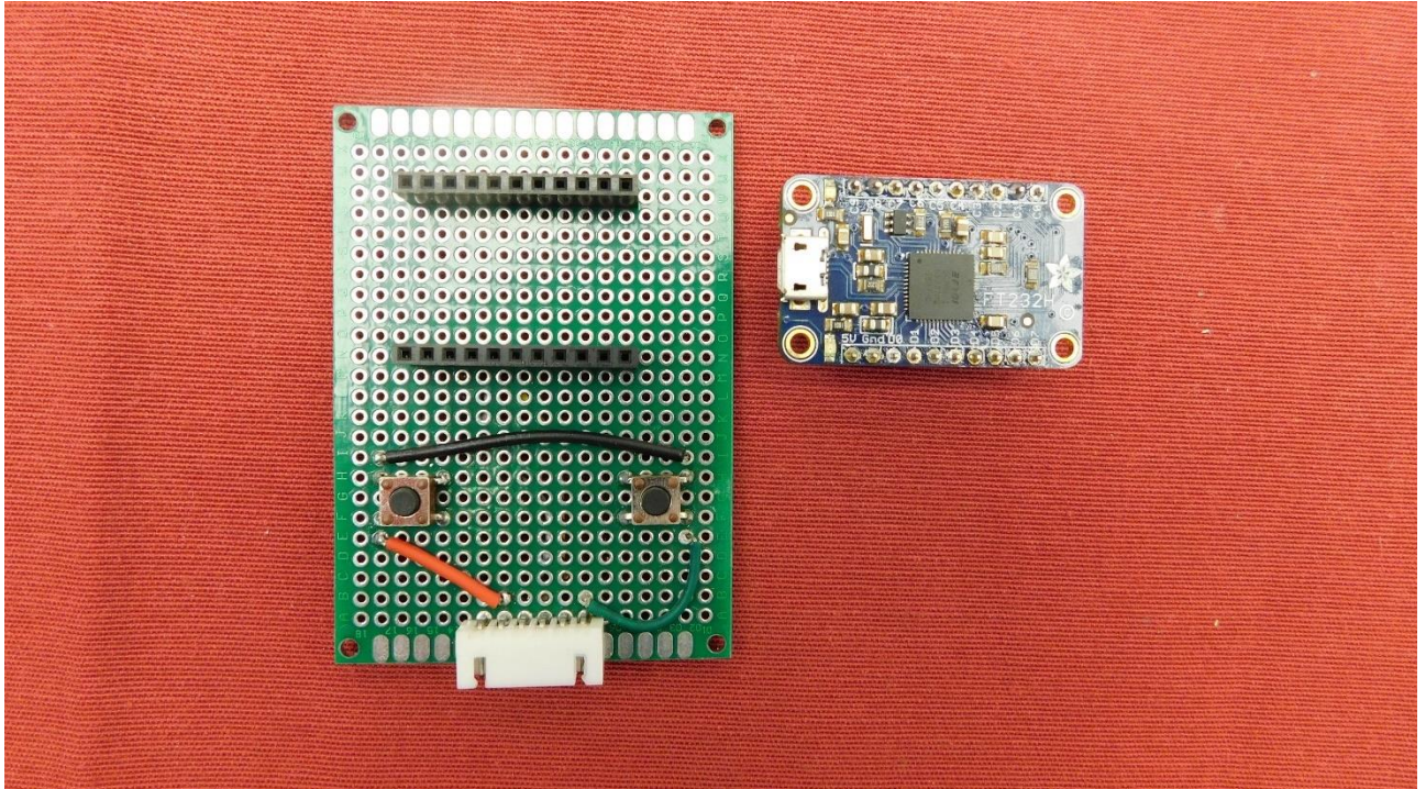
Picture 18: Adapter without module– top view
