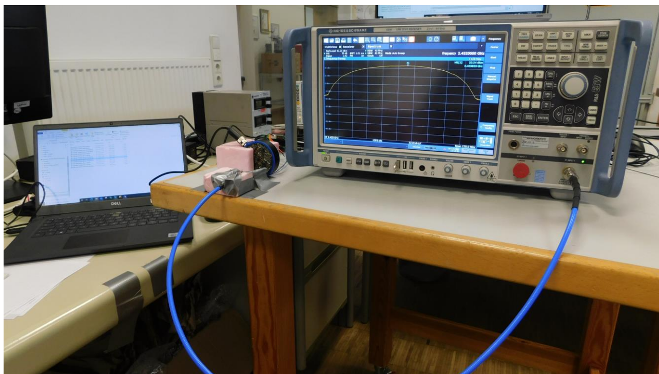
Picture 11: Conducted measurements – conducted output power
