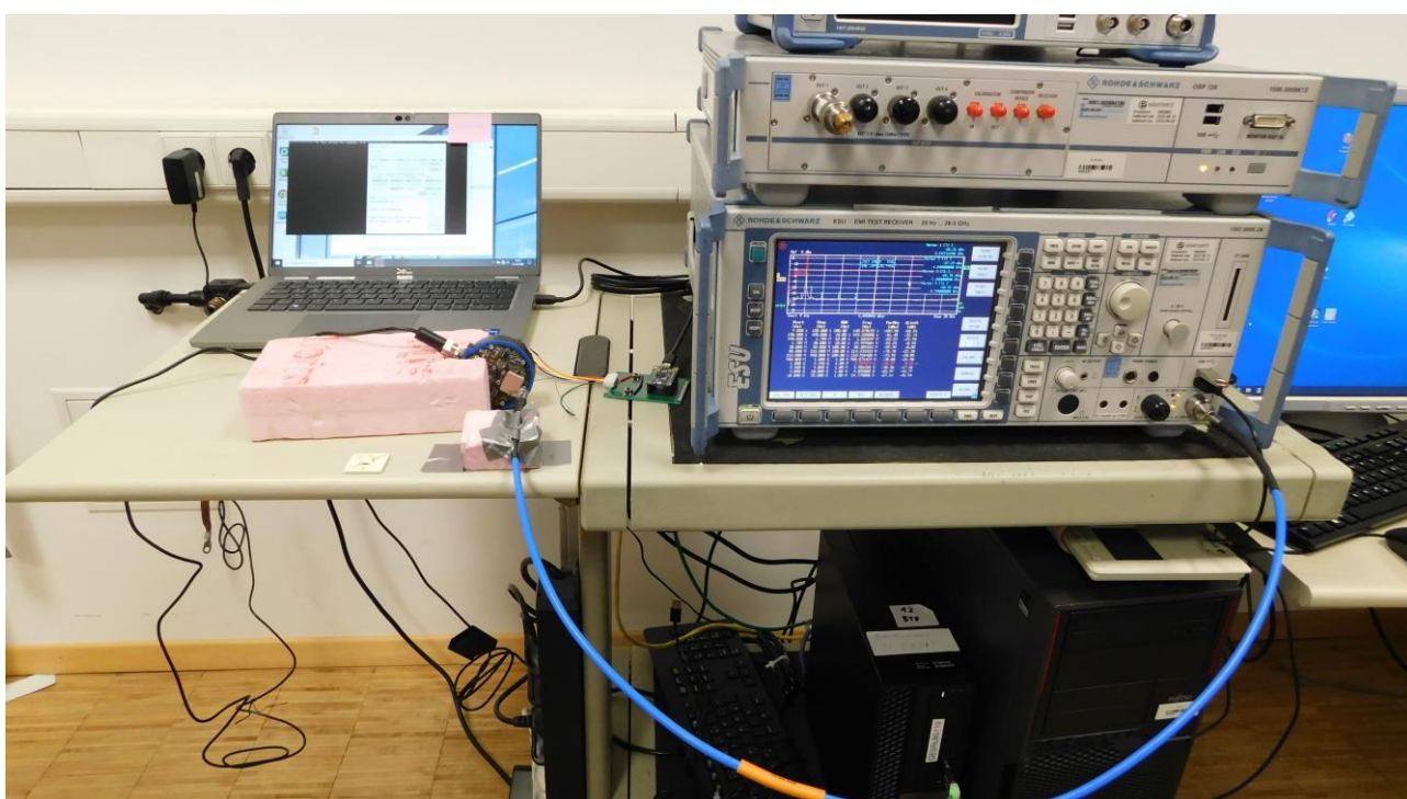
Picture 10: Conducted measurements except conducted output power
