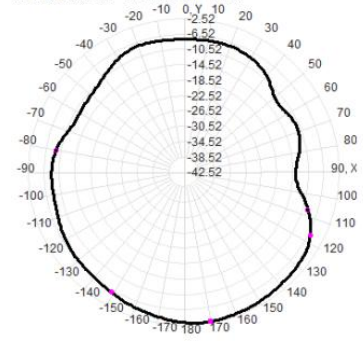
Total(H-XY), Max=-3.15dBi, CirD=10.94
