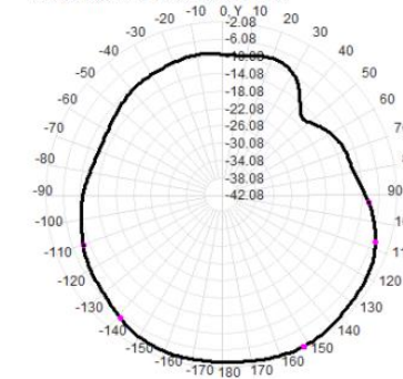
Total(H-XY), Max=-2.55dBi, CirD=13.99
