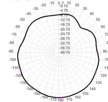
Total(H-XY), Max=-2.01dBi, CirD=10.10
