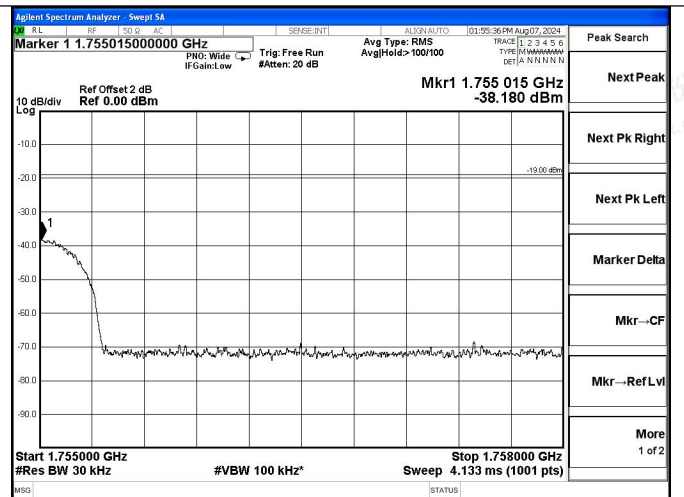
AWS Band UL-CDMA Right Side AGC+10dB
