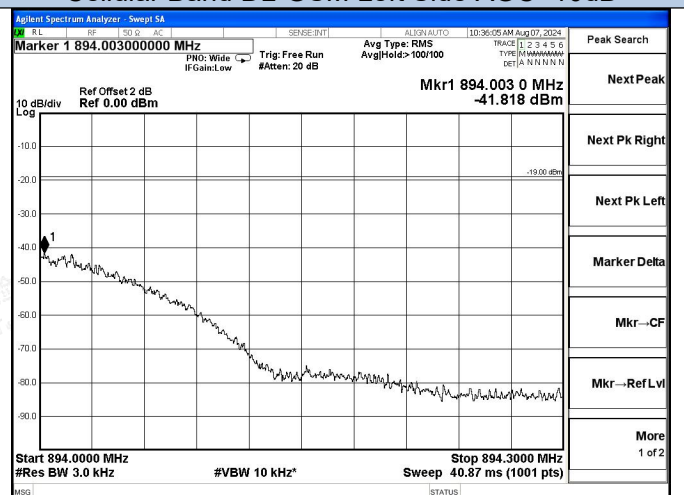
Cellular Band DL-GSM Right Side AGC+10dB
