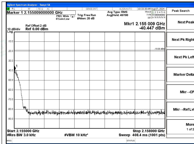
AWS Band DL-GSM Right Side Pre AGC
