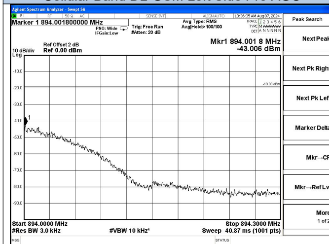
Cellular Band DL-GSM Right Side Pre AGC
