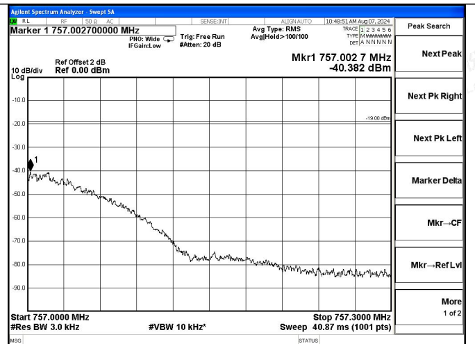
Upper 700 Band DL-GSM Right Side AGC+10dB
