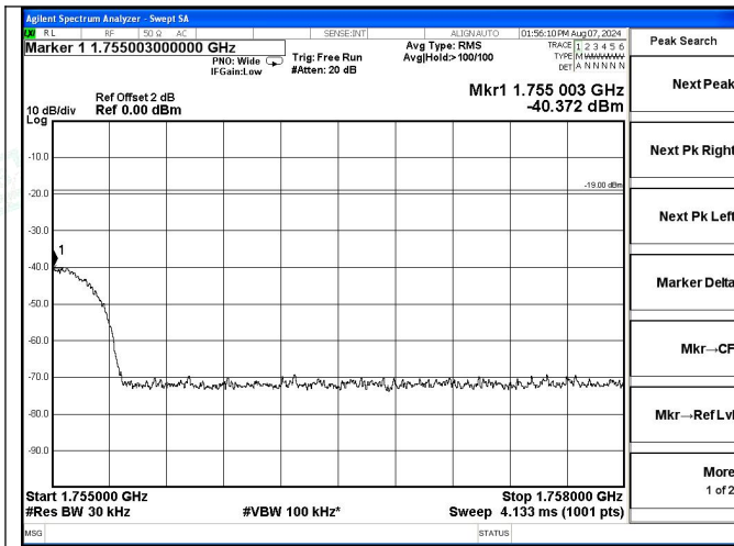
AWS Band UL-CDMA Right Side Pre AGC
