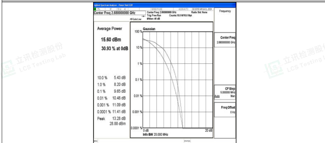
Band41-20MHz-16QAM-41490-100RB#0-PASS
