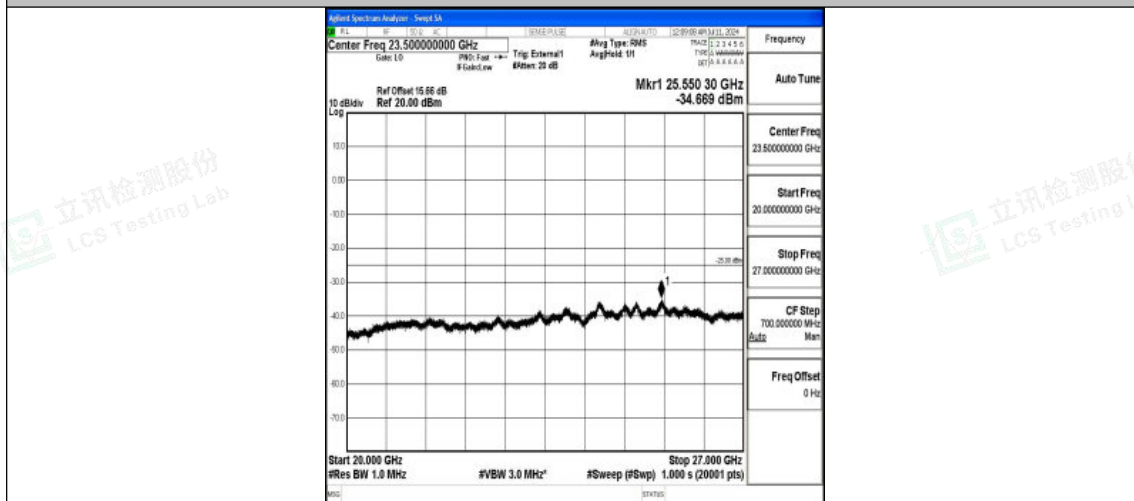
Band41_5MHz_QPSK_39675_1RB#0_20000~27000_20000~27000
