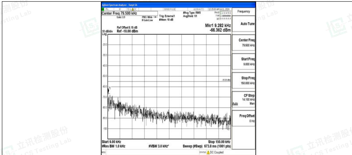
Band41_5MHz_QPSK_41565_1RB#0_0.009~0.15_0.009~0.15
