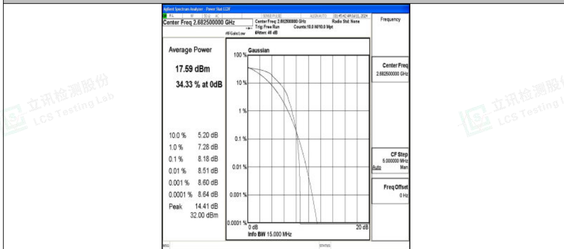
Band41-15MHz-QPSK-41515-1RB#0-PASS
