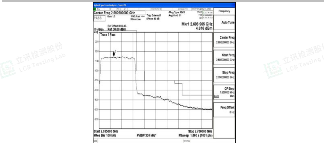
Band41_5MHz_16QAM_41565_25RB#0
