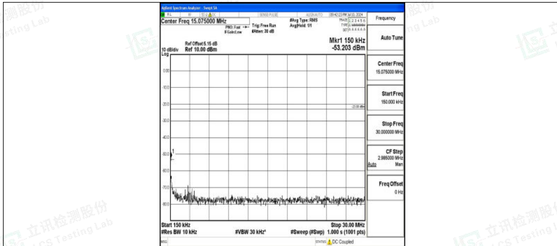
Band26_10MHz_QPSK_26740_1RB#0_0.15~30_0.15~30
