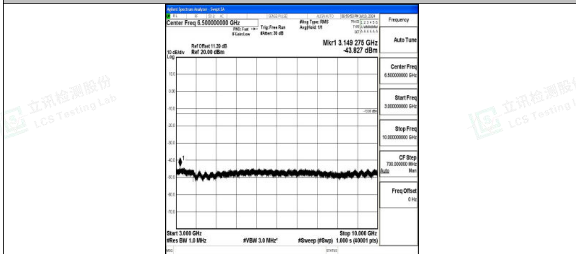
Band26_3MHz_QPSK_26775_1RB#0_3000~10000_3000~10000
