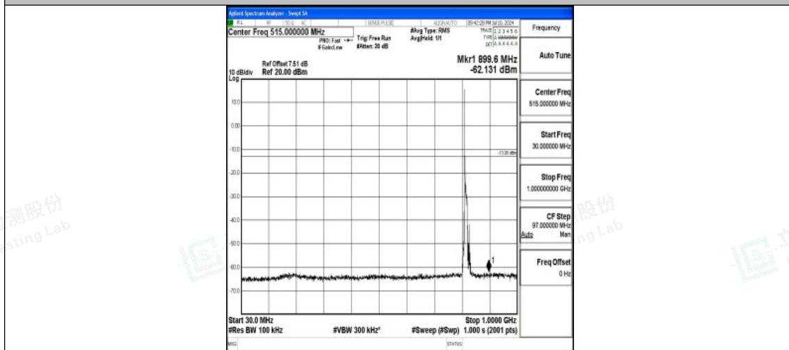
Band26_10MHz_QPSK_26740_1RB#0_30~1000_30~1000
