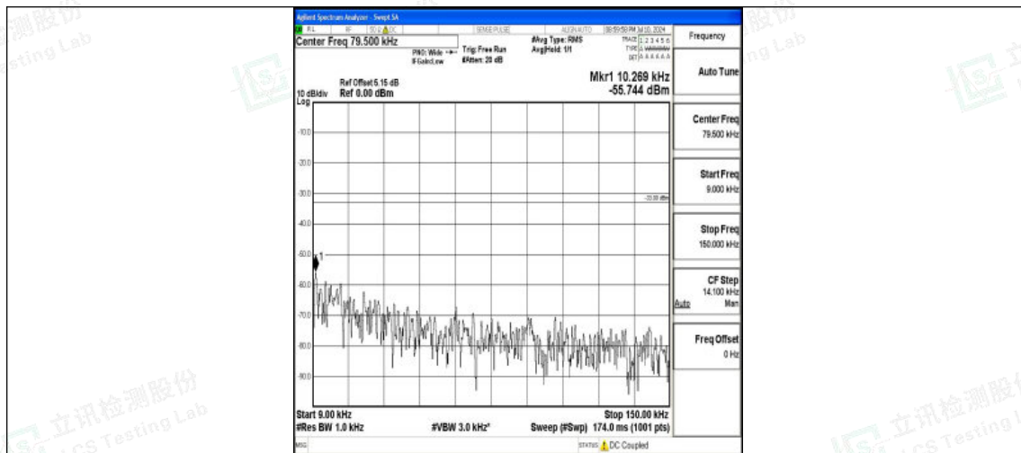
Band26_3MHz_16QAM_26775_1RB#0_0.009~0.15_0.009~0.15
