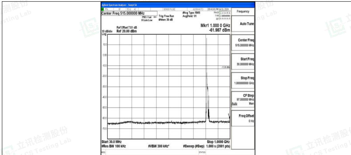
Band26_10MHz_16QAM_26740_1RB#0_30~1000_30~1000
