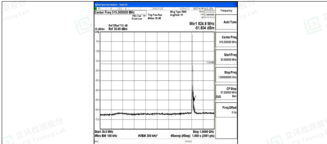
Band26_3MHz_16QAM_26705_1RB#0_30~1000_30~1000
