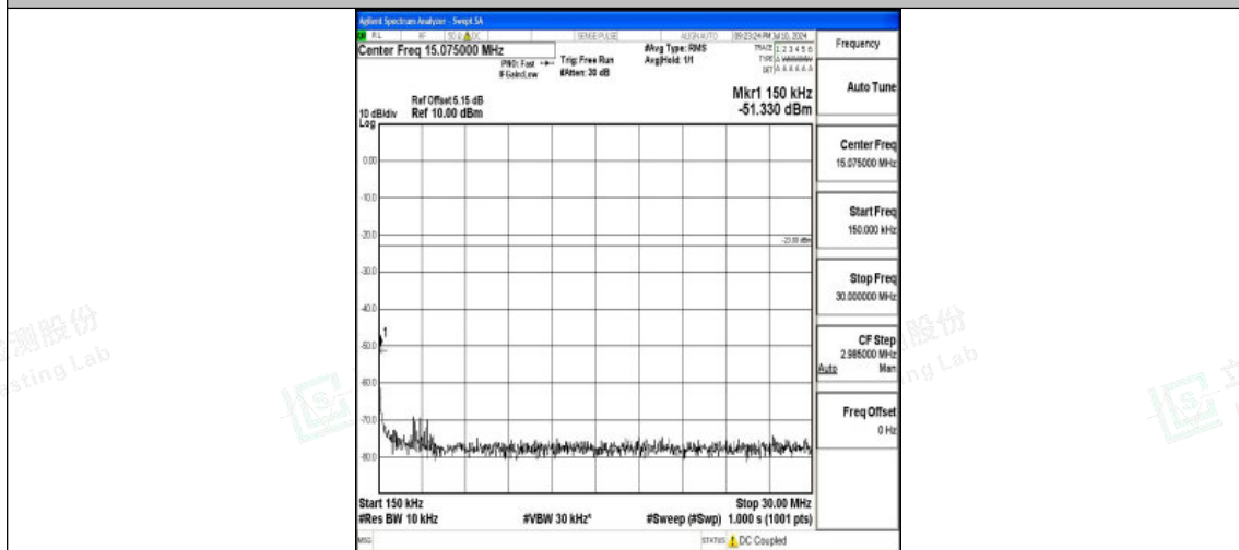
Band26_5MHz_QPSK_26740_1RB#0_0.15~30_0.15~30
