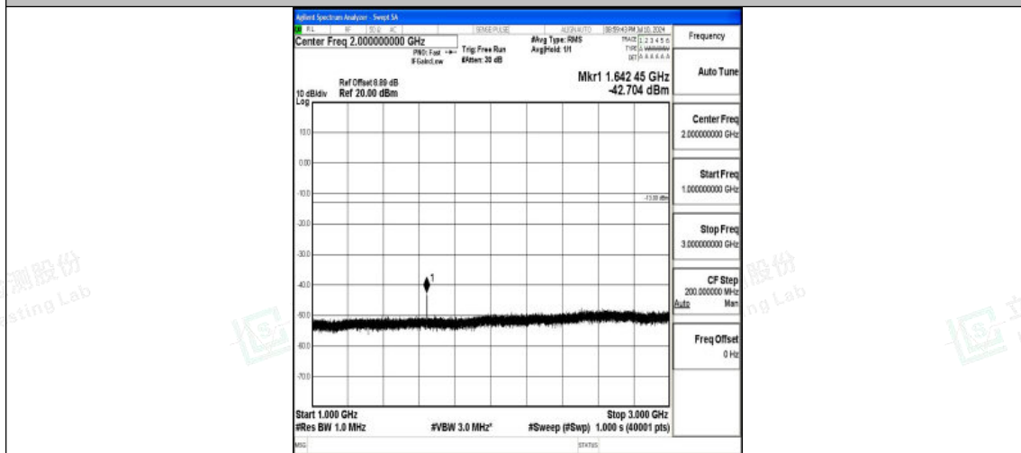
Band26_3MHz_QPSK_26775_1RB#0_1000~3000_1000~3000
