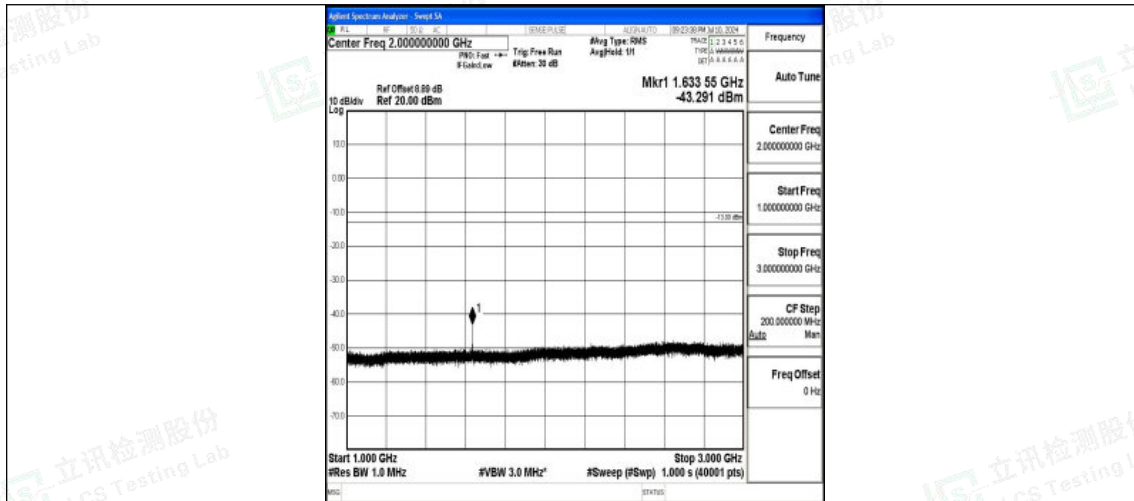
Band26_5MHz_QPSK_26740_1RB#0_1000~3000_1000~3000
