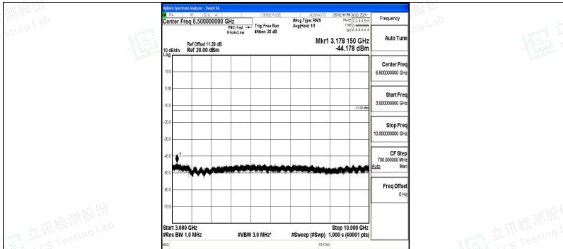
Band26_10MHz_QPSK_26740_1RB#0_3000~10000_3000~10000
