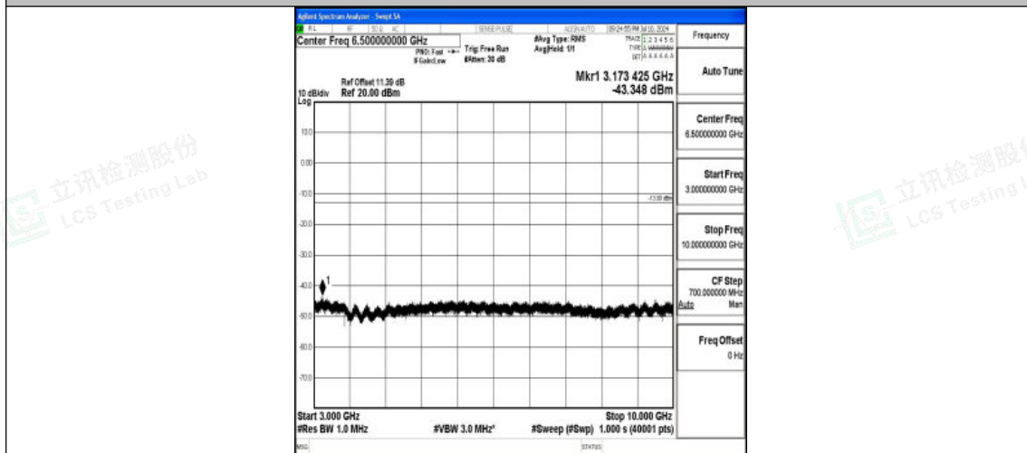
Band26_5MHz_QPSK_26765_1RB#0_3000~10000_3000~10000
