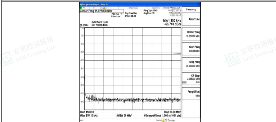
Band26_10MHz_16QAM_26740_1RB#0_0.15~30_0.15~30
