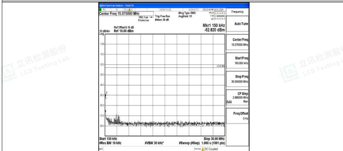
Band26_5MHz_16QAM_26715_1RB#0_0.15~30_0.15~30
