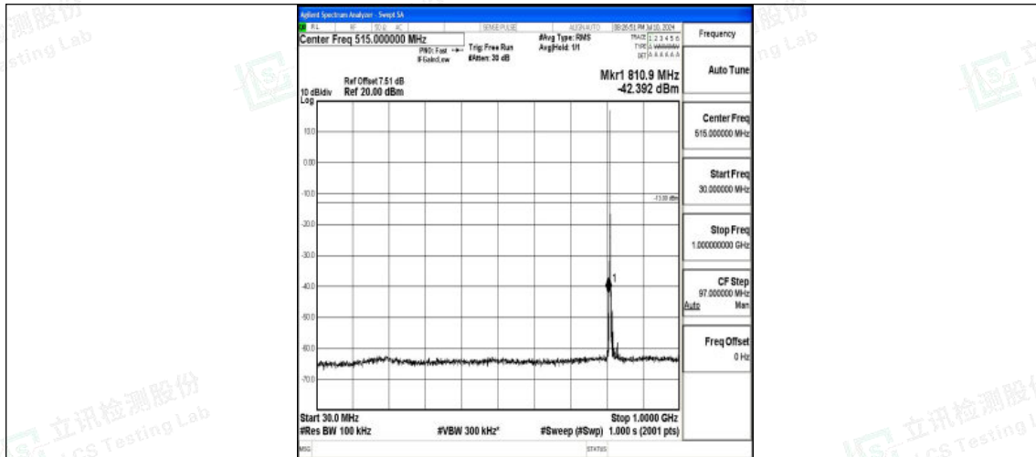
Band26_1.4MHz_16QAM_26697_1RB#0_30~1000_30~1000
