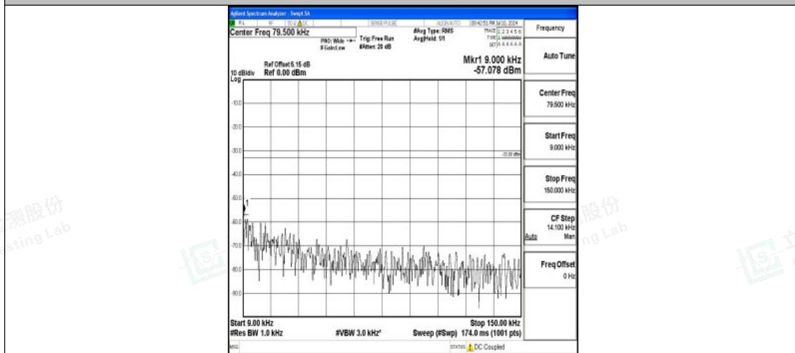
Band26_10MHz_16QAM_26740_1RB#0_0.009~0.15_0.009~0.15
