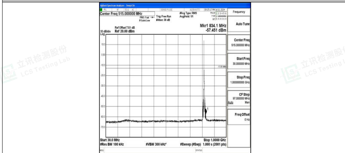
Band26_5MHz_16QAM_26765_1RB#0_30~1000_30~1000
