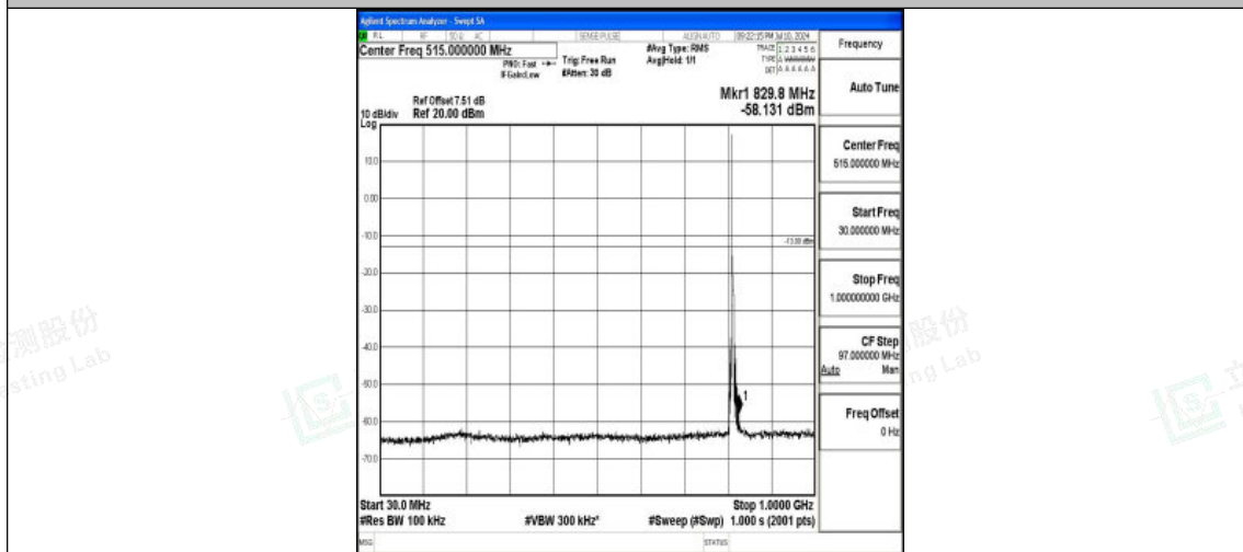
Band26_5MHz_QPSK_26715_1RB#0_30~1000_30~1000
