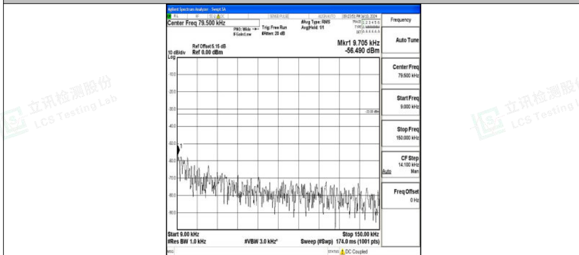
Band26_5MHz_16QAM_26740_1RB#0_0.009~0.15_0.009~0.15
