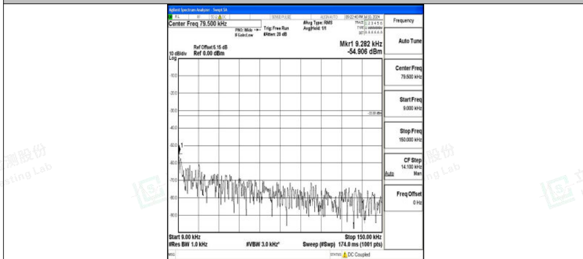
Band26_5MHz_16QAM_26715_1RB#0_0.009~0.15_0.009~0.15
