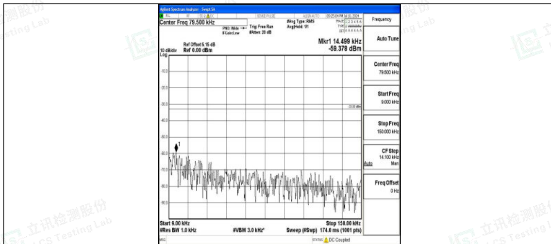
Band26_5MHz_16QAM_26765_1RB#0_0.009~0.15_0.009~0.15
