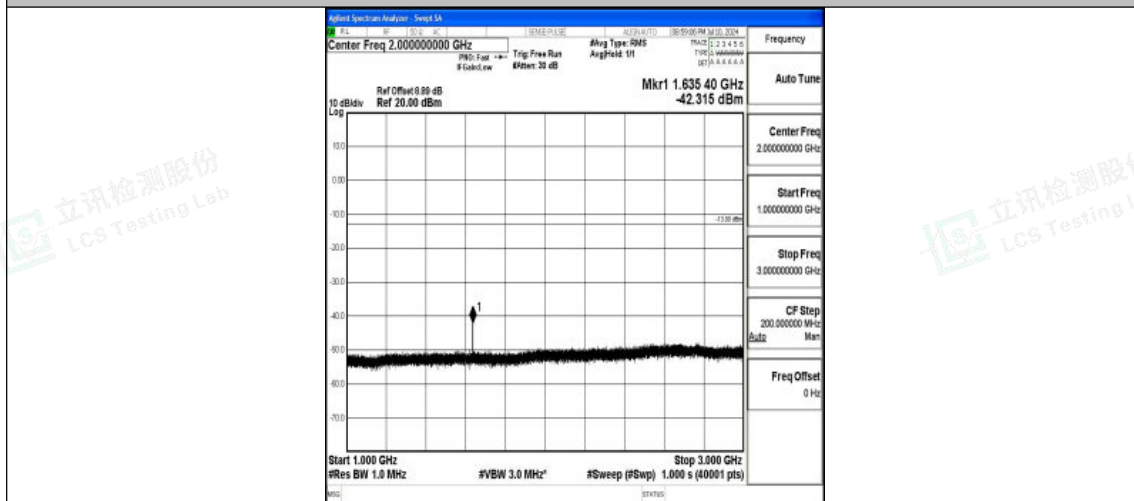
Band26_3MHz_16QAM_26740_1RB#0_1000~3000_1000~3000
