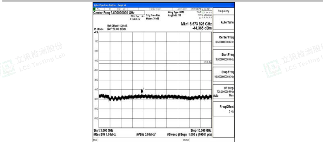
Band26_5MHz_16QAM_26715_1RB#0_3000~10000_3000~10000
