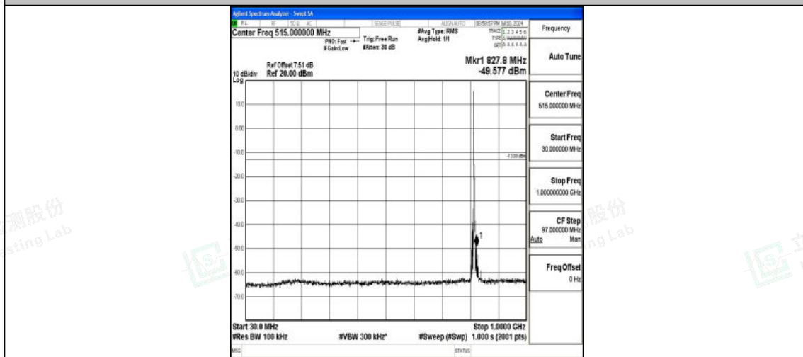
Band26_3MHz_16QAM_26740_1RB#0_30~1000_30~1000
