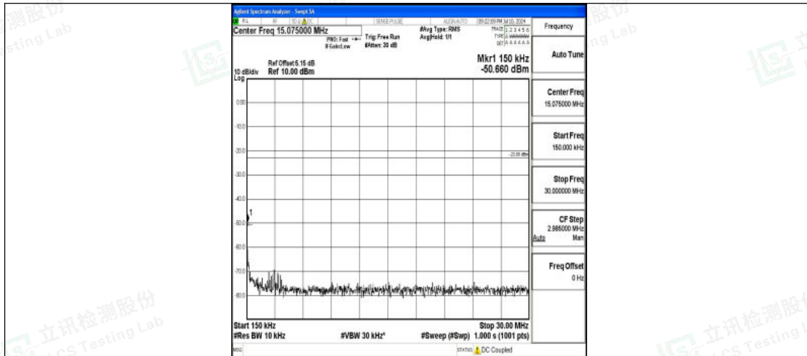
Band26_5MHz_QPSK_26715_1RB#0_0.15~30_0.15~30
