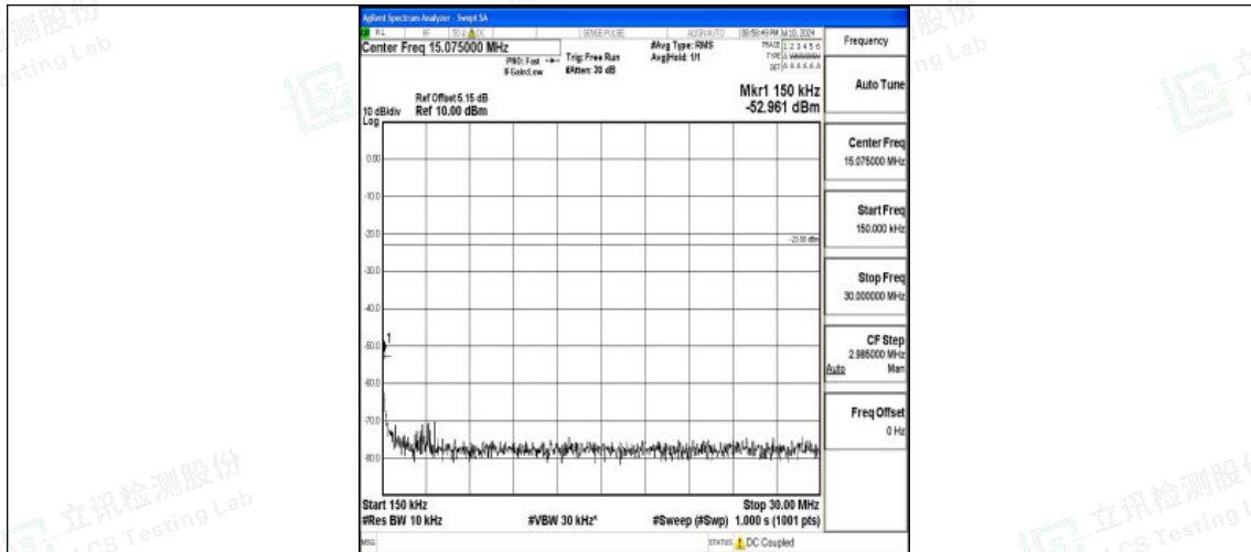
Band26_3MHz_16QAM_26740_1RB#0_0.15~30_0.15~30
