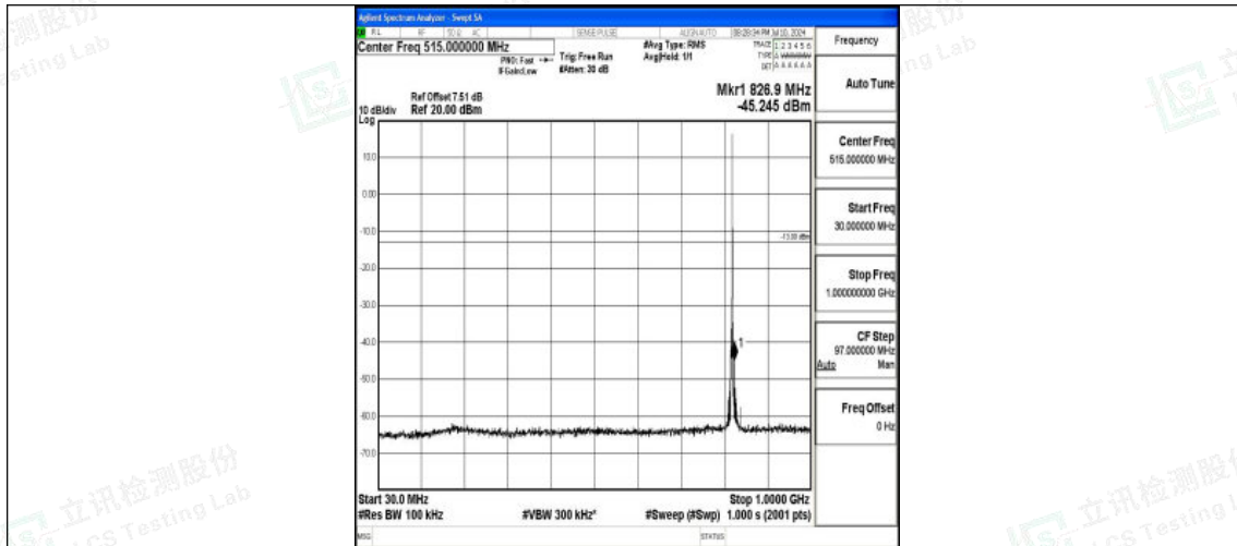
Band26_1.4MHz_QPSK_26783_1RB#0_30~1000_30~1000
