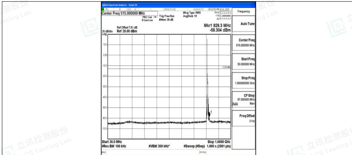
Band26_5MHz_16QAM_26715_1RB#0_30~1000_30~1000
