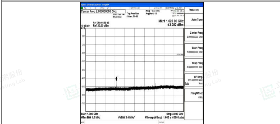
Band26_5MHz_16QAM_26715_1RB#0_1000~3000_1000~3000
