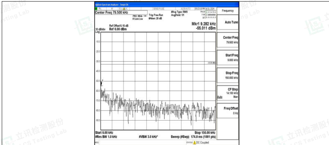
Band26_5MHz_QPSK_26740_1RB#0_0.009~0.15_0.009~0.15
