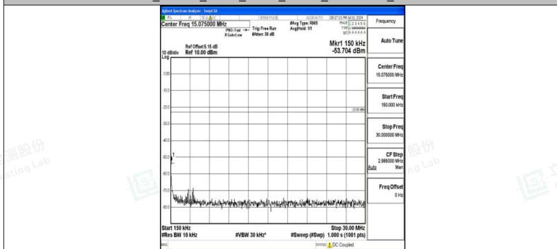
Band26_1.4MHz_QPSK_26740_1RB#0_0.15~30_0.15~30
