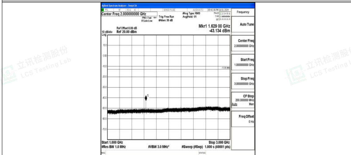
Band26_10MHz_QPSK_26740_1RB#0_1000~3000_1000~3000
