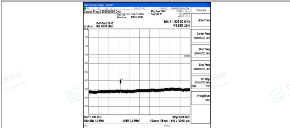
Band26_10MHz_16QAM_26740_1RB#0_1000~3000_1000~3000
