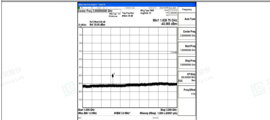
Band26_5MHz_QPSK_26765_1RB#0_1000~3000_1000~3000
