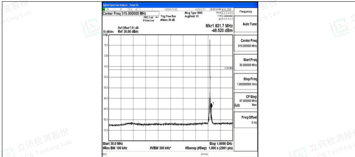
Band26_3MHz_QPSK_26775_1RB#0_30~1000_30~1000
