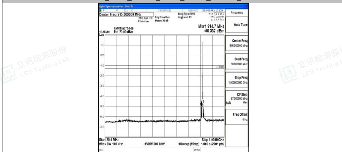
Band26_3MHz_16QAM_26775_1RB#0_30~1000_30~1000
