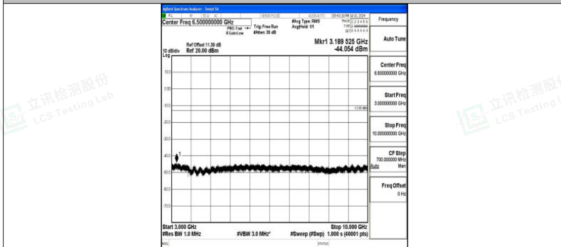
Band26_10MHz_16QAM_26740_1RB#0_3000~10000_3000~10000
