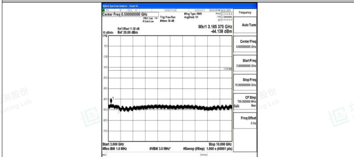
Band26_5MHz_QPSK_26740_1RB#0_3000~10000_3000~10000
