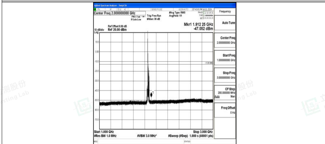
Band25_15MHz_16QAM_26115_1RB#0_1000~3000_1000~3000
