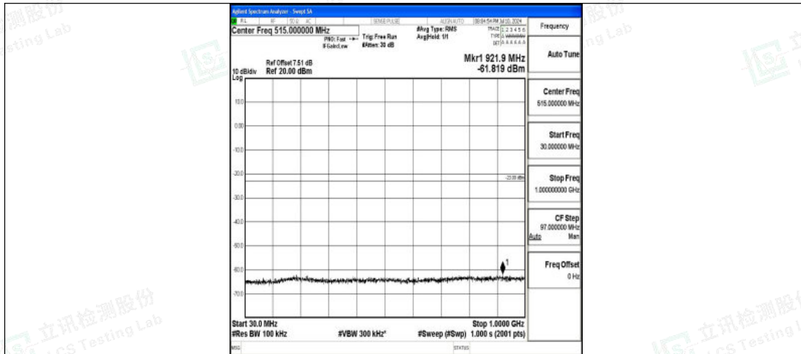
Band25_20MHz_16QAM_26140_1RB#0_30~1000_30~1000
