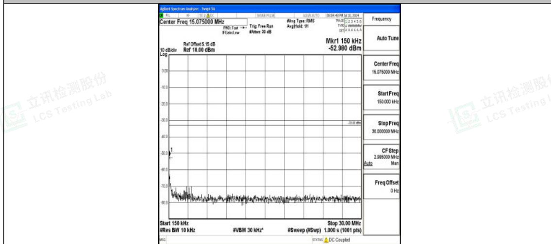
Band25_20MHz_16QAM_26140_1RB#0_0.15~30_0.15~30
