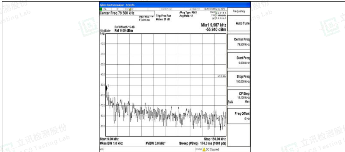
Band25_5MHz_16QAM_26665_1RB#0_0.009~0.15_0.009~0.15
