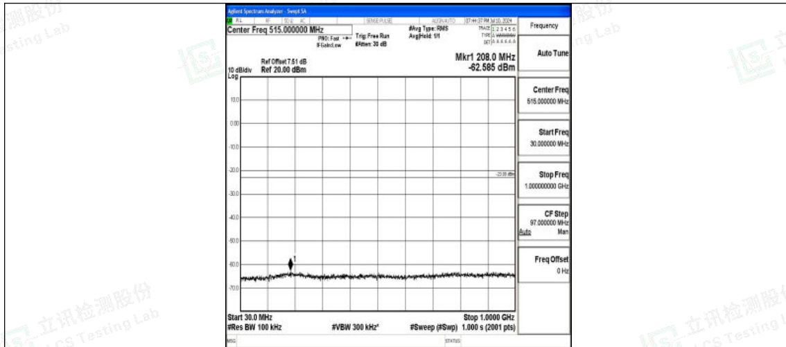
Band25_15MHz_QPSK_26615_1RB#0_30~1000_30~1000
