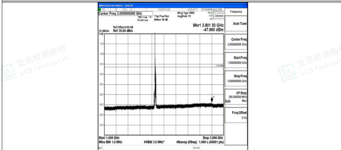
Band25_10MHz_QPSK_26090_1RB#0_1000~3000_1000~3000
