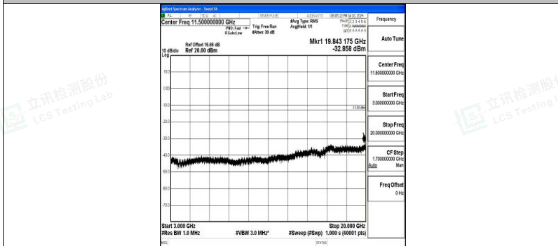
Band25_20MHz_16QAM_26140_1RB#0_3000~20000_3000~20000
