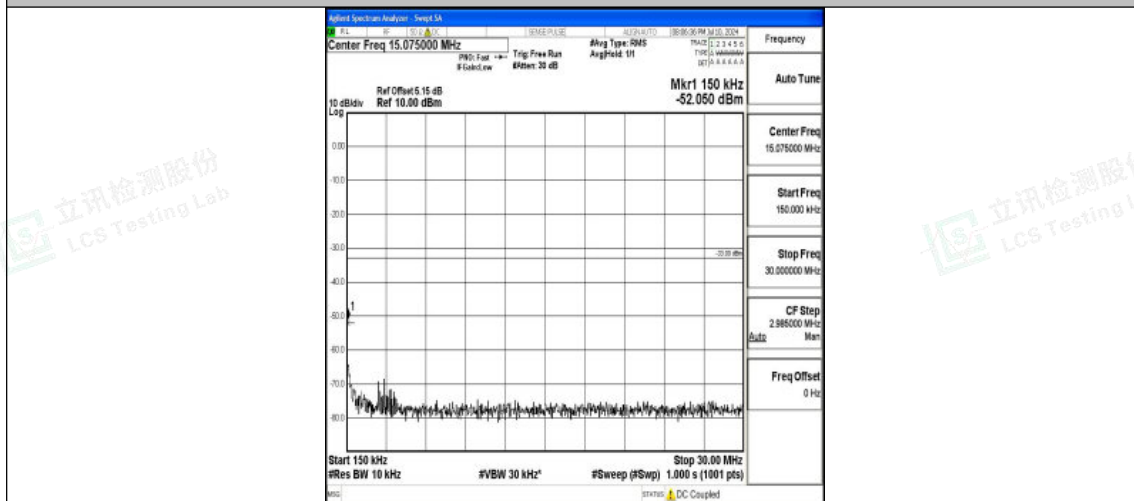
Band25_20MHz_QPSK_26590_1RB#0_0.15~30_0.15~30
