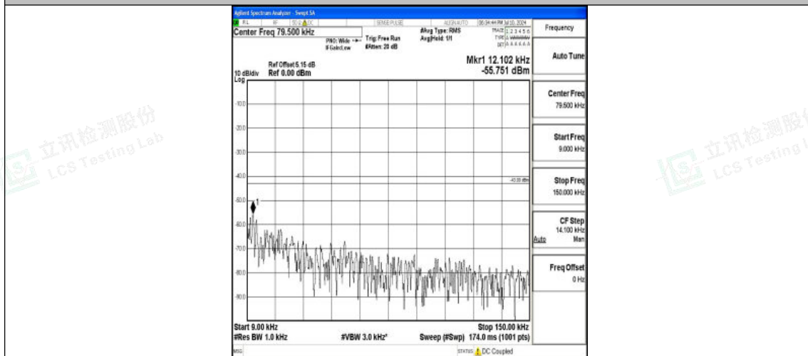
Band25_3MHz_16QAM_26365_1RB#0_0.009~0.15_0.009~0.15
