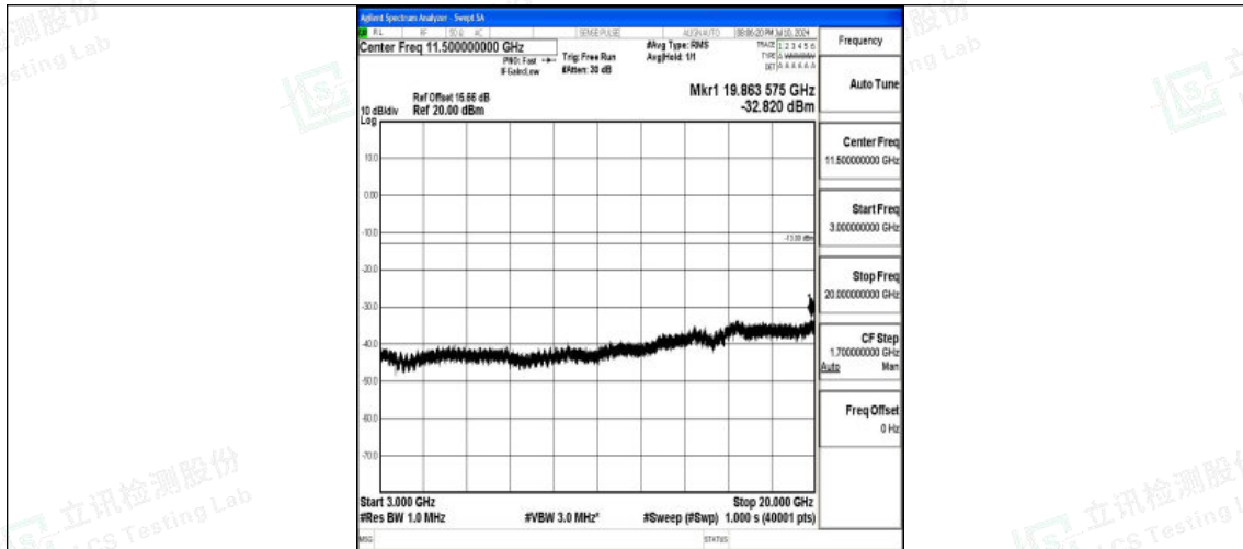
Band25_20MHz_16QAM_26365_1RB#0_3000~20000_3000~20000
