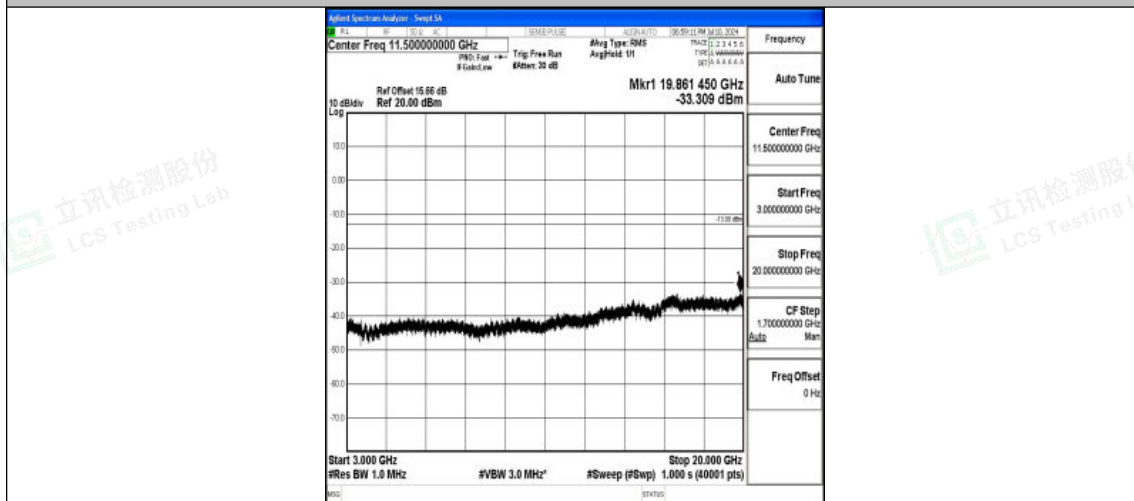
Band25_5MHz_QPSK_26665_1RB#0_3000~20000_3000~20000
