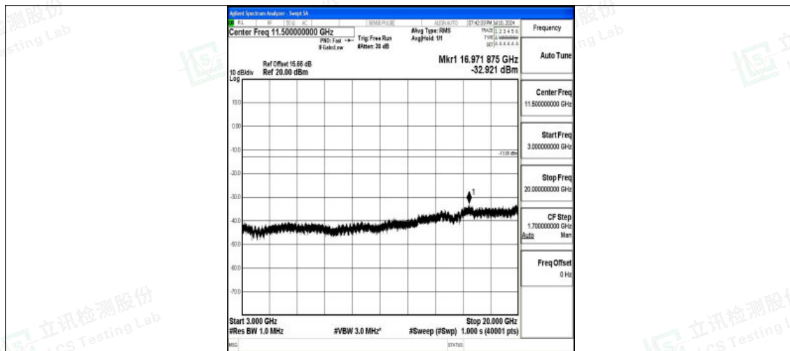
Band25_15MHz_QPSK_26115_1RB#0_3000~20000_3000~20000
