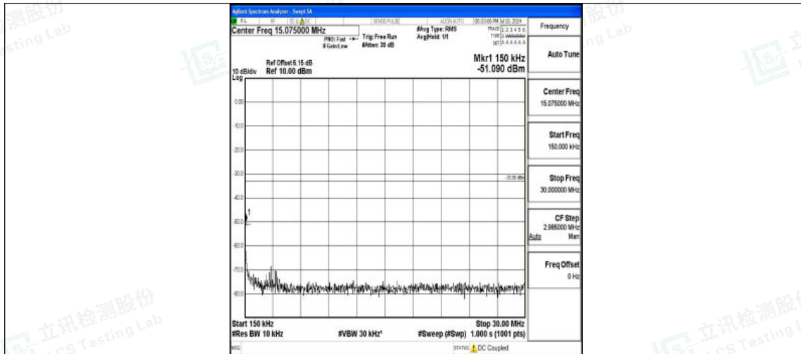
Band25_3MHz_QPSK_26055_1RB#0_0.15~30_0.15~30
