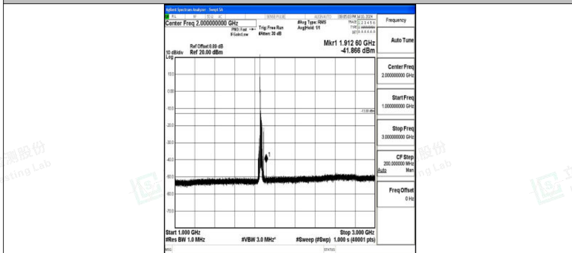
Band25_20MHz_16QAM_26140_1RB#0_1000~3000_1000~3000
