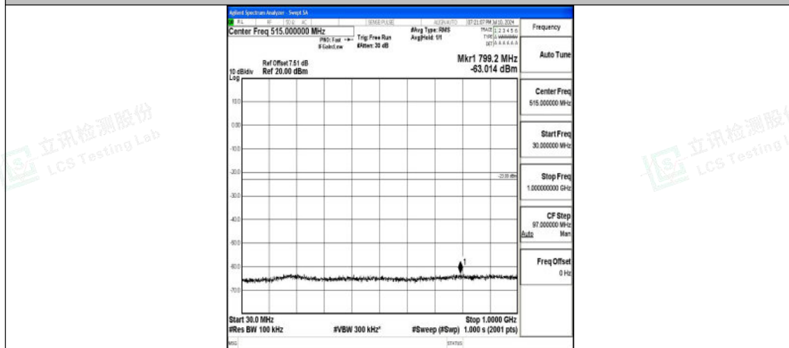
Band25_10MHz_QPSK_26365_1RB#0_30~1000_30~1000
