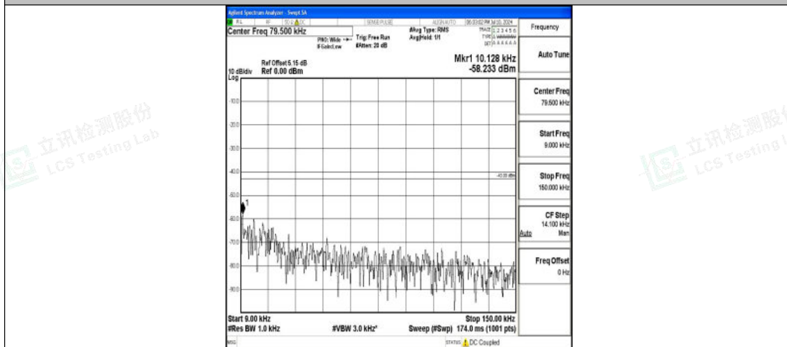
Band25_3MHz_QPSK_26055_1RB#0_0.009~0.15_0.009~0.15
