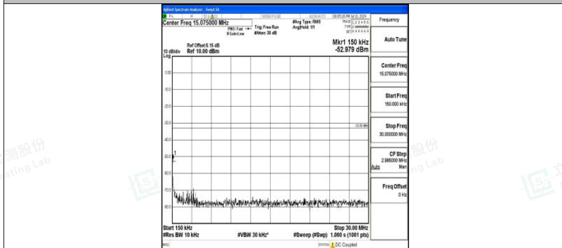
Band25_20MHz_QPSK_26365_1RB#0_0.15~30_0.15~30
