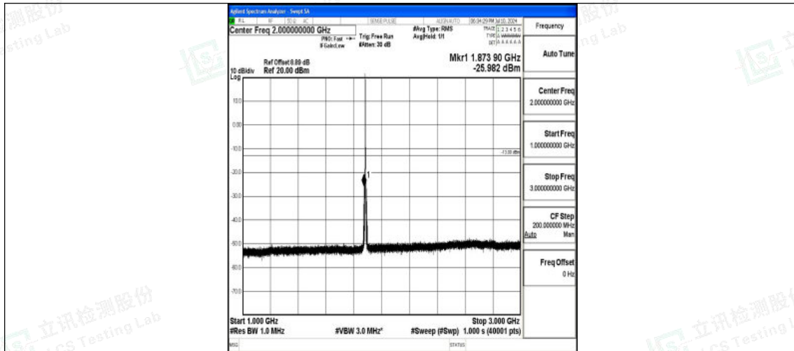
Band25_3MHz_QPSK_26365_1RB#0_1000~3000_1000~3000
