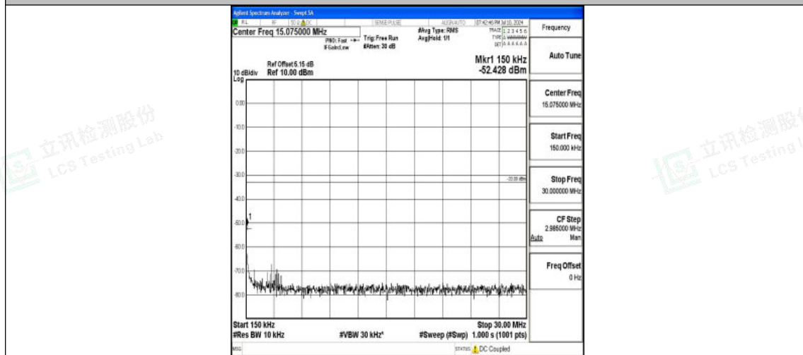
Band25_15MHz_16QAM_26115_1RB#0_0.15~30_0.15~30
