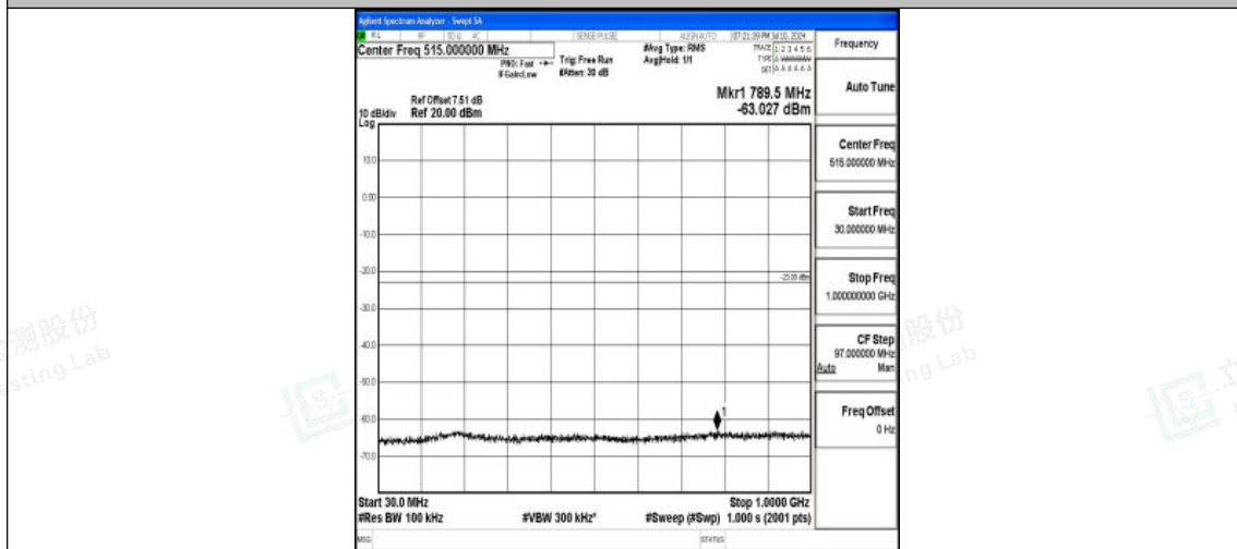
Band25_10MHz_16QAM_26365_1RB#0_30~1000_30~1000
