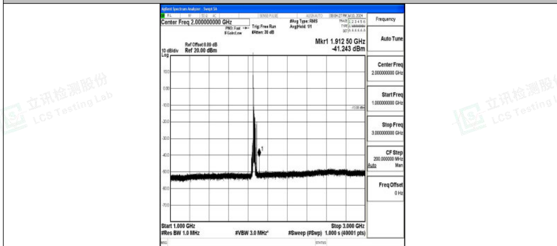
Band25_20MHz_QPSK_26140_1RB#0_1000~3000_1000~3000
