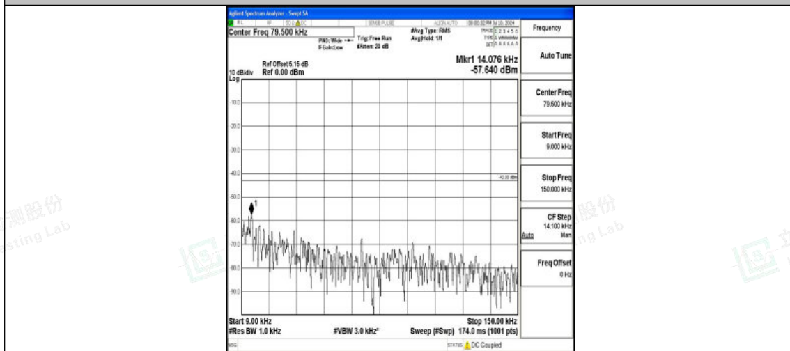
Band25_20MHz_QPSK_26590_1RB#0_0.009~0.15_0.009~0.15
