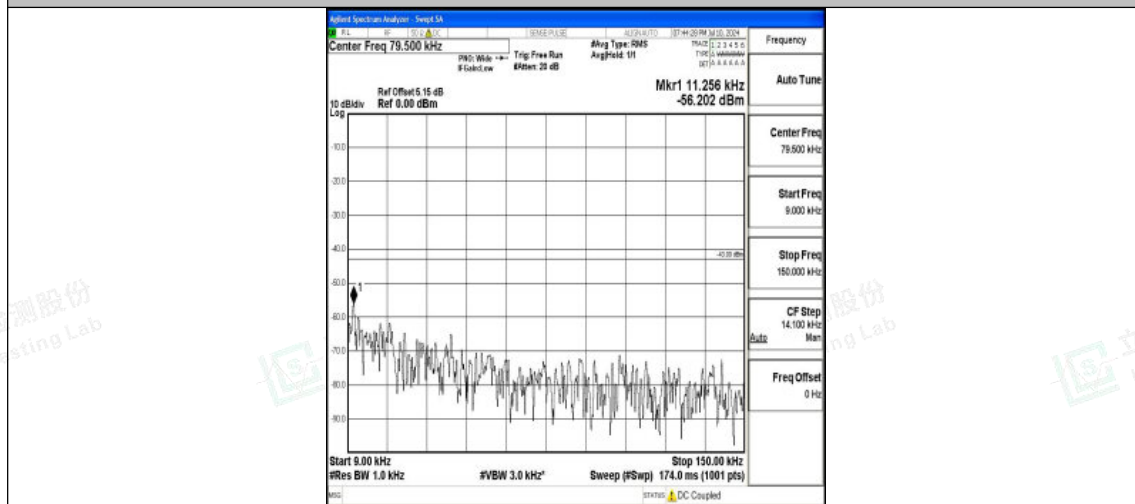
Band25_15MHz_QPSK_26615_1RB#0_0.009~0.15_0.009~0.15
