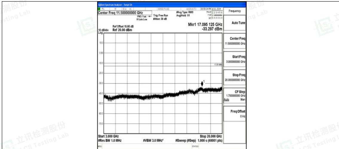
Band25_5MHz_16QAM_26365_1RB#0_3000~20000_3000~20000
