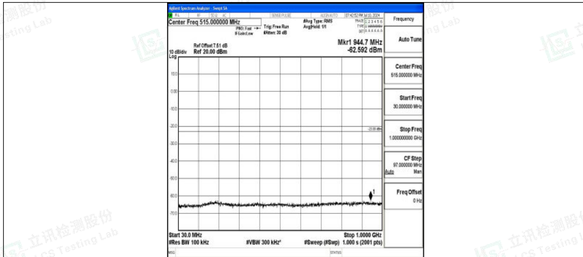
Band25_15MHz_16QAM_26115_1RB#0_30~1000_30~1000
