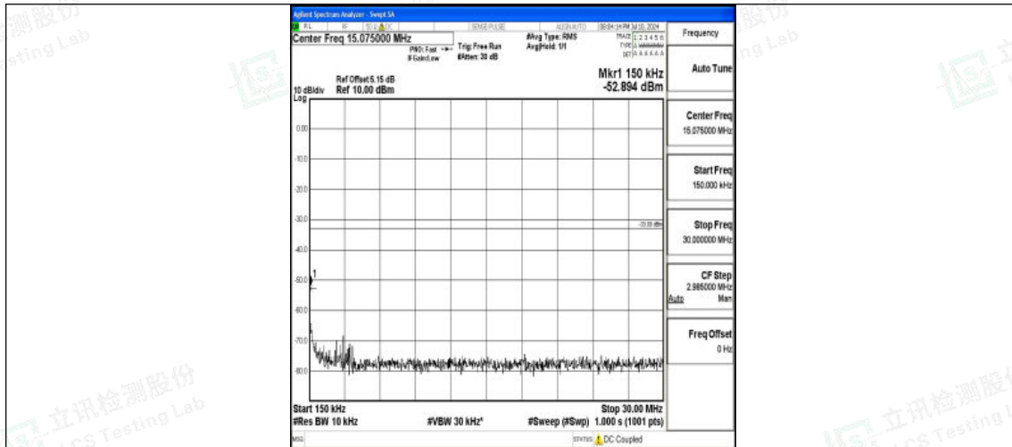
Band25_20MHz_QPSK_26140_1RB#0_0.15~30_0.15~30
