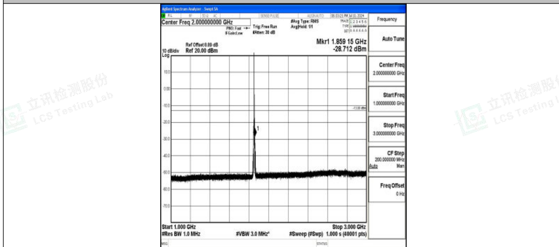
Band25_3MHz_QPSK_26055_1RB#0_1000~3000_1000~3000
