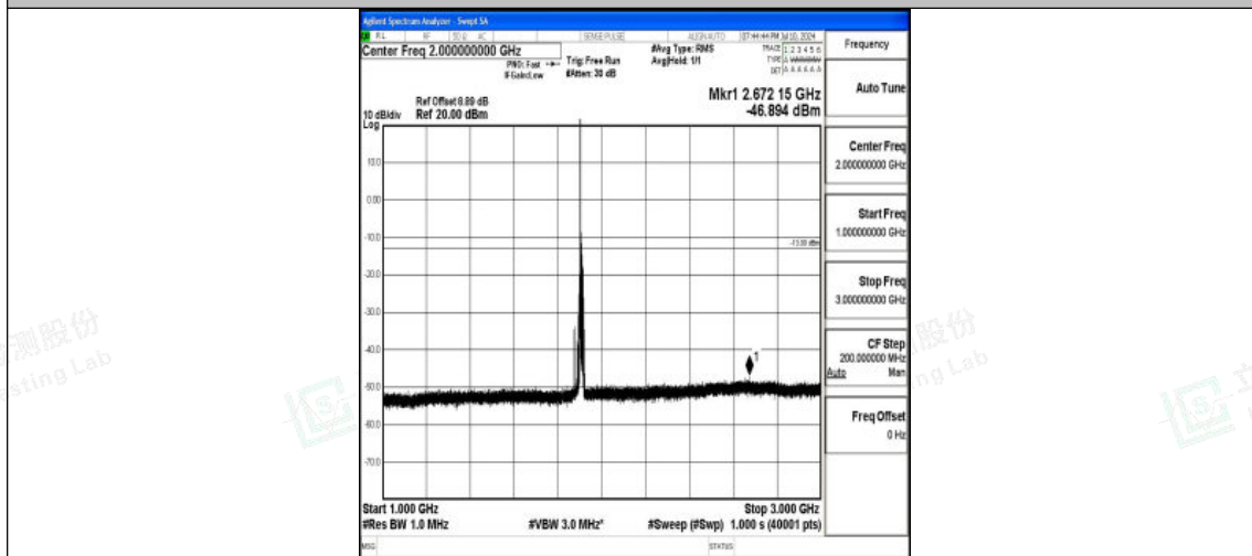
Band25_15MHz_QPSK_26615_1RB#0_1000~3000_1000~3000
