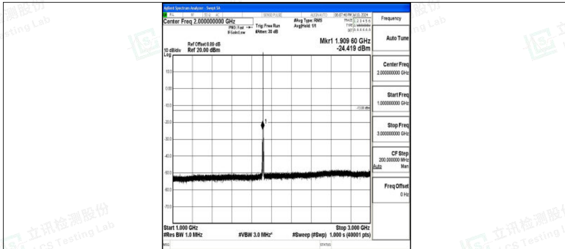
Band25_1.4MHz_16QAM_26683_1RB#0_1000~3000_1000~3000
