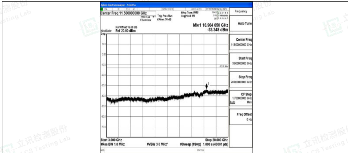
Band25_10MHz_16QAM_26365_1RB#0_3000~20000_3000~20000
