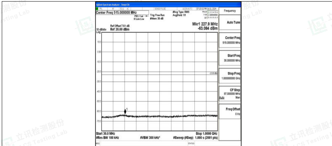
Band25_10MHz_16QAM_26090_1RB#0_30~1000_30~1000
