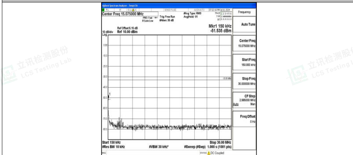
Band25_10MHz_QPSK_26640_1RB#0_0.15~30_0.15~30
