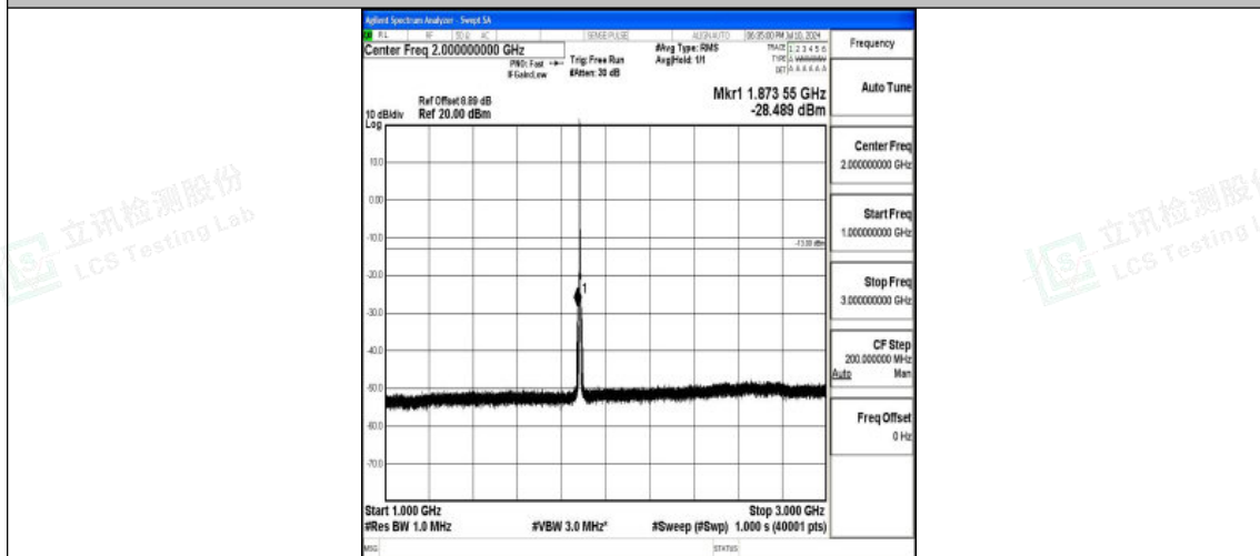
Band25_3MHz_16QAM_26365_1RB#0_1000~3000_1000~3000
