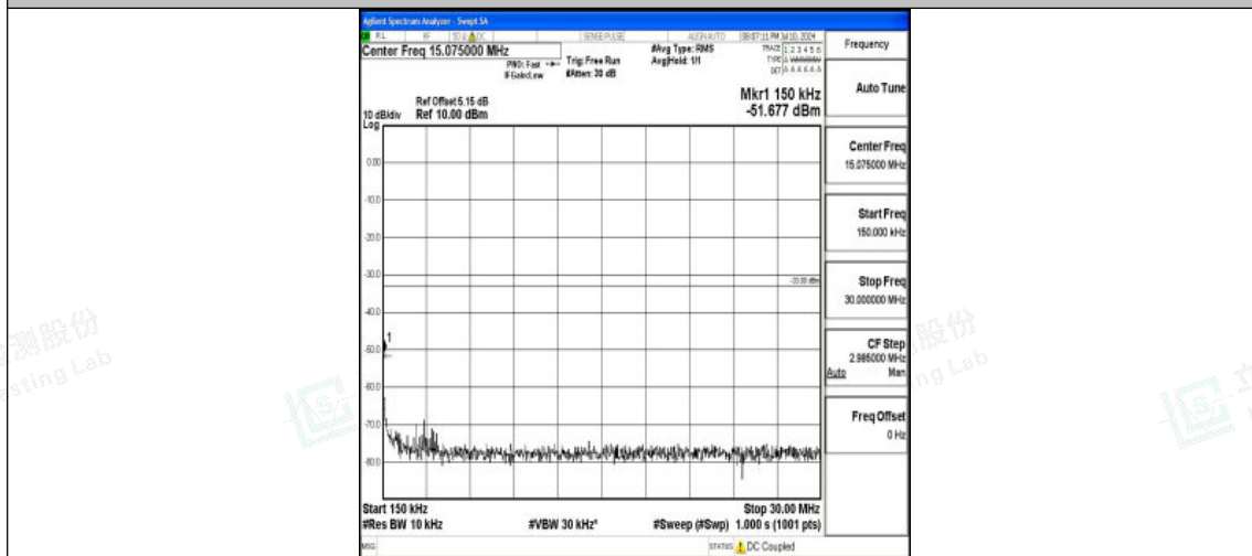
Band25_20MHz_16QAM_26590_1RB#0_0.15~30_0.15~30
