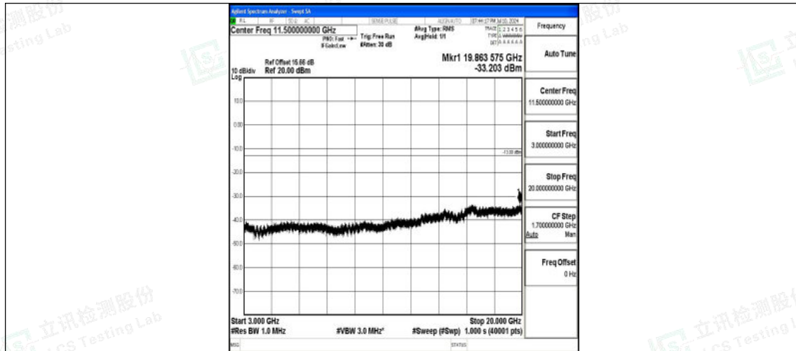
Band25_15MHz_16QAM_26365_1RB#0_3000~20000_3000~20000
