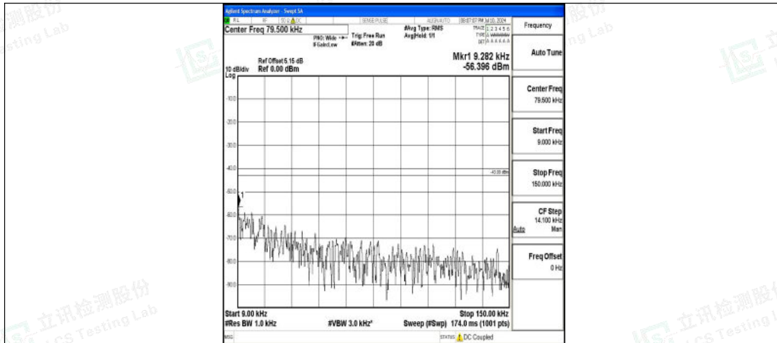
Band25_20MHz_16QAM_26590_1RB#0_0.009~0.15_0.009~0.15
