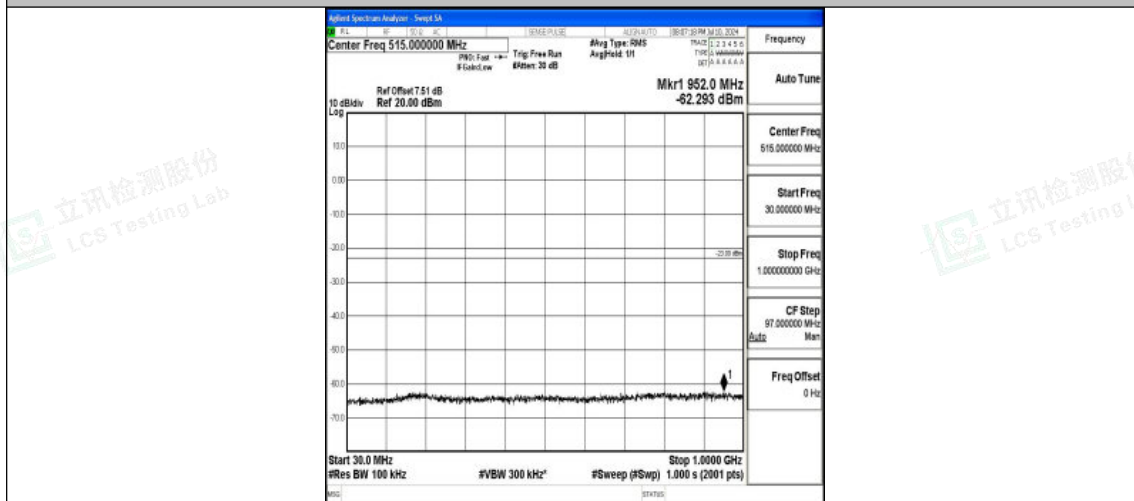
Band25_20MHz_16QAM_26590_1RB#0_30~1000_30~1000
