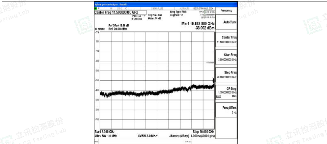
Band25_3MHz_16QAM_26365_1RB#0_3000~20000_3000~20000
