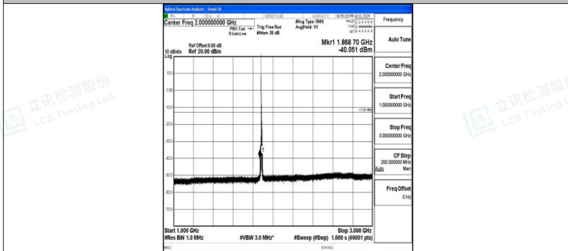
Band25_5MHz_16QAM_26365_1RB#0_1000~3000_1000~3000
