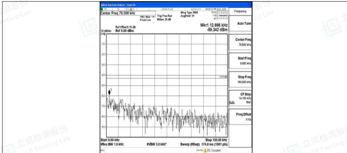
Band25_20MHz_QPSK_26365_1RB#0_0.009~0.15_0.009~0.15
