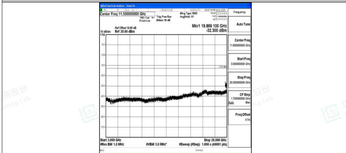
Band25_20MHz_16QAM_26590_1RB#0_3000~20000_3000~20000
