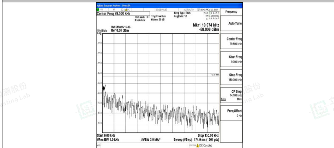
Band25_15MHz_16QAM_26115_1RB#0_0.009~0.15_0.009~0.15
