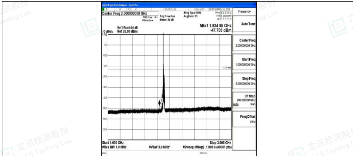
Band25_20MHz_16QAM_26590_1RB#0_1000~3000_1000~3000
