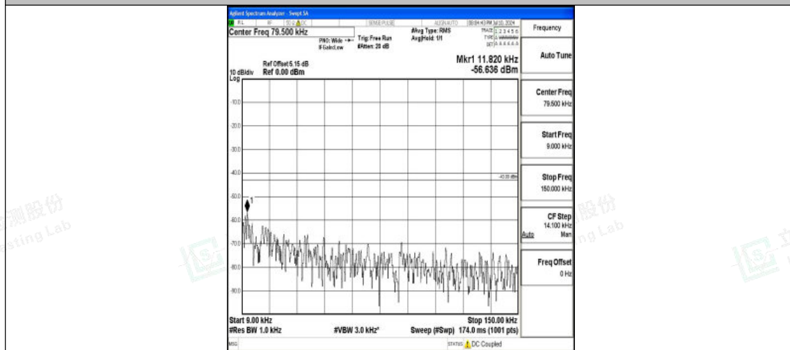
Band25_20MHz_16QAM_26140_1RB#0_0.009~0.15_0.009~0.15
