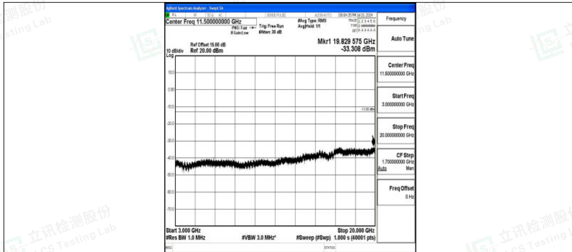
Band25_20MHz_QPSK_26140_1RB#0_3000~20000_3000~20000
