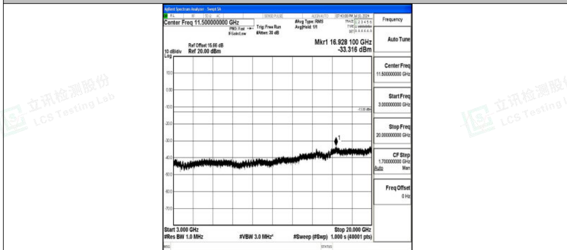
Band25_15MHz_16QAM_26115_1RB#0_3000~20000_3000~20000
