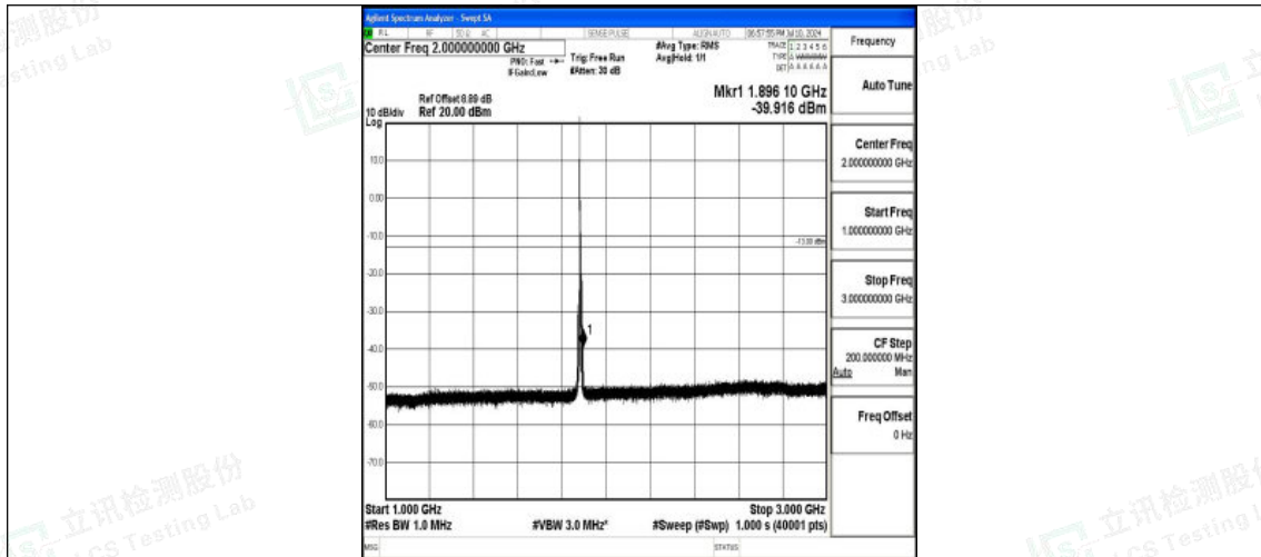
Band25_5MHz_QPSK_26365_1RB#0_1000~3000_1000~3000
