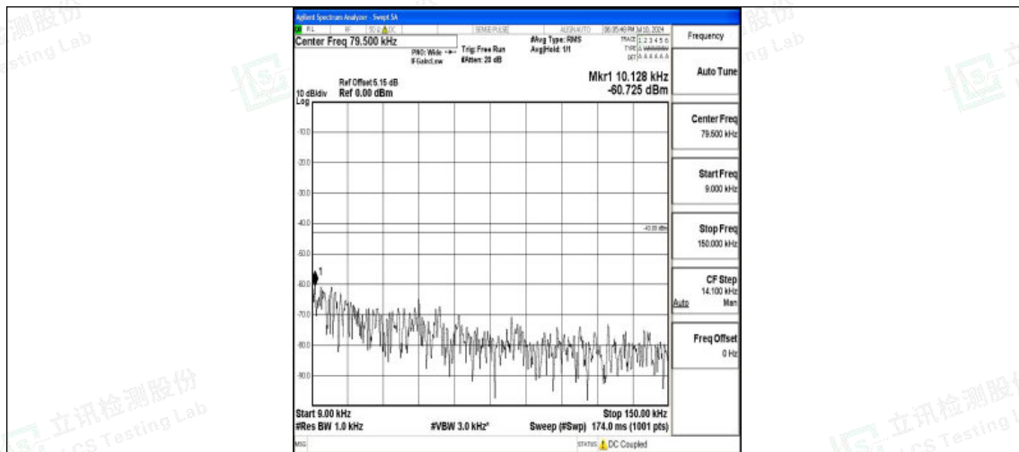
Band25_3MHz_16QAM_26675_1RB#0_0.009~0.15_0.009~0.15
