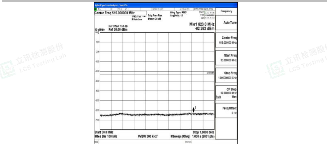
Band25_5MHz_16QAM_26665_1RB#0_30~1000_30~1000
