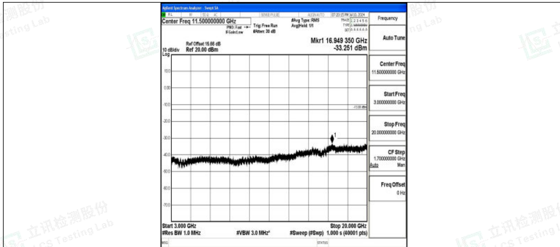
Band25_10MHz_QPSK_26090_1RB#0_3000~20000_3000~20000
