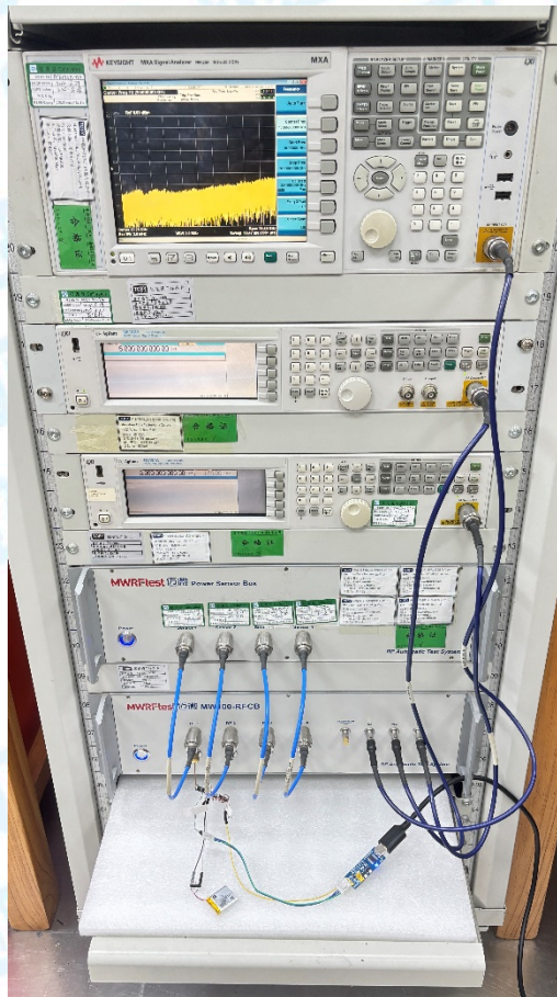
Photo of Setup for Conducted Measurement
