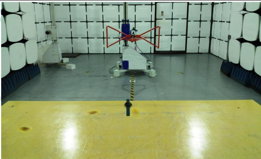
Emissions in frequency bands (below 1GHz)
