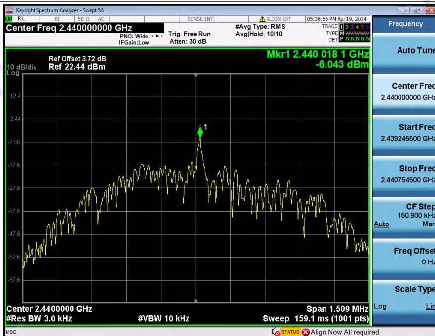
Power_Spectral_Density_NVNT_ANT1_1Mbps_2440
