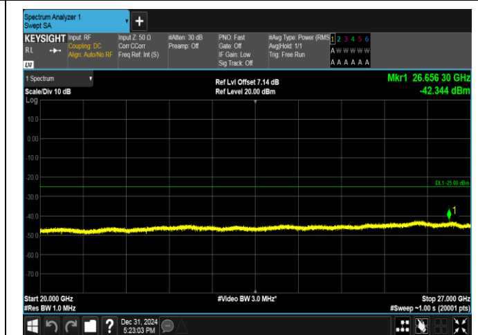
Band38-5MHz-QPSK-38000-1RB#0-20000~27000-PASS
