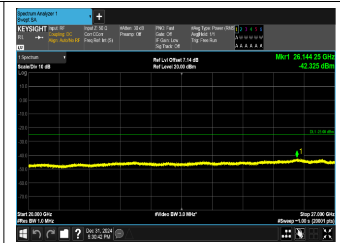
Band38-5MHz-QPSK-38225-1RB#24-20000~27000-PASS
