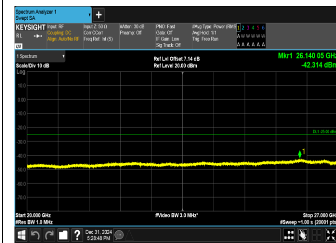
Band38-5MHz-QPSK-38225-1RB#0-20000~27000-PASS
