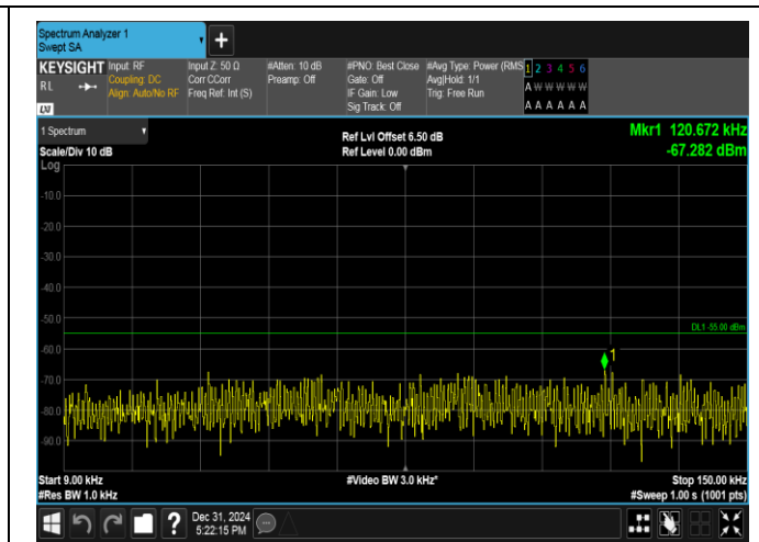
Band38-5MHz-QPSK-38000-1RB#0-0.009~0.15-PASS
