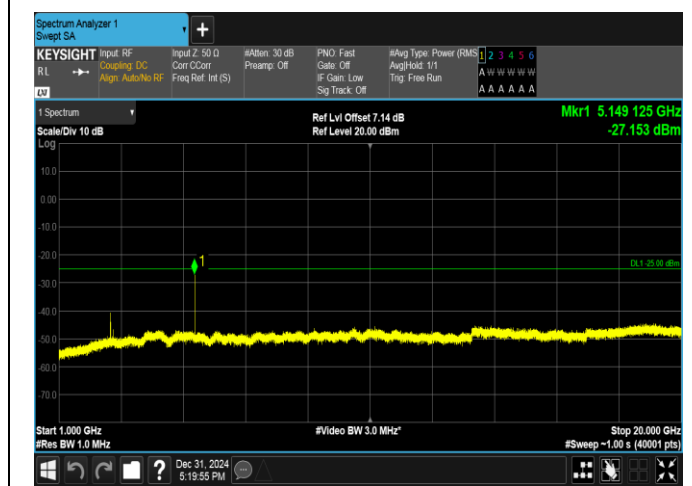
Band38-5MHz-16QAM-37775-1RB#24-1000~20000-PASS
