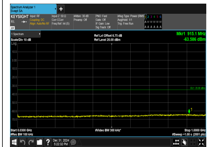
Band38-5MHz-QPSK-38000-1RB#0-30~1000-PASS
