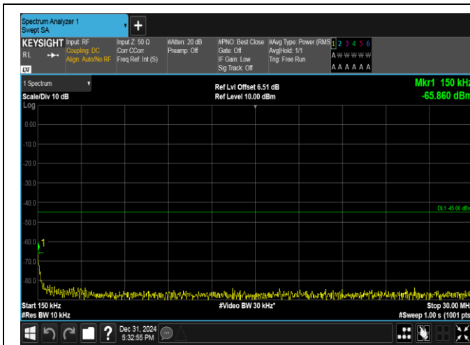
Band38-5MHz-16QAM-38225-25RB#0-0.15~30-PASS
