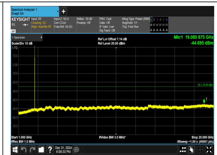
Band38-10MHz-QPSK-37800-1RB#0-1000~20000-PASS
