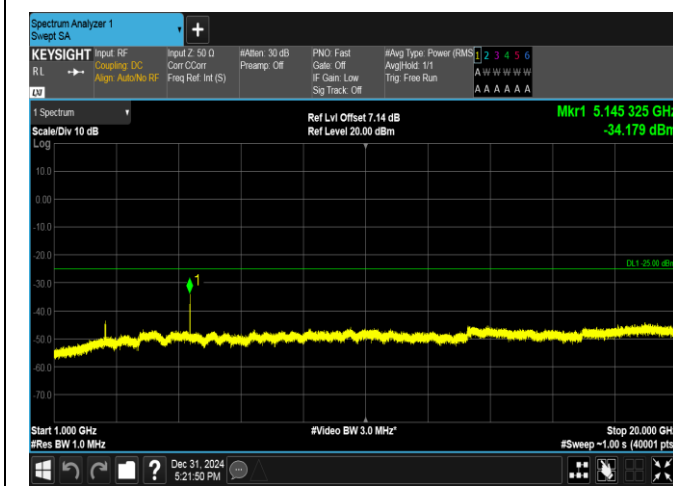
Band38-5MHz-16QAM-37775-25RB#0-1000~20000-PASS
