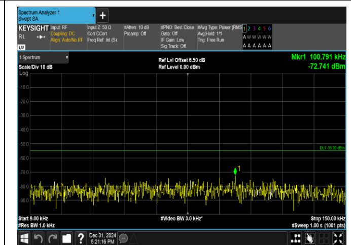
Band38-5MHz-16QAM-37775-25RB#0-0.009~0.15-PASS
