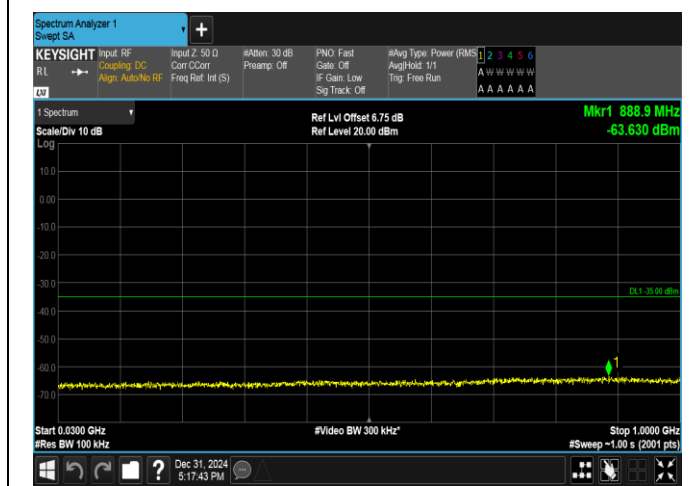
Band38-5MHz-16QAM-37775-1RB#0-30~1000-PASS
