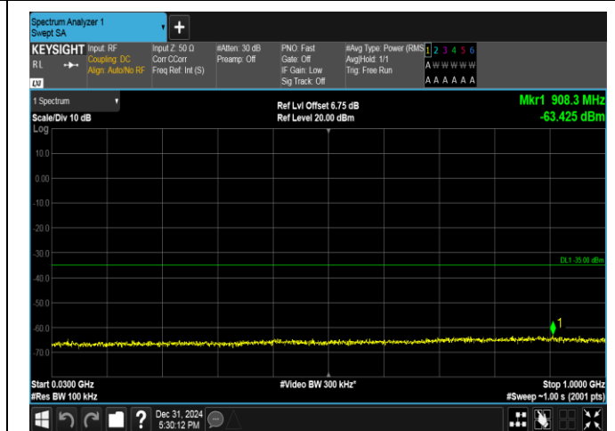
Band38-5MHz-QPSK-38225-1RB#24-30~1000-PASS
