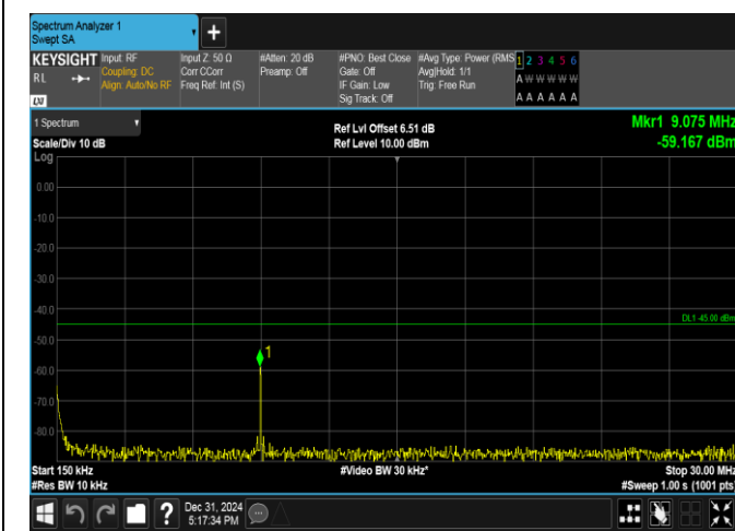
Band38-5MHz-16QAM-37775-1RB#0-0.15~30-PASS
