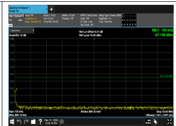
Band38-5MHz-QPSK-38000-1RB#24-0.15~30-PASS
