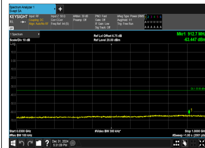
Band38-5MHz-16QAM-38225-1RB#24-30~1000-PASS
