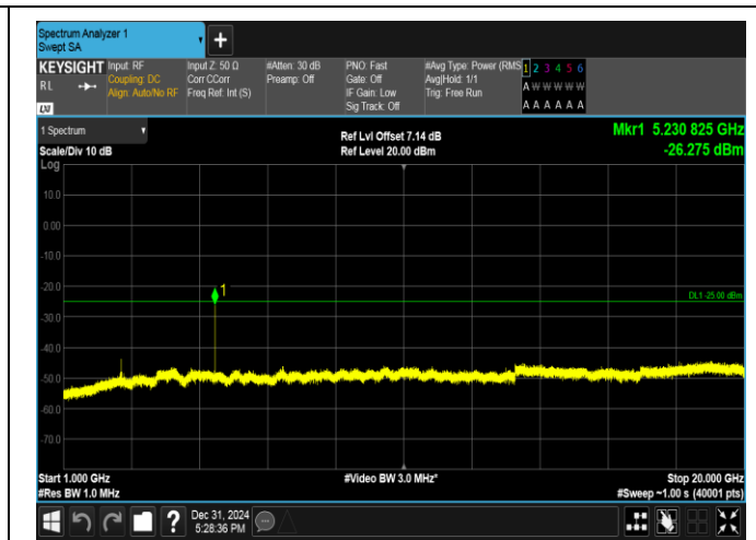
Band38-5MHz-QPSK-38225-1RB#0-1000~20000-PASS
