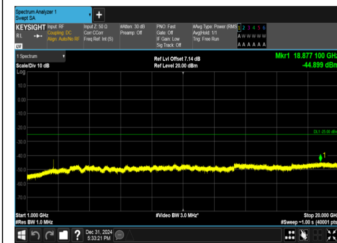
Band38-5MHz-16QAM-38225-25RB#0-1000~20000-PASS
