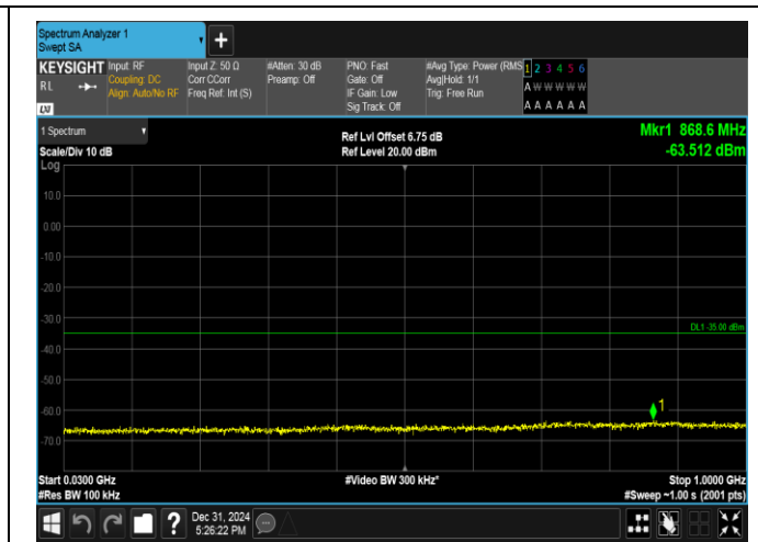
Band38-5MHz-QPSK-38000-25RB#0-30~1000-PASS
