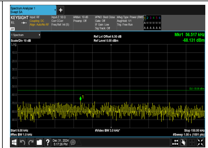
Band38-5MHz-16QAM-37775-1RB#0-0.009~0.15-PASS
