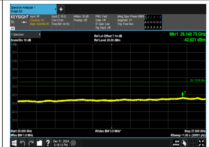
Band38-5MHz-16QAM-37775-1RB#0-20000~27000-PASS
