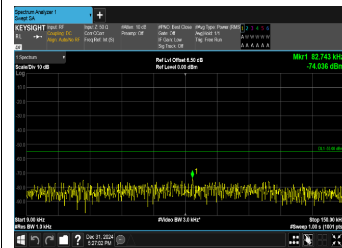
Band38-5MHz-16QAM-38000-25RB#0-0.009~0.15-PASS
