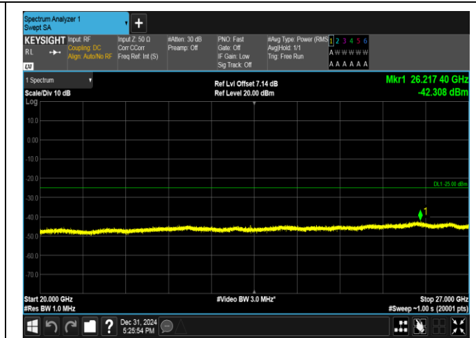
Band38-5MHz-16QAM-38000-1RB#24-20000~27000-PASS
