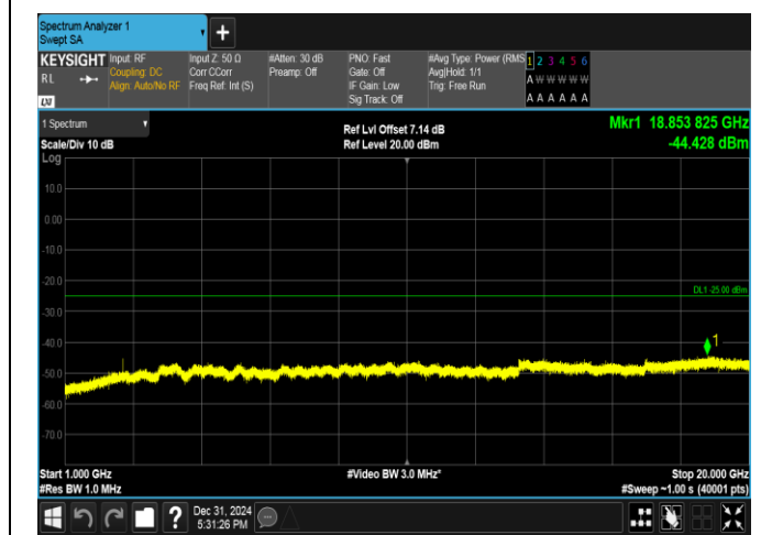
Band38-5MHz-16QAM-38225-1RB#24-1000~20000-PASS
