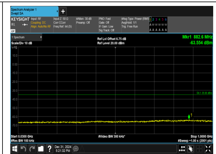
Band38-5MHz-16QAM-37775-25RB#0-30~1000-PASS
