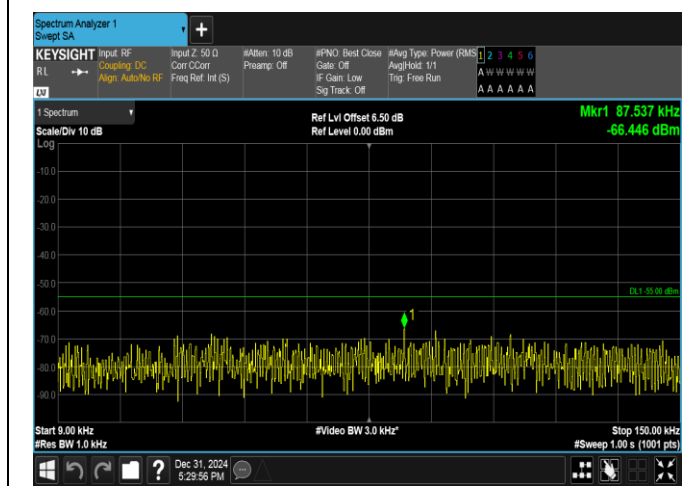
Band38-5MHz-QPSK-38225-1RB#24-0.009~0.15-PASS
