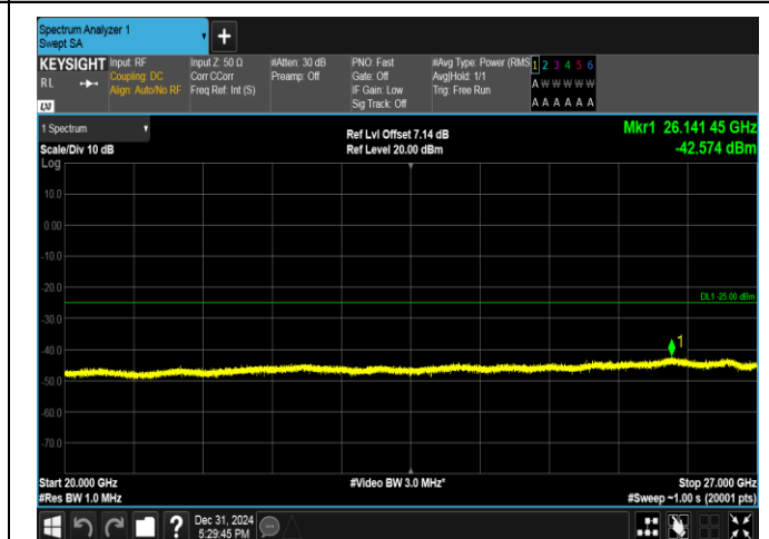
Band38-5MHz-16QAM-38225-1RB#0-20000~27000-PASS
