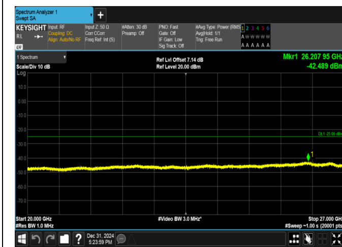
Band38-5MHz-16QAM-38000-1RB#0-20000~27000-PASS
