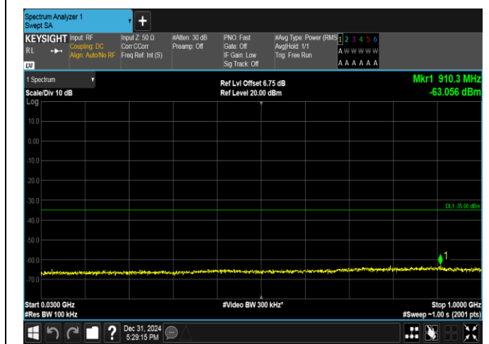
Band38-5MHz-16QAM-38225-1RB#0-30~1000-PASS
