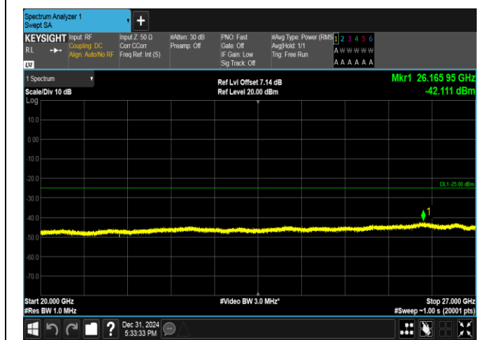
Band38-5MHz-16QAM-38225-25RB#0-20000~27000-PASS
