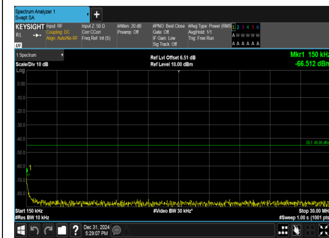
Band38-5MHz-16QAM-38225-1RB#0-0.15~30-PASS
