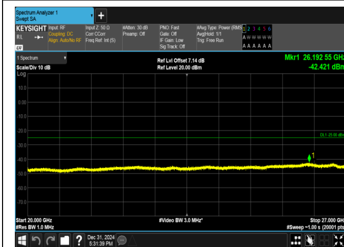
Band38-5MHz-16QAM-38225-1RB#24-20000~27000-PASS
