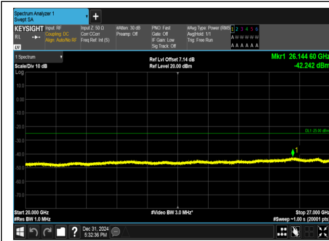
Band38-5MHz-QPSK-38225-25RB#0-20000~27000-PASS
