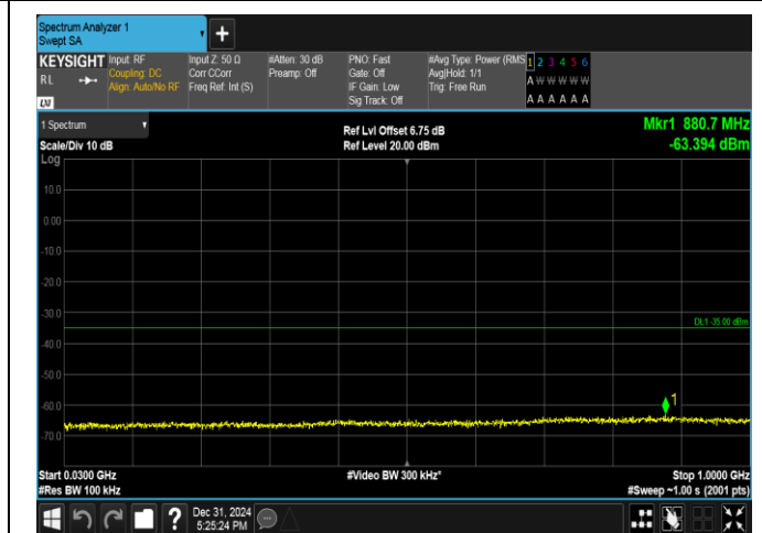
Band38-5MHz-16QAM-38000-1RB#24-30~1000-PASS
