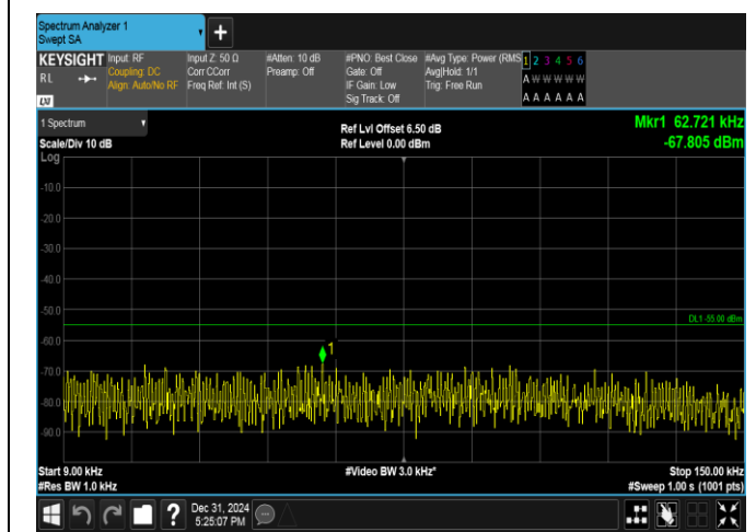
Band38-5MHz-16QAM-38000-1RB#24-0.009~0.15-PASS
