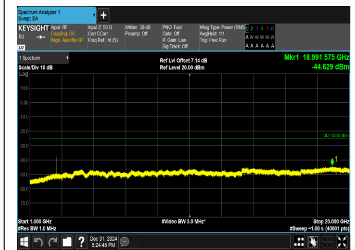
Band38-5MHz-QPSK-38000-1RB#24-1000~20000-PASS
