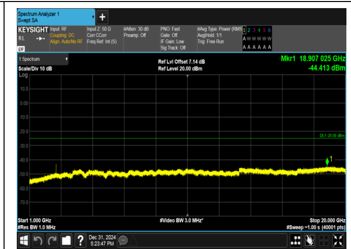
Band38-5MHz-16QAM-38000-1RB#0-1000~20000-PASS
