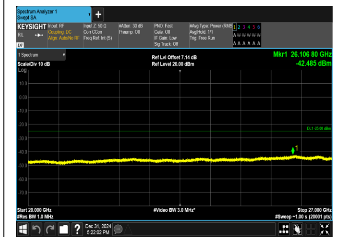
Band38-5MHz-16QAM-37775-25RB#0-20000~27000-PASS
