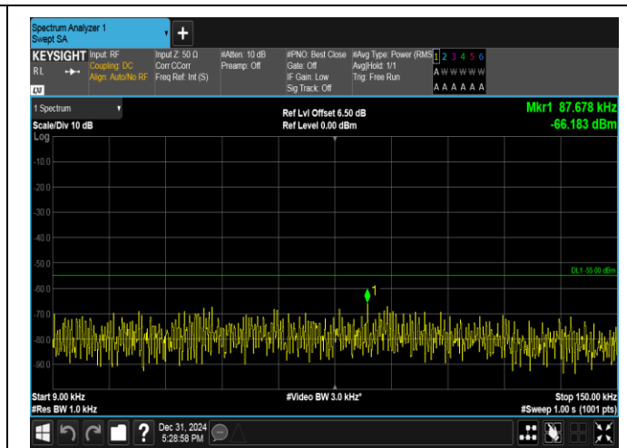
Band38-5MHz-16QAM-38225-1RB#0-0.009~0.15-PASS
