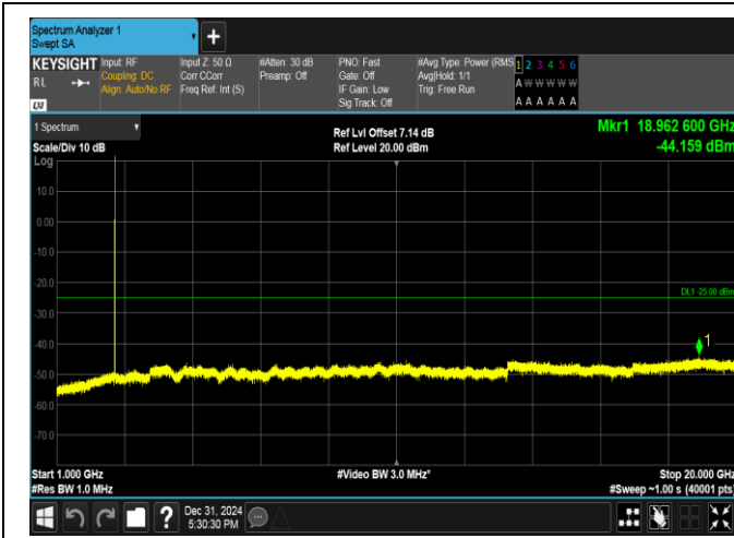
Band38-5MHz-QPSK-38225-1RB#24-1000~20000-PASS
