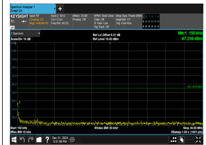
Band38-5MHz-QPSK-38225-25RB#0-0.15~30-PASS
