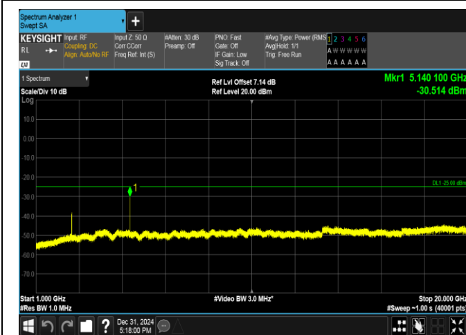
Band38-5MHz-16QAM-37775-1RB#0-1000~20000-PASS
