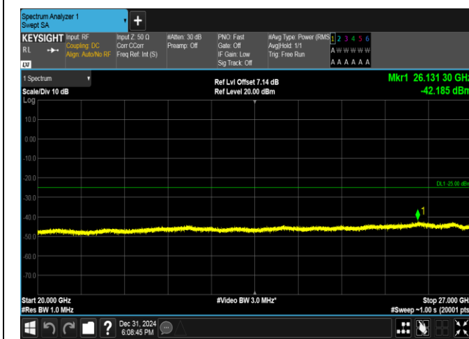
Band38-10MHz-QPSK-37800-1RB#0-20000~27000-PASS
