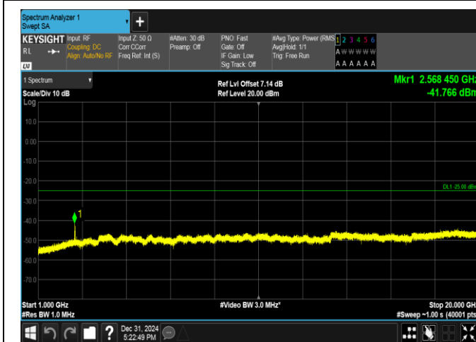
Band38-5MHz-QPSK-38000-1RB#0-1000~20000-PASS
