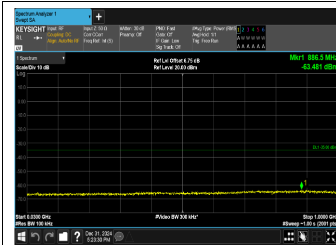
Band38-5MHz-16QAM-38000-1RB#0-30~1000-PASS
