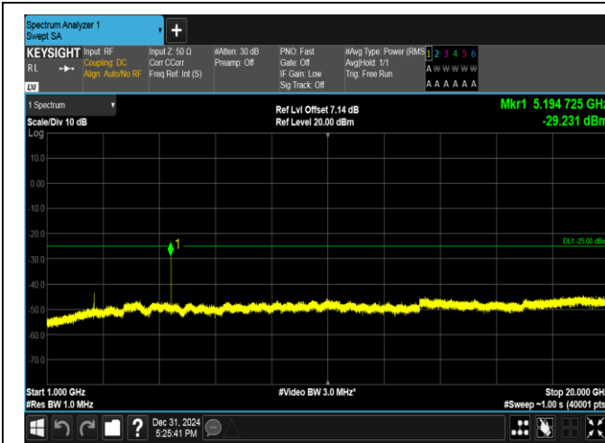
Band38-5MHz-16QAM-38000-1RB#24-1000~20000-PASS
