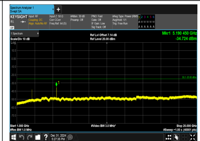
Band38-5MHz-16QAM-38000-25RB#0-1000~20000-PASS
