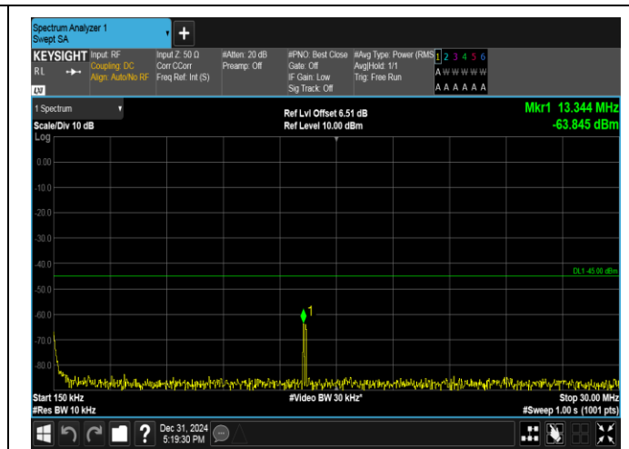
Band38-5MHz-16QAM-37775-1RB#24-0.15~30-PASS
