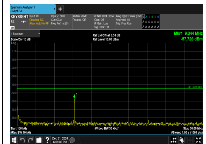
Band38-10MHz-QPSK-37800-1RB#0-0.15~30-PASS
