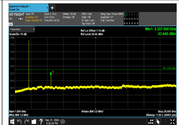
Band38-5MHz-QPSK-38225-25RB#0-1000~20000-PASS
