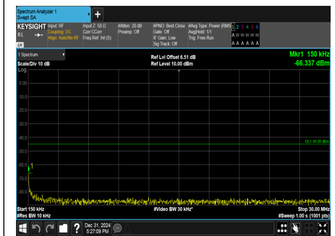
Band38-5MHz-16QAM-38000-25RB#0-0.15~30-PASS
