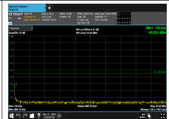
Band38-5MHz-QPSK-38225-1RB#0-0.15~30-PASS
