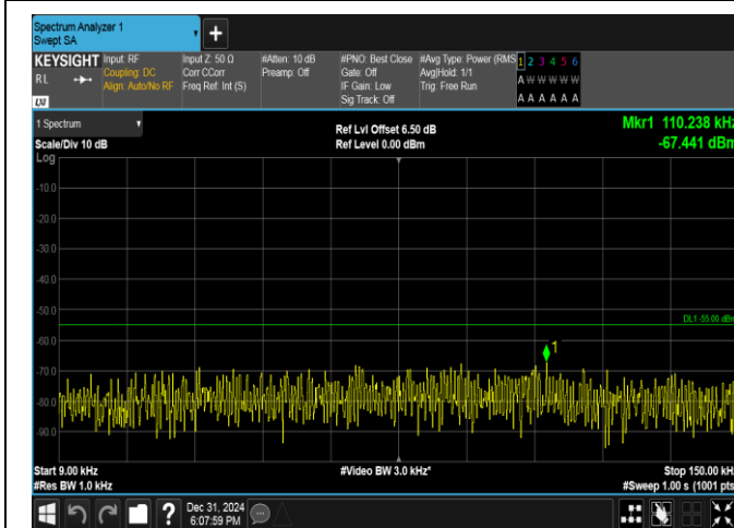
Band38-10MHz-QPSK-37800-1RB#0-0.009~0.15-PASS
