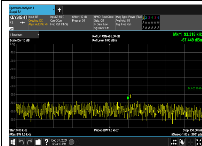
Band38-5MHz-16QAM-38000-1RB#0-0.009~0.15-PASS
