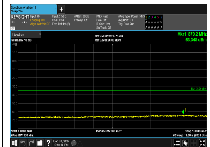
Band38-10MHz-QPSK-37800-1RB#49-30~1000-PASS
