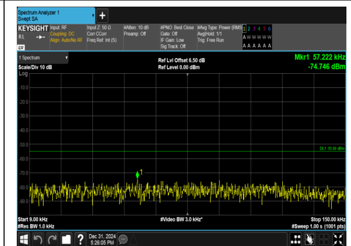
Band38-5MHz-QPSK-38000-25RB#0-0.009~0.15-PASS
