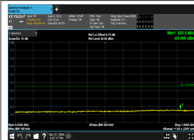
Band38-5MHz-16QAM-38000-25RB#0-30~1000-PASS
