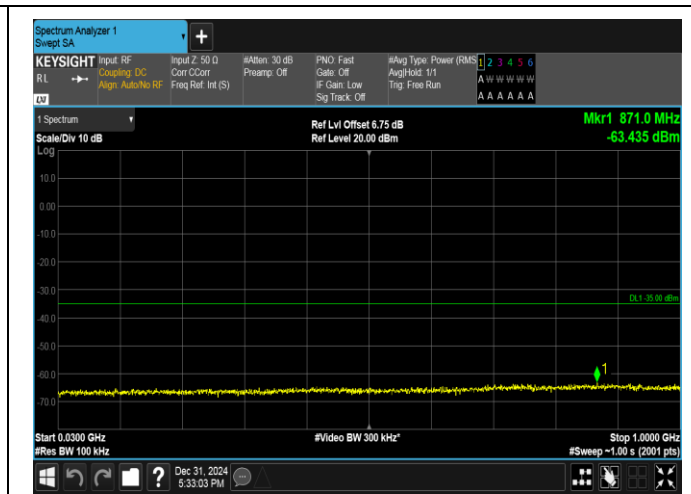
Band38-5MHz-16QAM-38225-25RB#0-30~1000-PASS
