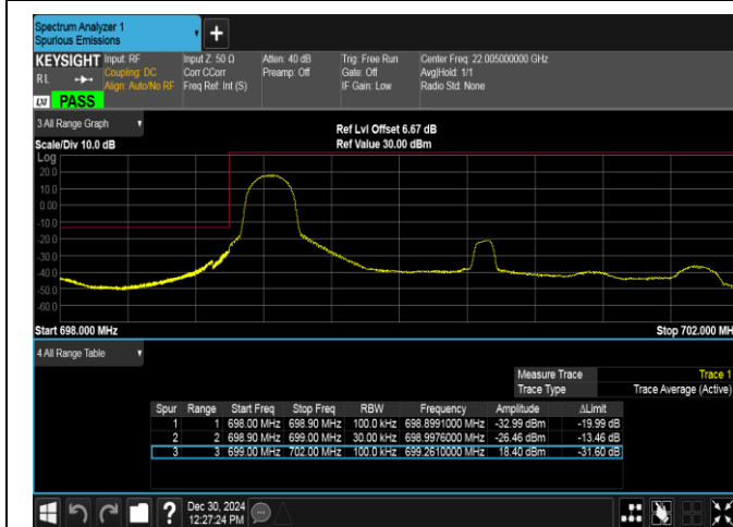
Band12-3MHz-16QAM-23025-1RB#0-PASS
