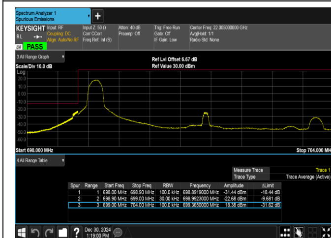
Band12-5MHz-16QAM-23035-1RB#0-PASS
