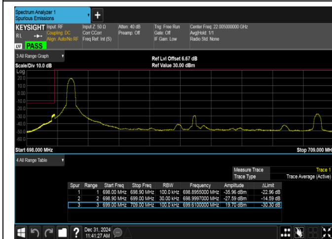
Band12-10MHz-QPSK-23060-1RB#0-PASS
