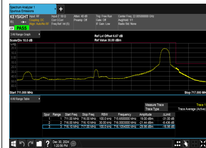
Band12-5MHz-QPSK-23155-1RB#24-PASS
