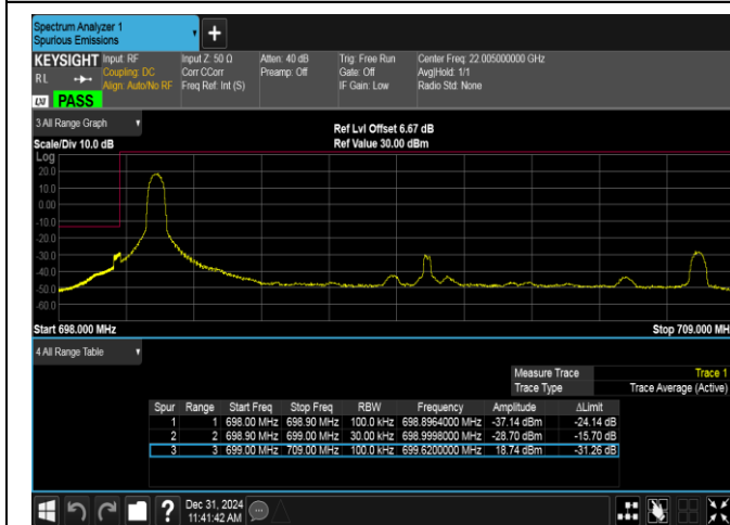
Band12-10MHz-16QAM-23060-1RB#0-PASS
