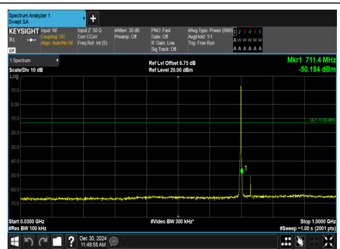
Band12-1.4MHz-QPSK-23095-6RB#0-30~1000-PASS
