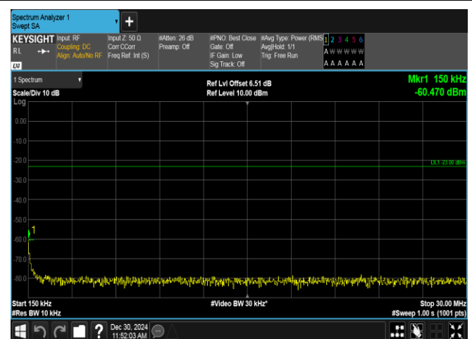
Band12-1.4MHz-QPSK-23173-1RB#0-0.15~30-PASS
