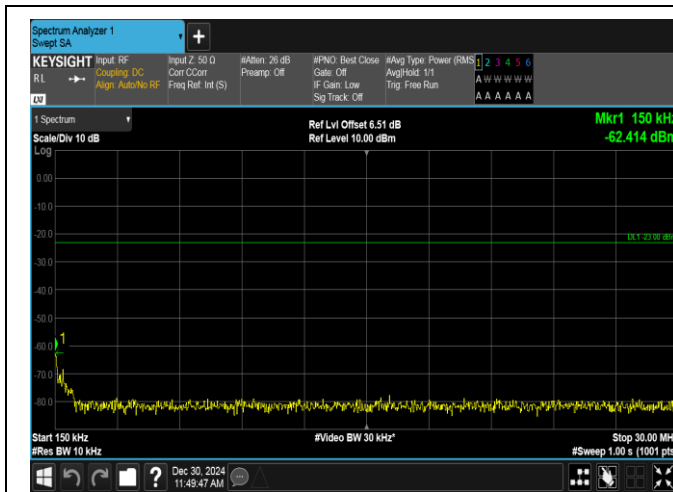
Band12-1.4MHz-QPSK-23095-6RB#0-0.15~30-PASS
