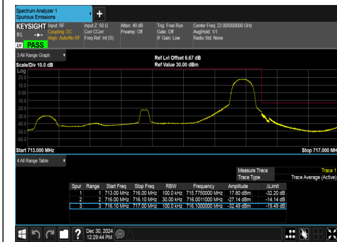
Band12-3MHz-16QAM-23165-1RB#14-PASS
