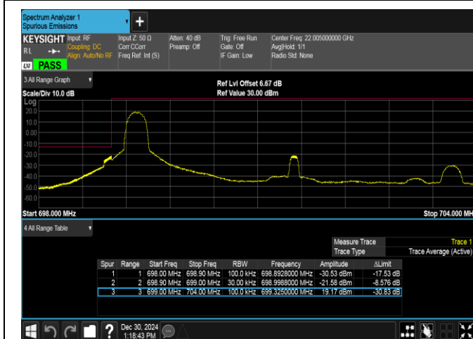
Band12-5MHz-QPSK-23035-1RB#0-PASS
