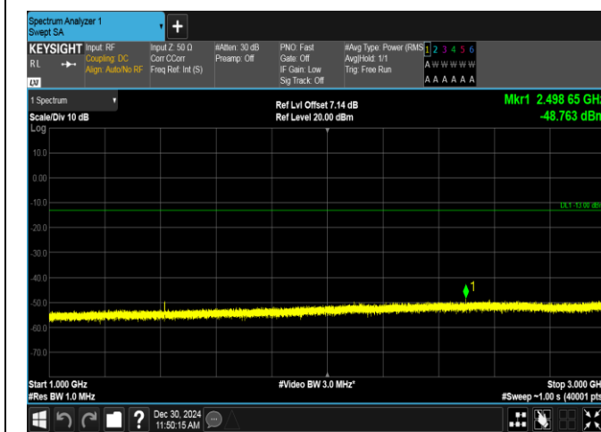
Band12-1.4MHz-QPSK-23095-6RB#0-1000~3000-PASS
