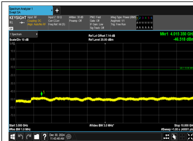
Band12-1.4MHz-QPSK-23017-6RB#0-3000~10000-PASS
