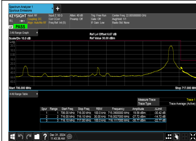
Band12-10MHz-QPSK-23130-1RB#49-PASS
