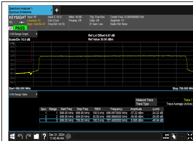
Band12-10MHz-16QAM-23060-50RB#0-PASS
