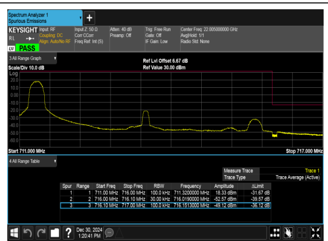
Band12-5MHz-16QAM-23155-1RB#0-PASS
