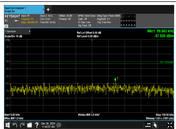
Band12-1.4MHz-QPSK-23095-1RB#0-0.009~0.15-PASS
