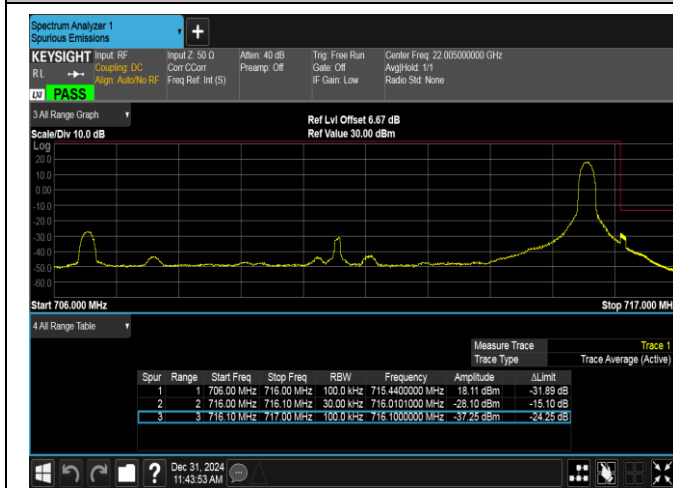
Band12-10MHz-16QAM-23130-1RB#49-PASS
