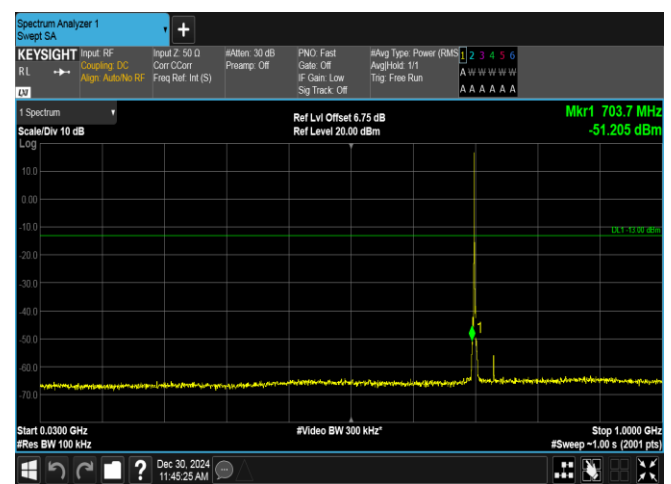
Band12-1.4MHz-QPSK-23095-1RB#0-30~1000-PASS
