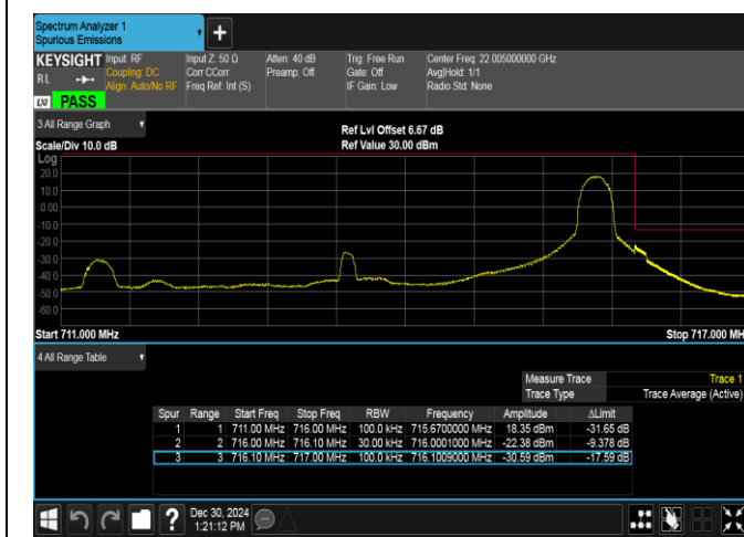
Band12-5MHz-16QAM-23155-1RB#24-PASS
