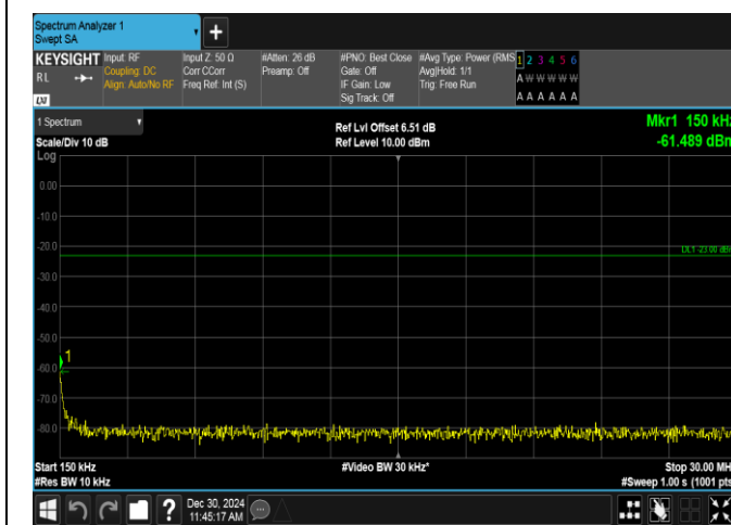
Band12-1.4MHz-QPSK-23095-1RB#0-0.15~30-PASS
