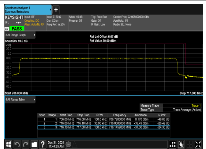
Band12-10MHz-16QAM-23130-50RB#0-PASS
