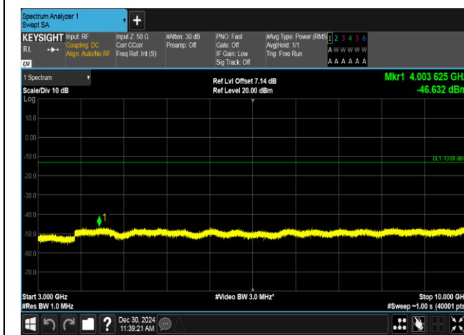
Band12-1.4MHz-QPSK-23017-1RB#0-3000~10000-PASS
