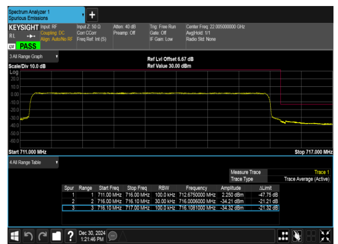
Band12-5MHz-16QAM-23155-25RB#0-PASS
