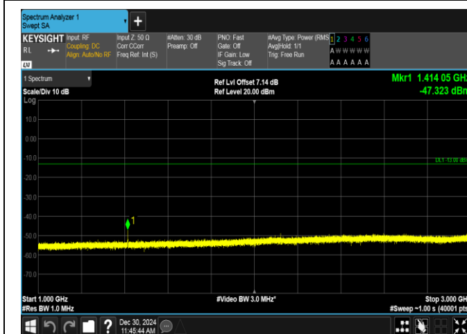
Band12-1.4MHz-QPSK-23095-1RB#0-1000~3000-PASS
