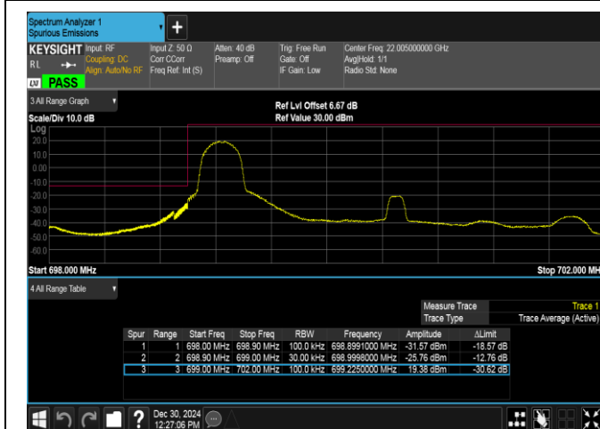
Band12-3MHz-QPSK-23025-1RB#0-PASS
