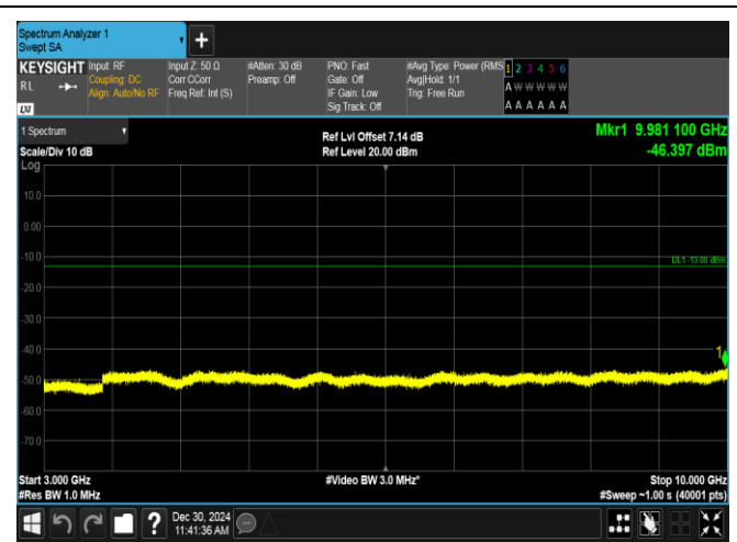
Band12-1.4MHz-QPSK-23017-1RB#5-3000~10000-PASS
