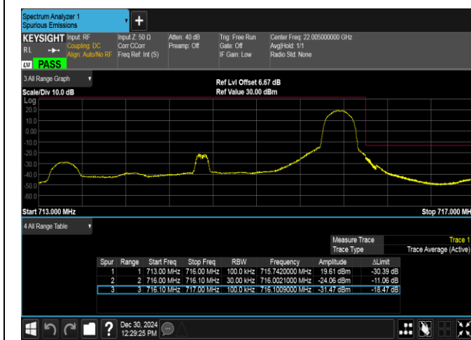
Band12-3MHz-QPSK-23165-1RB#14-PASS
