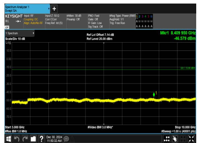
Band12-1.4MHz-QPSK-23095-6RB#0-3000~10000-PASS
