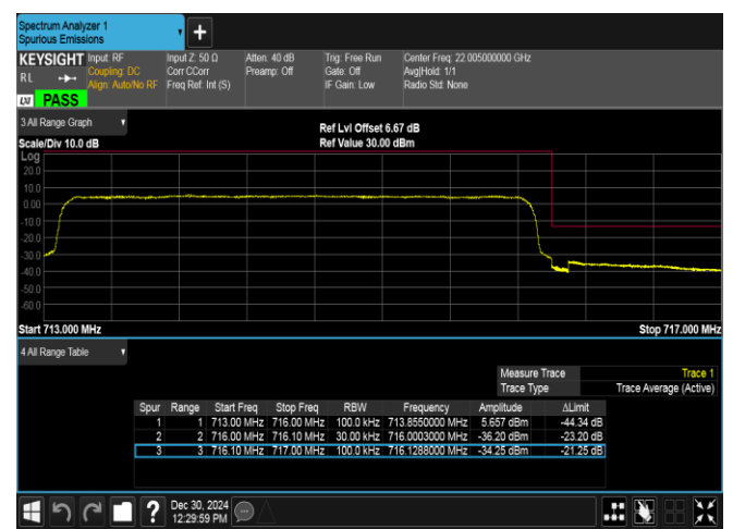
Band12-3MHz-QPSK-23165-15RB#0-PASS
