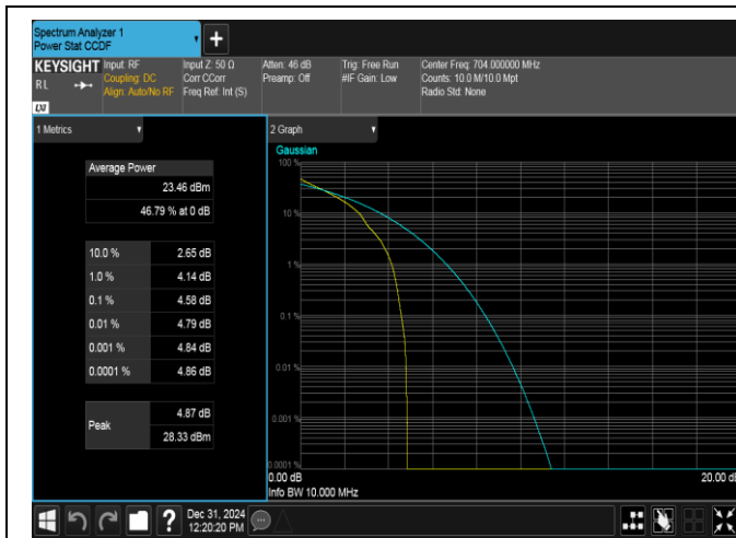
Band12-10MHz-QPSK-23060-1RB#0-PASS
