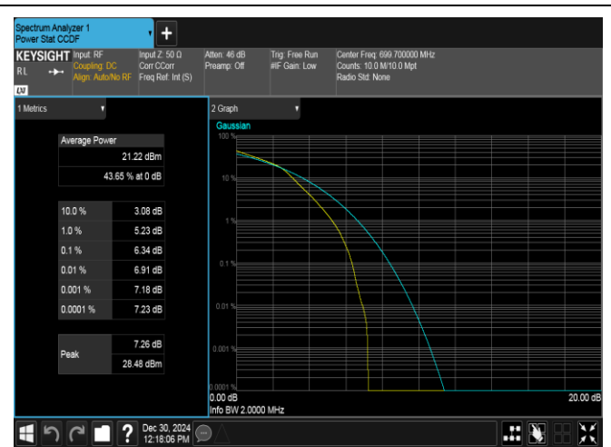
Band12-1.4MHz-16QAM-23017-6RB#0-PASS
