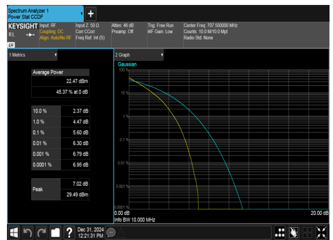
Band12-10MHz-QPSK-23095-50RB#0-PASS
