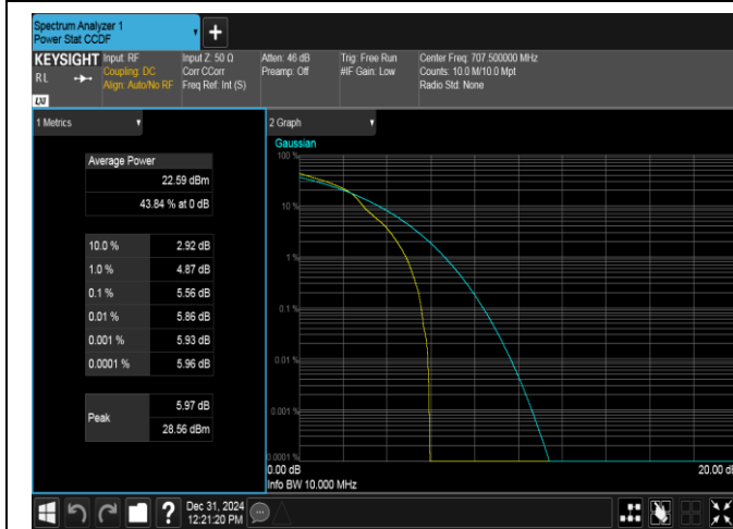
Band12-10MHz-16QAM-23095-1RB#0-PASS
