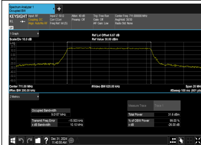
Band12-10MHz-QPSK-23130-50RB#0-PASS
