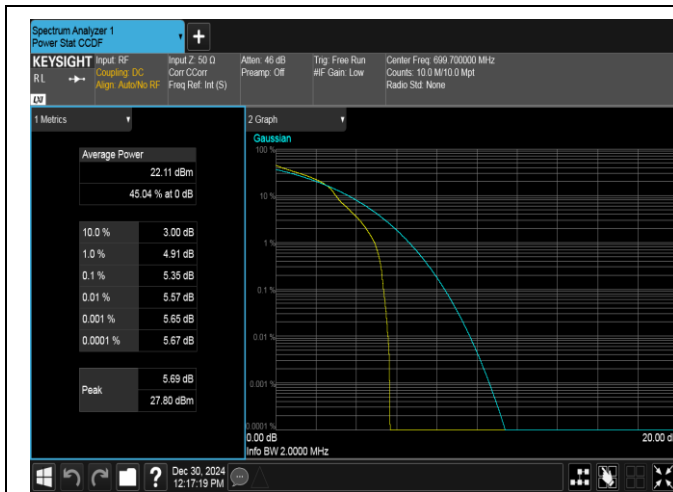
Band12-1.4MHz-16QAM-23017-1RB#0-PASS
