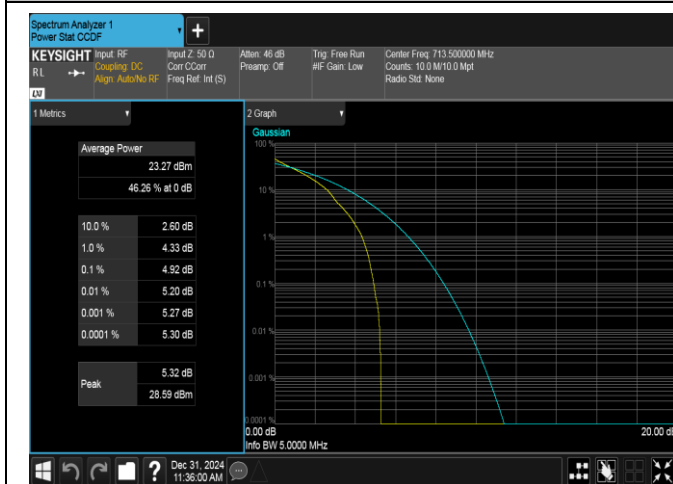
Band12-5MHz-QPSK-23155-1RB#0-PASS
