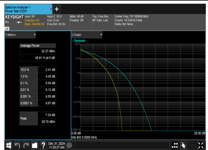
Band12-5MHz-QPSK-23095-25RB#0-PASS
