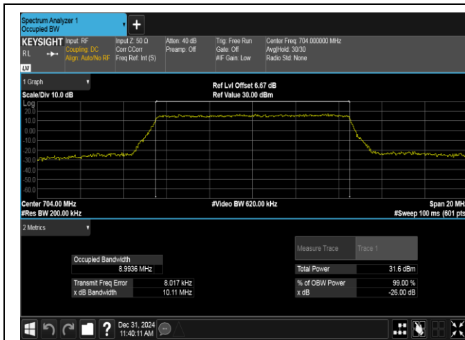
Band12-10MHz-QPSK-23060-50RB#0-PASS
