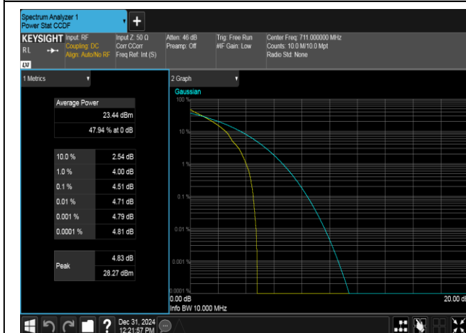
Band12-10MHz-QPSK-23130-1RB#0-PASS
