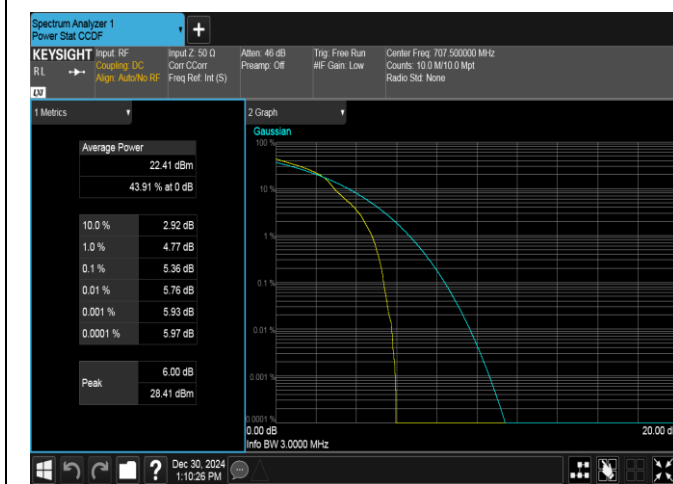
Band12-3MHz-16QAM-23095-1RB#0-PASS
