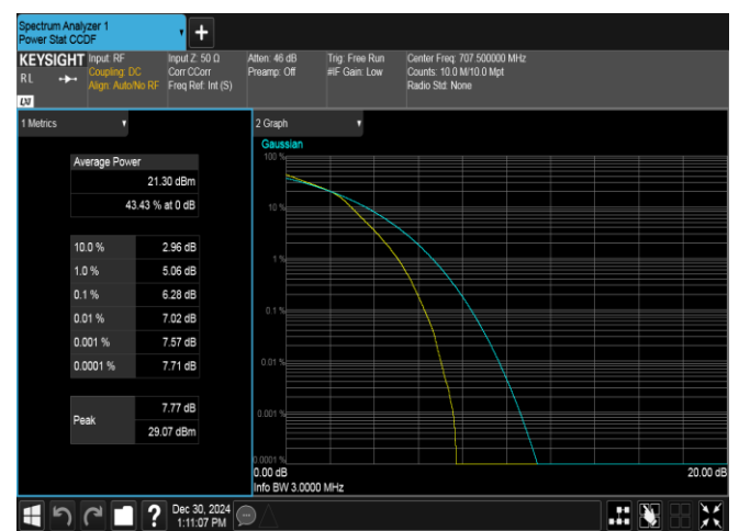
Band12-3MHz-16QAM-23095-15RB#0-PASS
