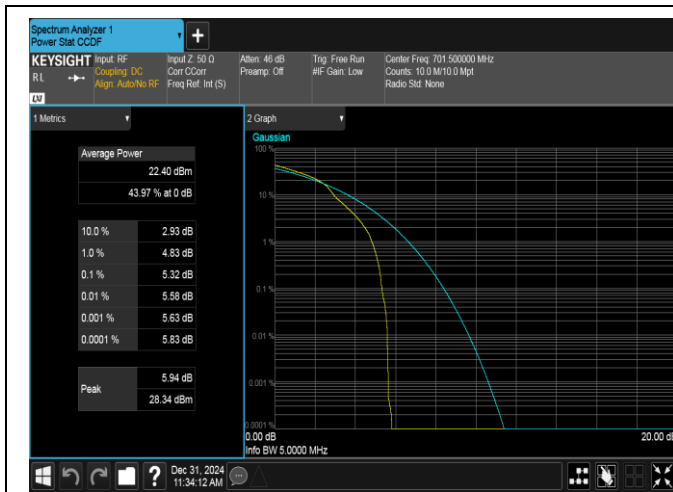
Band12-5MHz-16QAM-23035-1RB#0-PASS
