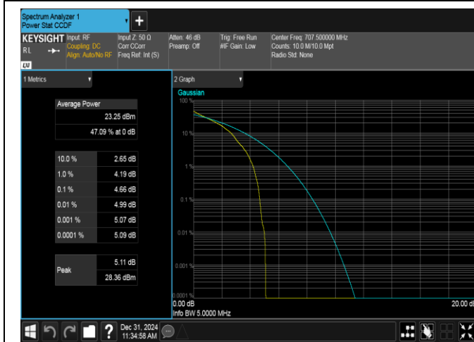
Band12-5MHz-QPSK-23095-1RB#0-PASS
