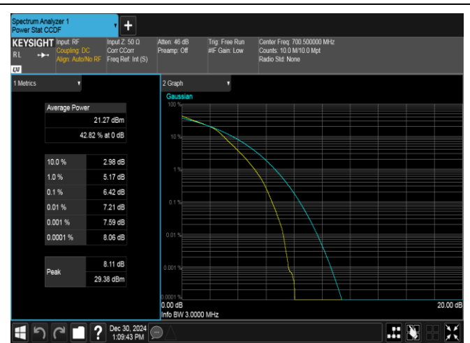
Band12-3MHz-16QAM-23025-15RB#0-PASS
