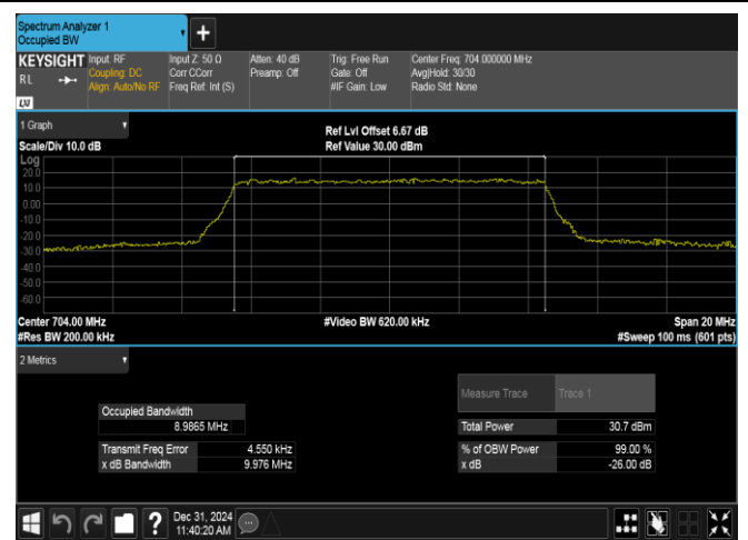
Band12-10MHz-16QAM-23060-50RB#0-PASS
