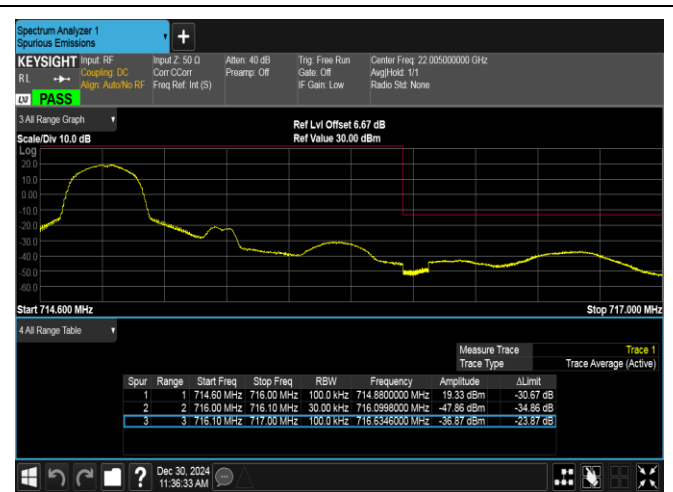
Band12-1.4MHz-QPSK-23173-1RB#0-PASS
