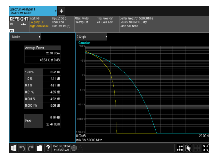
Band12-5MHz-QPSK-23035-1RB#0-PASS
