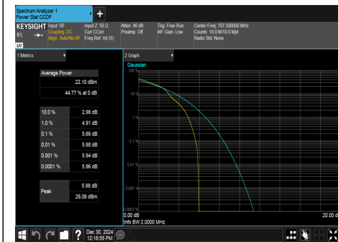
Band12-1.4MHz-16QAM-23095-1RB#0-PASS
