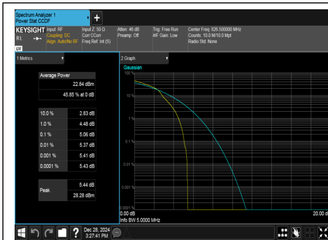
Band5-5MHz-16QAM-20425-1RB#0-PASS
