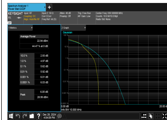
Band5-10MHz-16QAM-20525-1RB#0-PASS
