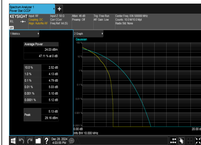
Band5-10MHz-QPSK-20525-1RB#0-PASS
