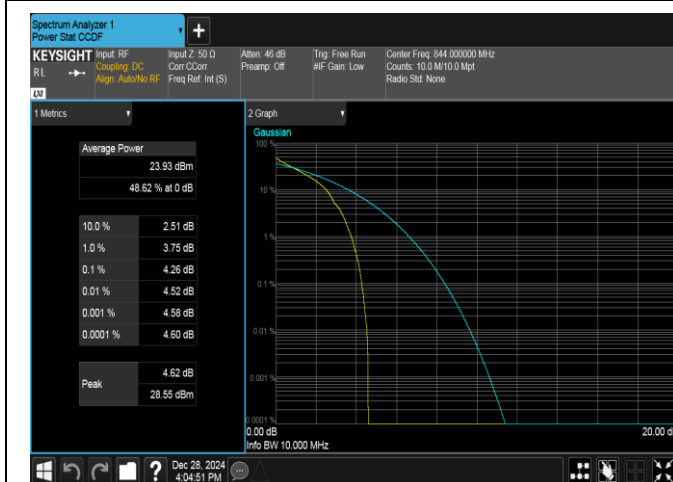
Band5-10MHz-QPSK-20600-1RB#0-PASS
