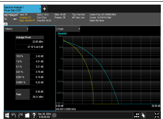
Band5-3MHz-QPSK-20415-15RB#0-PASS
