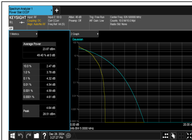
Band5-5MHz-QPSK-20425-1RB#0-PASS
