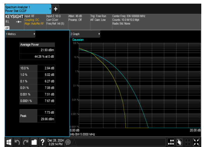
Band5-5MHz-16QAM-20525-25RB#0-PASS
