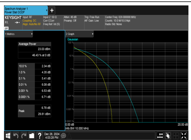
Band5-10MHz-QPSK-20450-50RB#0-PASS
