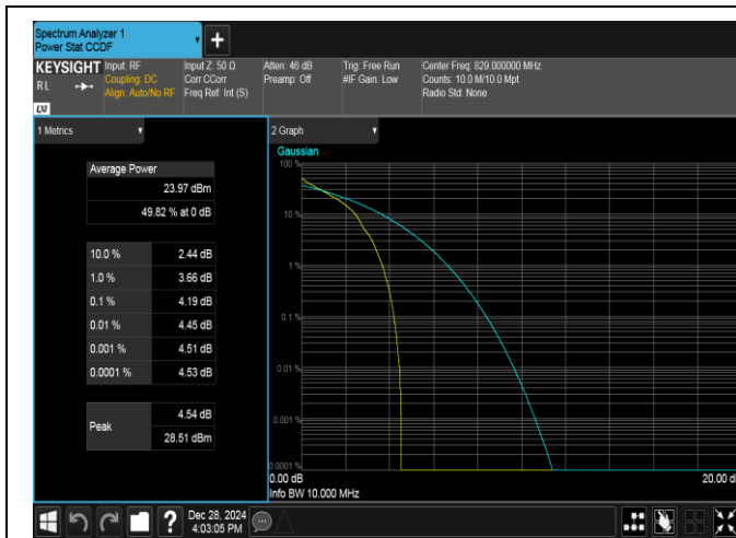
Band5-10MHz-QPSK-20450-1RB#0-PASS
