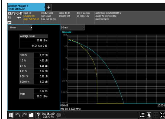
Band5-5MHz-16QAM-20525-1RB#0-PASS
