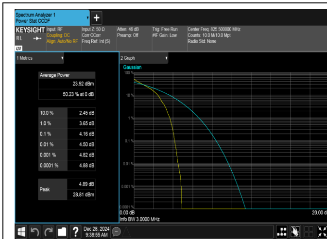
Band5-3MHz-QPSK-20415-1RB#0-PASS
