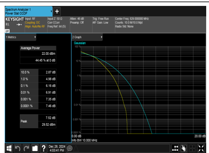
Band5-10MHz-16QAM-20450-50RB#0-PASS
