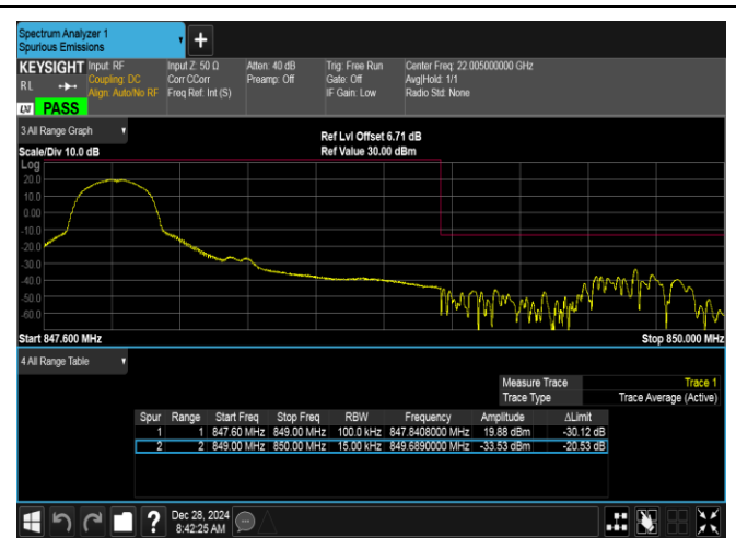
Band5-1.4MHz-QPSK-20643-1RB#0-PASS
