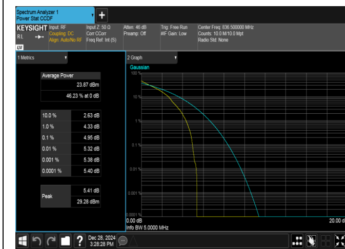
Band5-5MHz-QPSK-20525-1RB#0-PASS
