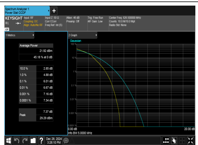
Band5-5MHz-16QAM-20425-25RB#0-PASS
