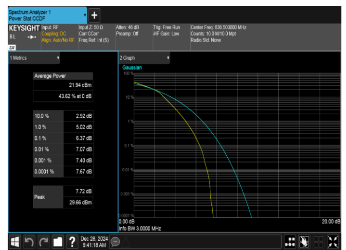
Band5-3MHz-16QAM-20525-15RB#0-PASS
