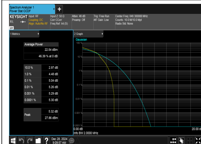
Band5-1.4MHz-16QAM-20643-1RB#0-PASS
