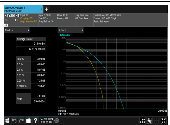
Band5-3MHz-16QAM-20415-15RB#0-PASS
