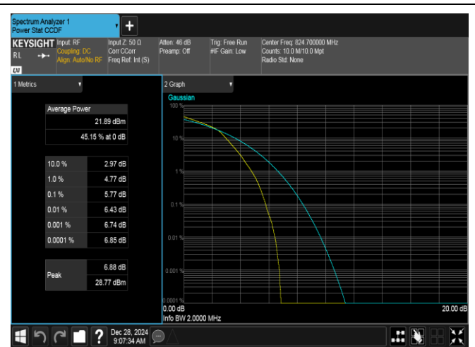
Band5-1.4MHz-16QAM-20407-6RB#0-PASS
