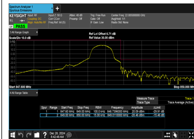
Band5-1.4MHz-QPSK-20643-1RB#5-PASS
