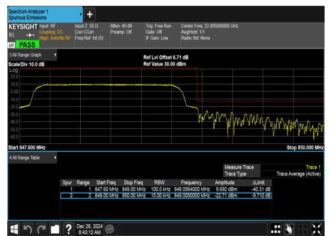
Band5-1.4MHz-QPSK-20643-6RB#0-PASS
