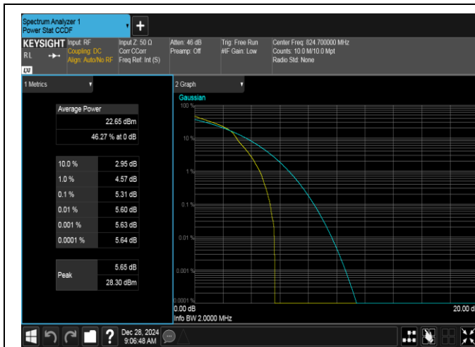
Band5-1.4MHz-16QAM-20407-1RB#0-PASS
