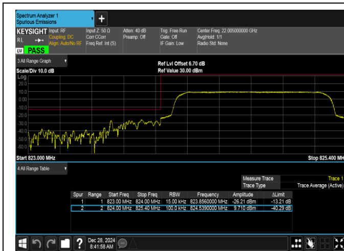
Band5-1.4MHz-QPSK-20407-6RB#0-PASS
