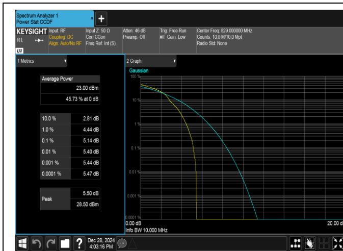
Band5-10MHz-16QAM-20450-1RB#0-PASS
