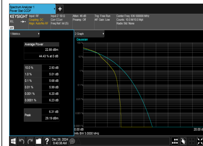
Band5-3MHz-16QAM-20525-1RB#0-PASS
