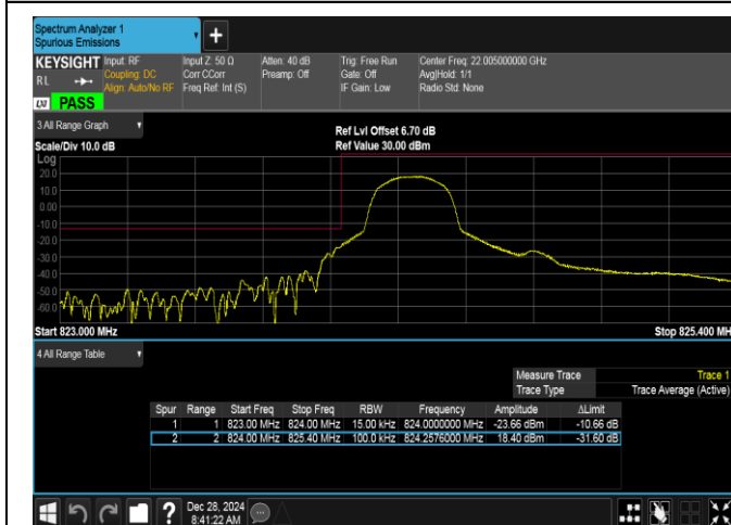
Band5-1.4MHz-16QAM-20407-1RB#0-PASS
