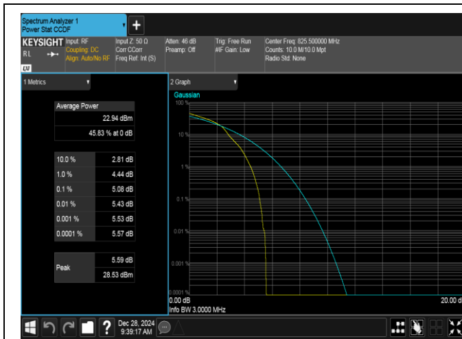
Band5-3MHz-16QAM-20415-1RB#0-PASS
