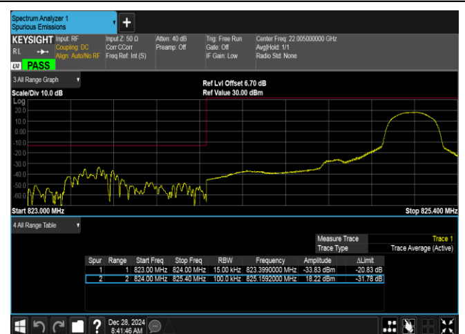
Band5-1.4MHz-16QAM-20407-1RB#5-PASS
