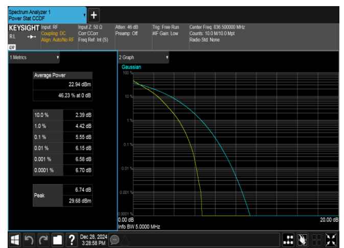
Band5-5MHz-QPSK-20525-25RB#0-PASS
