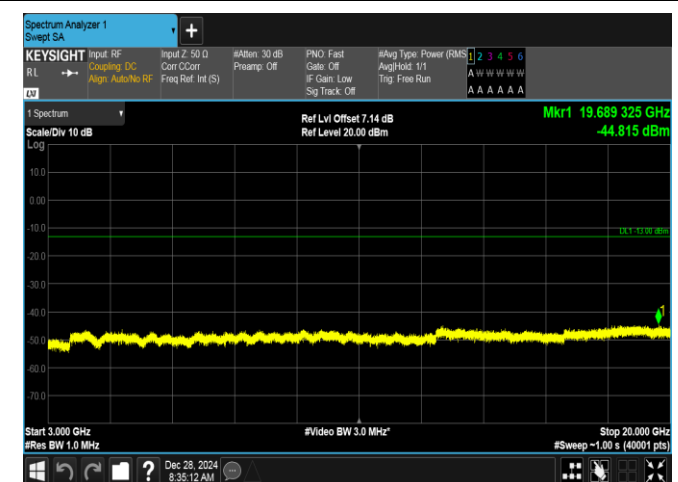
Band2-20MHz-16QAM-19100-100RB#0-3000~20000-PAS
