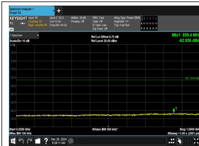
Band2-20MHz-16QAM-18900-100RB#0-30~1000-PASS
