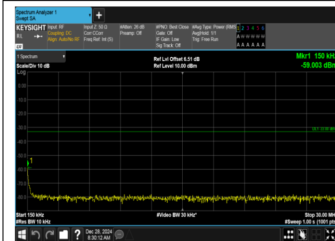
Band2-20MHz-16QAM-19100-1RB#0-0.15~30-PASS
