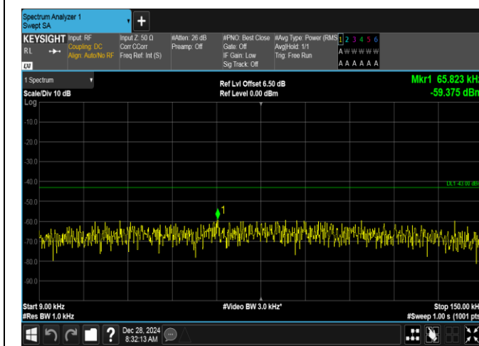
Band2-20MHz-16QAM-19100-1RB#99-0.009~0.15-PASS
