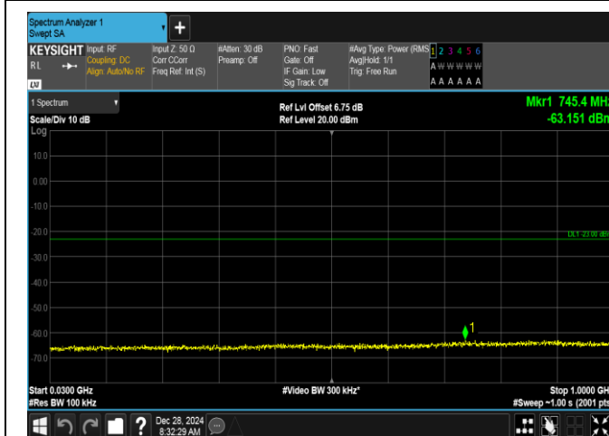
Band2-20MHz-16QAM-19100-1RB#99-30~1000-PASS
