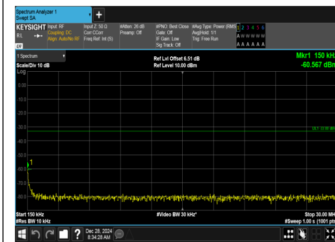
Band2-20MHz-16QAM-19100-100RB#0-0.15~30-PASS
