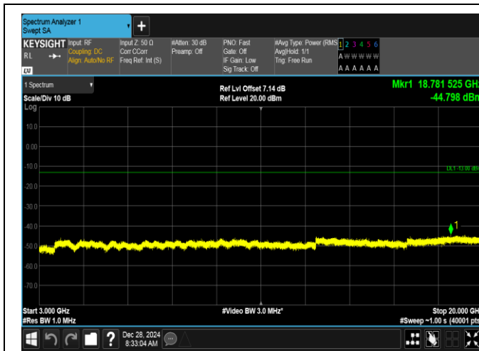
Band2-20MHz-16QAM-19100-1RB#99-3000~20000-PASS
