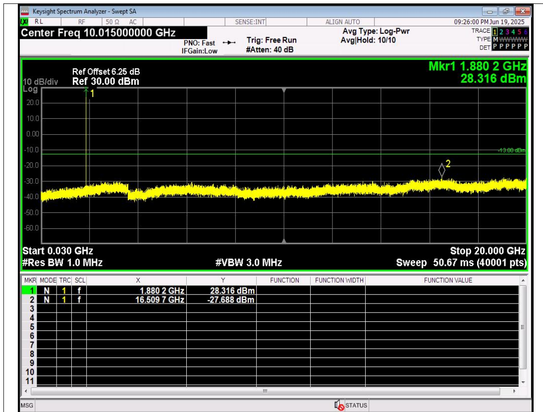
GPRS1900 Channel=661
