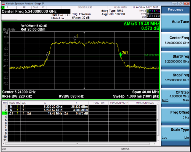
11AC20MIMO-Ant2-5240
