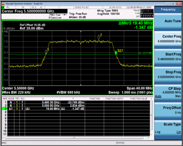
11AC20MIMO-Ant1-5500
