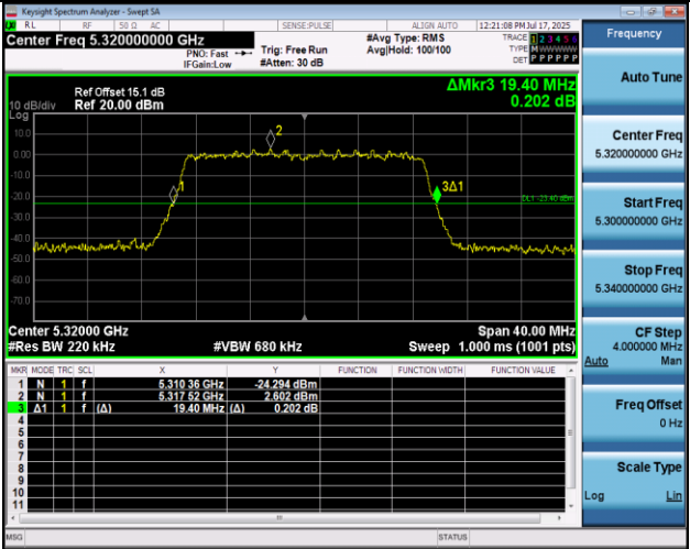
11AC20MIMO-Ant1-5320
