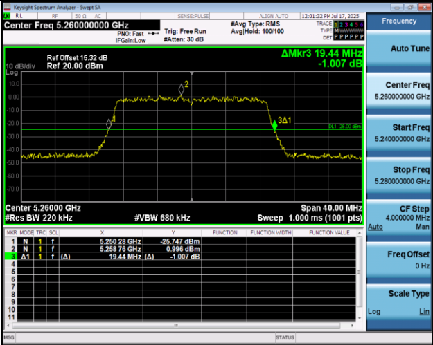
11AC20MIMO-Ant2-5260
