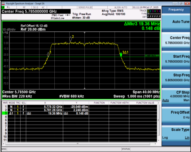
11AC20MIMO-Ant1-5785
