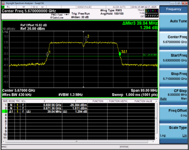
11N40MIMO-Ant2-5670
