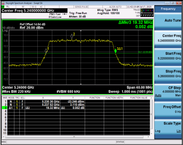
11AC20MIMO-Ant1-5240
