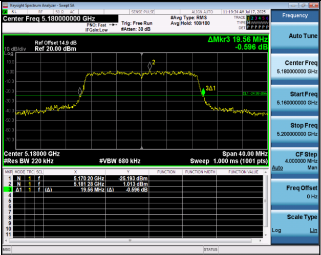
11AC20MIMO-Ant2-5180
