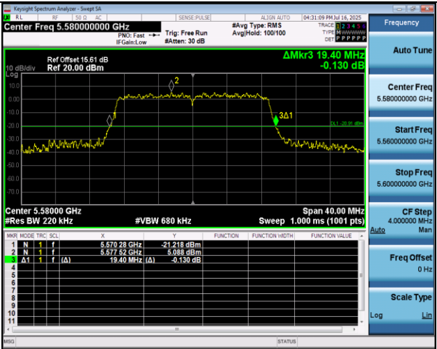
11N20MIMO-Ant2-5580
