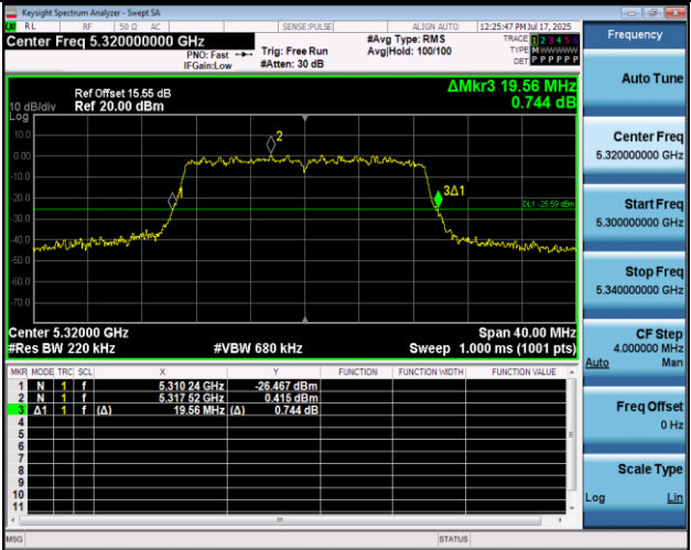
11AC20MIMO-Ant2-5320
