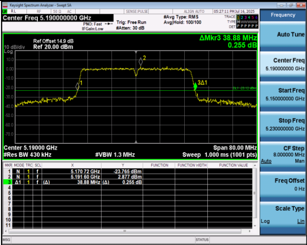
11N40MIMO-Ant2-5190
