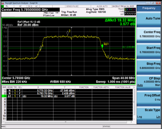
11N20MIMO-Ant1-5785
