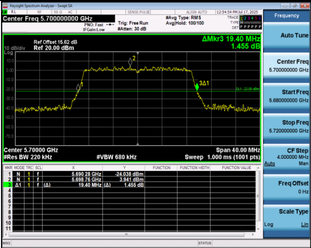
11AC20MIMO-Ant2-5700
