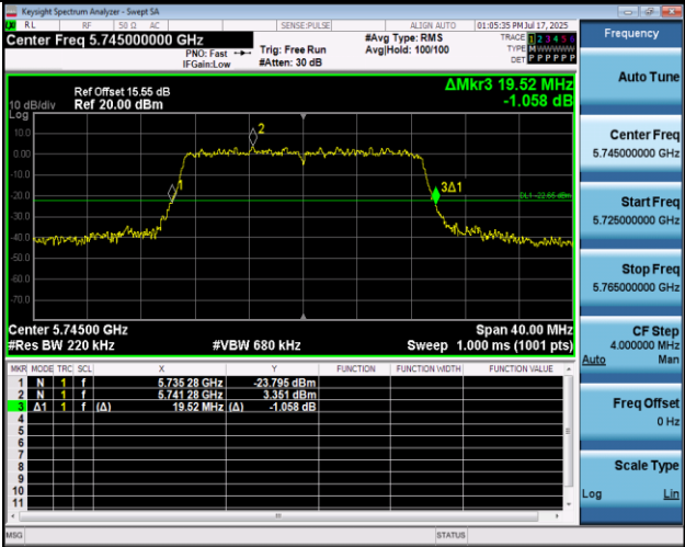
11AC20MIMO-Ant2-5745
