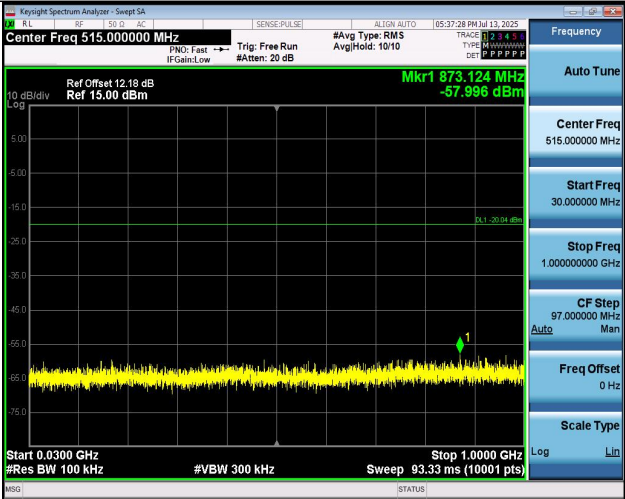
11N40MIMO-Ant2-2422-30~1000-PASS
