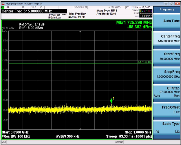
11AX20MIMO-Ant2-2437-30~1000-PASS
