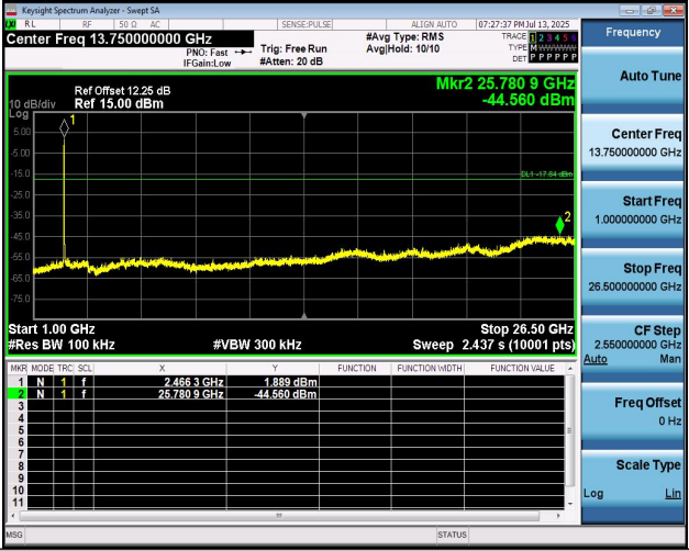
11AX20MIMO-Ant2-2462-1000~26500-PASS
