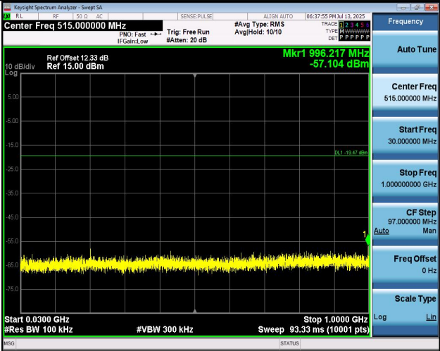
11N40MIMO-Ant2-2452-30~1000-PASS
