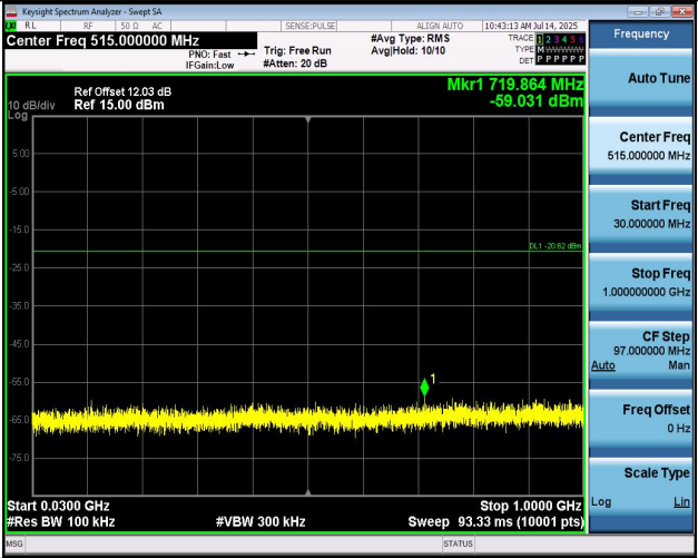
11AX40MIMO-Ant1-2437-30~1000-PASS
