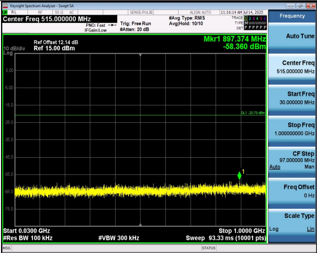
11AX40MIMO-Ant1-2452-30~1000-PASS
