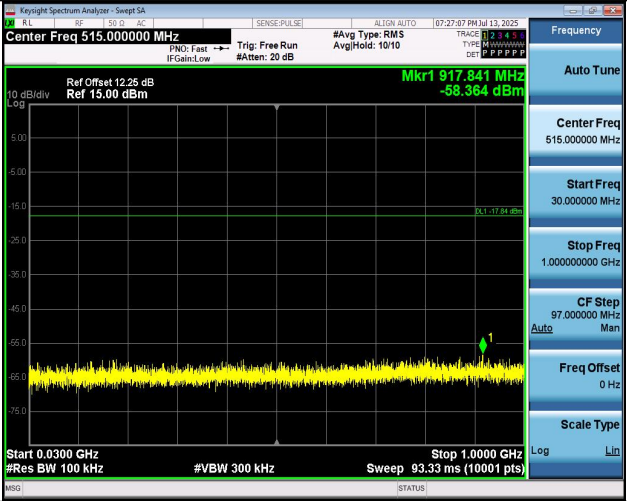
11AX20MIMO-Ant2-2462-30~1000-PASS
