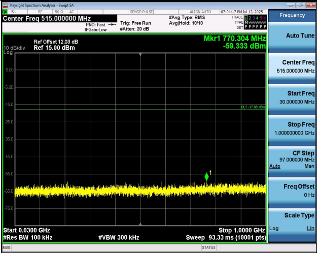
11AX20MIMO-Ant1-2437-30~1000-PASS
