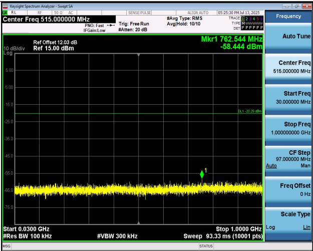
11N40MIMO-Ant1-2422-30~1000-PASS
