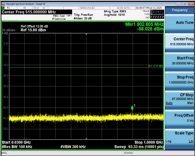
11AX20MIMO-Ant1-2412-30~1000-PASS
