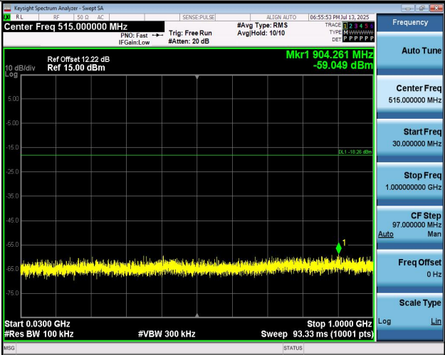
11AX20MIMO-Ant2-2412-30~1000-PASS
