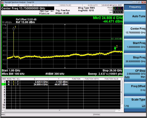
11AX40MIMO-Ant1-2437-1000~26500-PASS
