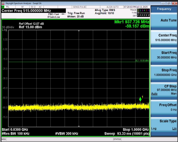
11AX20MIMO-Ant1-2462-30~1000-PASS
