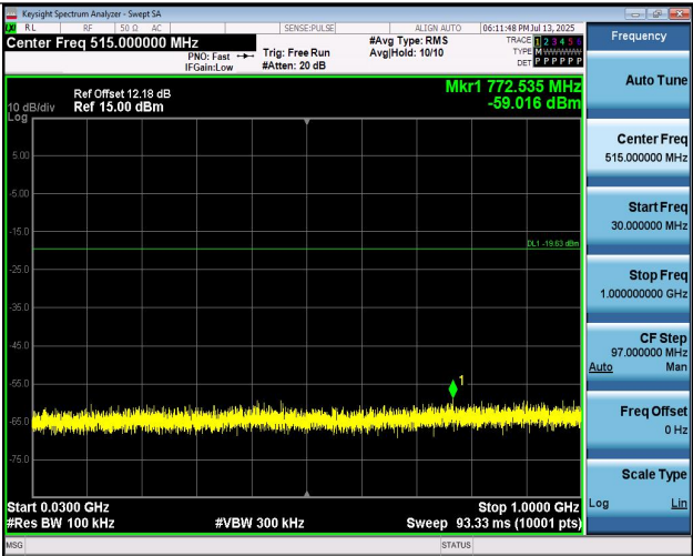
11N40MIMO-Ant2-2437-30~1000-PASS
