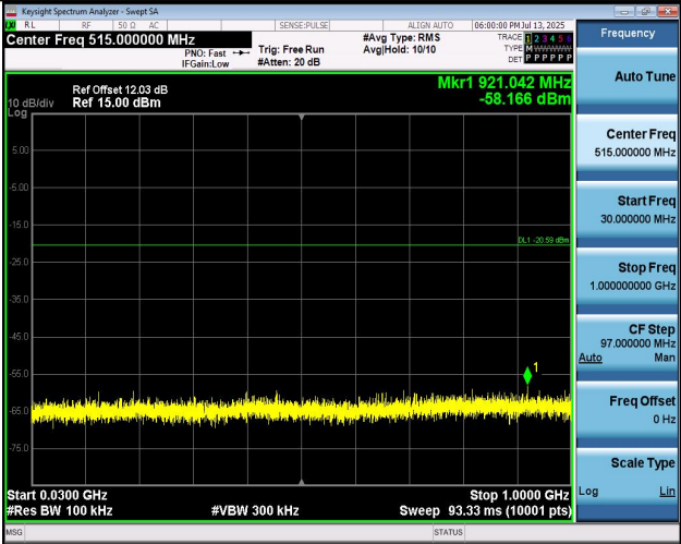
11N40MIMO-Ant1-2437-30~1000-PASS
