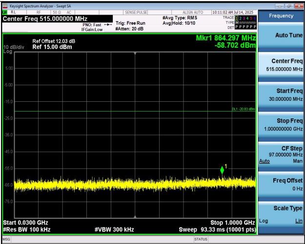
11AX40MIMO-Ant1-2422-30~1000-PASS
