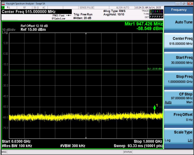
11AX40MIMO-Ant2-2422-30~1000-PASS
