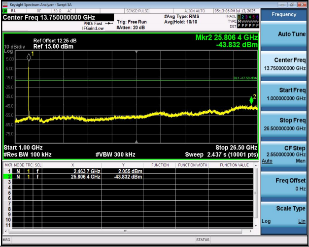
11N20MIMO-Ant2-2462-1000~26500-PASS
