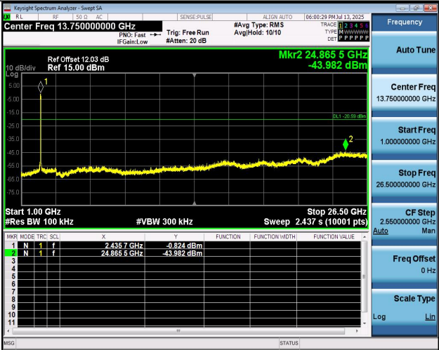
11N40MIMO-Ant1-2437-1000~26500-PASS
