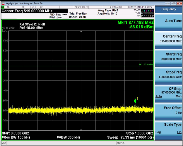
11N40MIMO-Ant1-2452-30~1000-PASS
