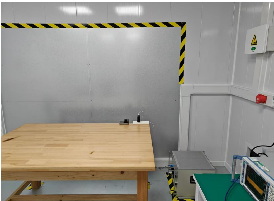
Wireless Power Transmission: Conducted Emission
