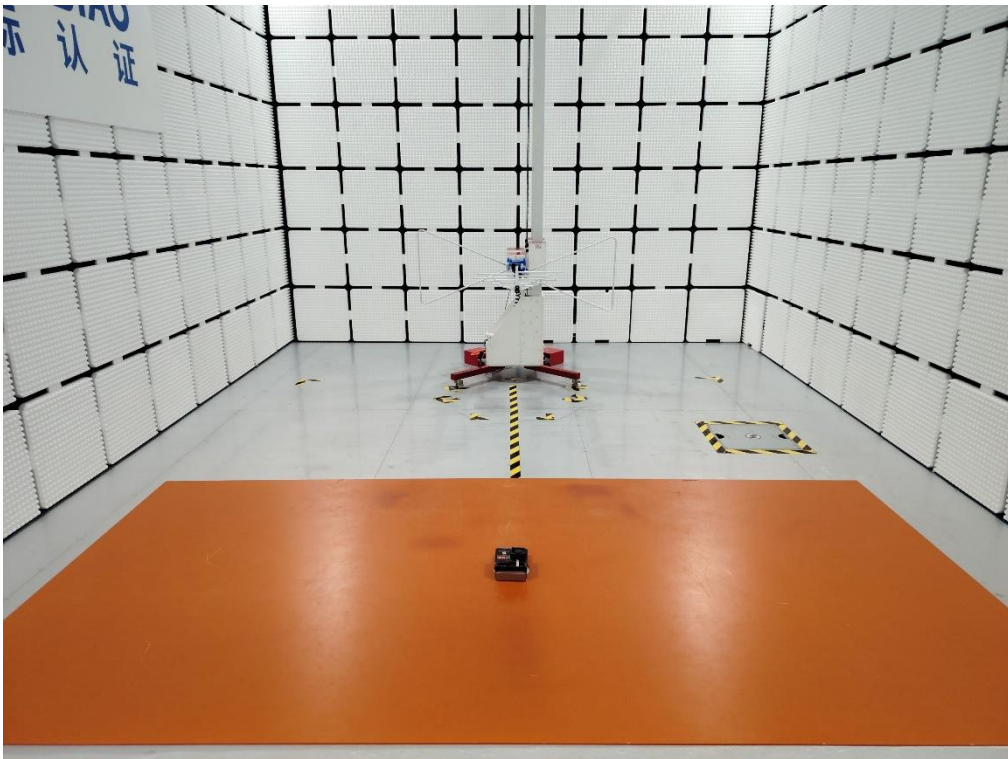
Wireless Power Transmission: Radiated Emission Above 30MHz
