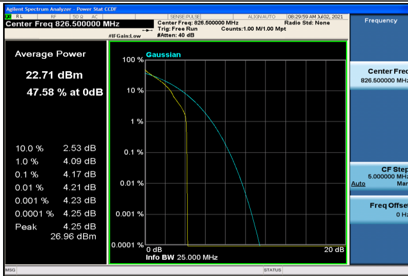
Band26-5MHz-QPSK-26815-1RB#0
