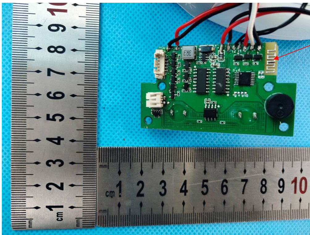
PCB Antenna
