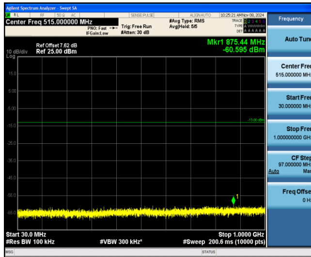
Band25-1.4MHz-QPSK-26047-1-0-Low-30-1000--60.6-PASS
