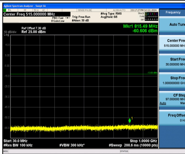
Band4-20MHz-1RB#0@Low-20300-1-0-High-30-1000--60.61-PASS
