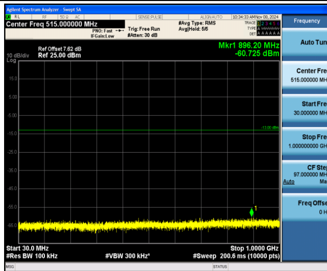
Band25-3MHz-16QAM-26365-1-0-Low-30-1000--60.73-PASS
