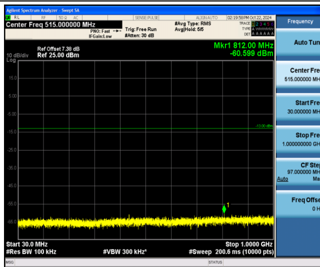
Band4-10MHz-16QAM-20175-1-0-Low-30-1000--60.6-PASS
