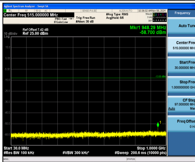
Band25-3MHz-16QAM-26675-1-0-Low-30-1000--58.7-PASS
