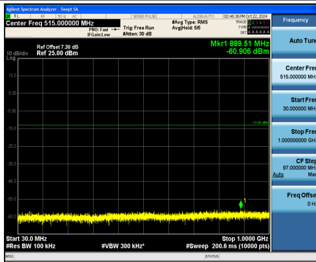
Band4-15MHz-QPSK-20175-1-0-Low-30-1000--60.91-PASS
