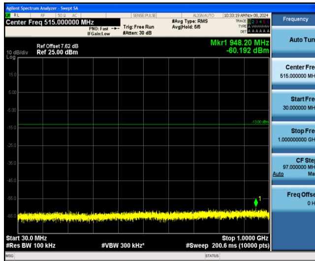
Band25-3MHz-16QAM-26055-1-0-Low-30-1000--60.19-PASS
