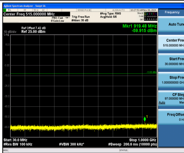
Band25-1.4MHz-QPSK-26683-1-0-High-30-1000--59.92-PASS
