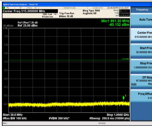
Band4-15MHz-16QAM-20175-1-0-Low-30-1000--60.13-PASS
