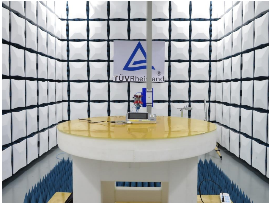
Photograph 1: Set-up for Radiated Spurious Emission, Above 1GHz
