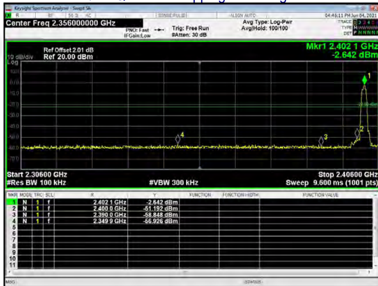
\pi/4 -DQPSK No-hopping Band edge-left side
