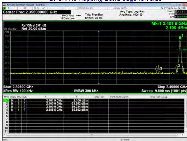
GFSK No-hopping Band edge-left side
