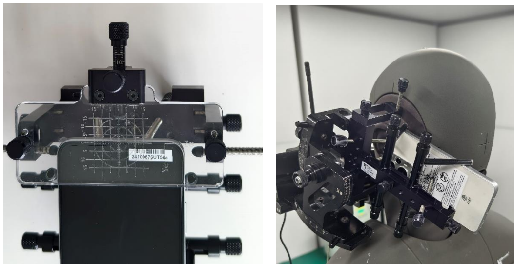
Pic 3: Handset Positioner (HHP III) with mounted EUT mobile phone
