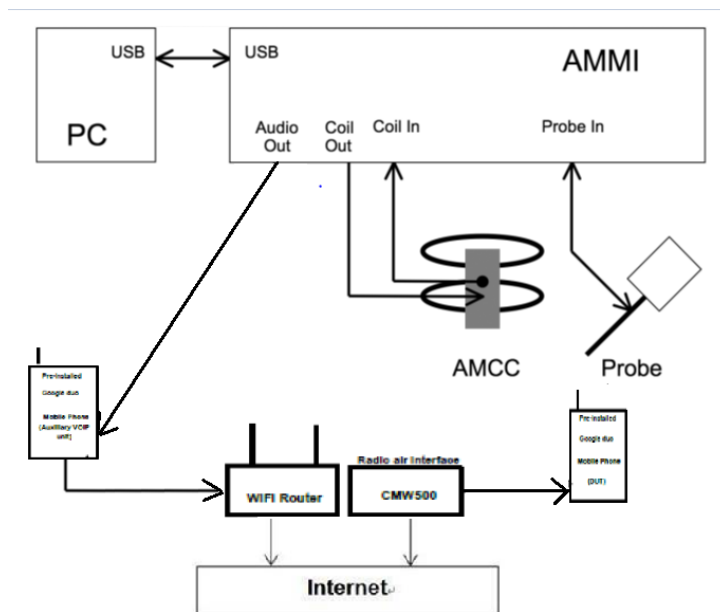
Fig. 2. T-coil signal measurement test setup
