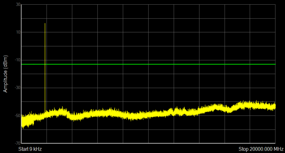
Band25 16QAM BW=1.4MHz Channel=26365 RB Size=1 Position=#0
