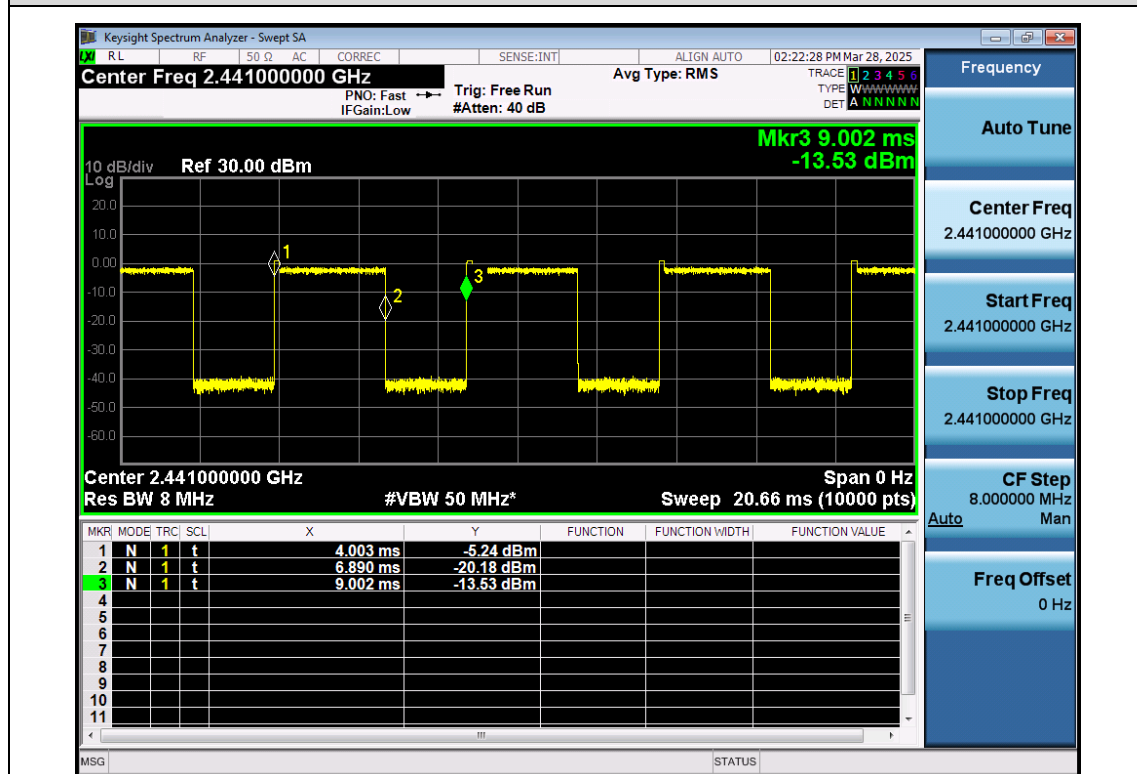
EDR-8DPSK-ANT1-2441
