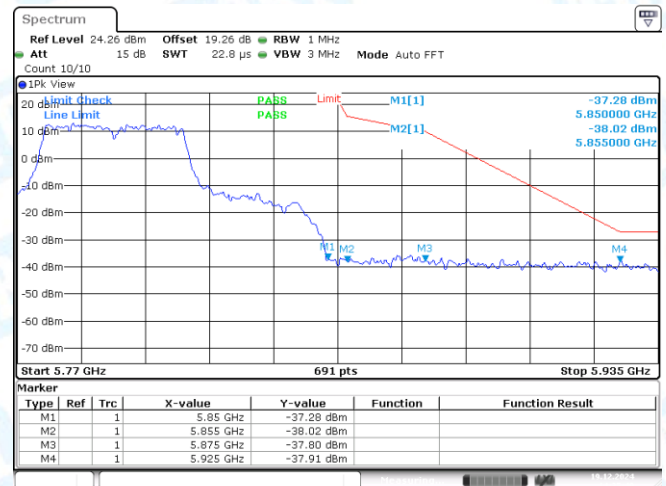
11AC40MIMO-Ant2-5755-PASS
