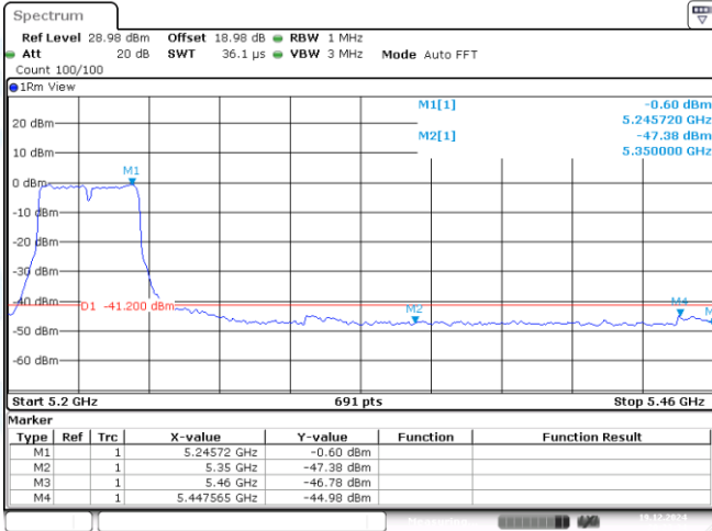
11N40MIMO-Ant1-5230-PASS
