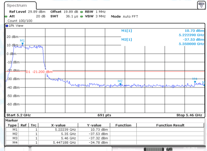
11AX40MIMO-Ant2-5190-PASS
