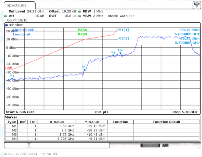
11N40MIMO-Ant2-5755-PASS
