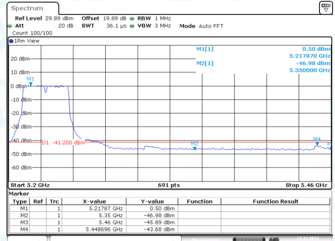
11AC40MIMO-Ant2-5230-PASS
