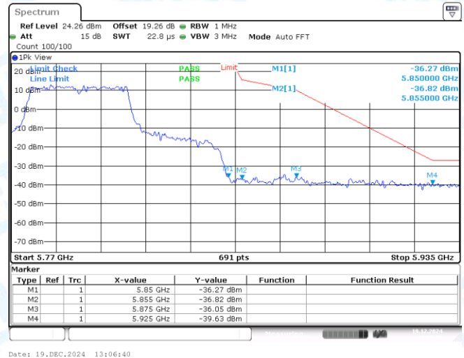
11N40MIMO-Ant2-5795-PASS
