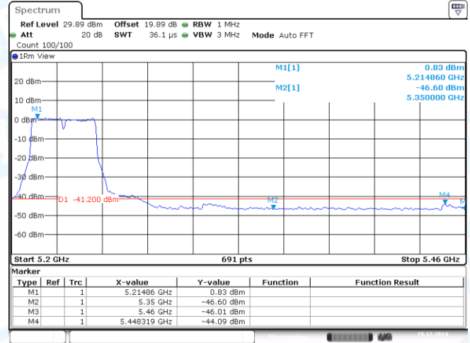
11N40MIMO-Ant2-5230-PASS
